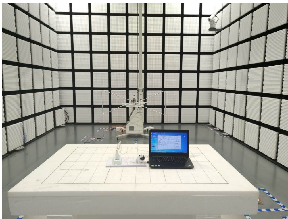
Radiated test setup for 30MHz~1GHz
