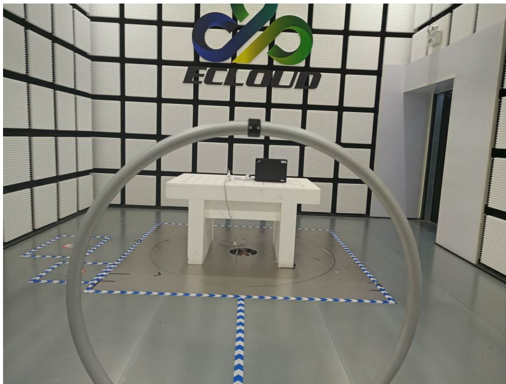
Radiated test setup for 9KHz~30MHz
