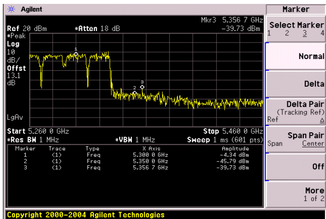
Antenna C
