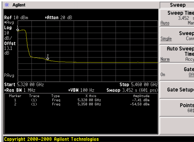
Antenna C
