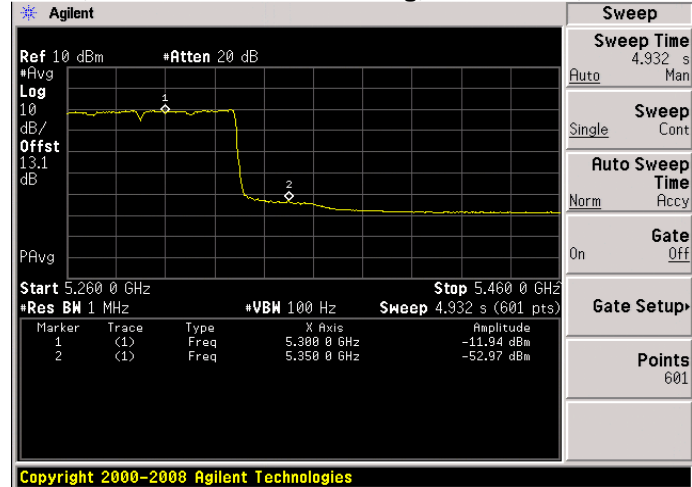
Antenna B
