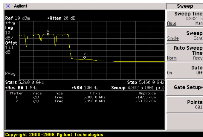
Antenna D
