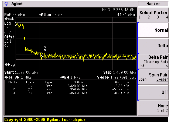
Antenna B
