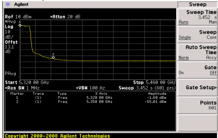
Antenna B
