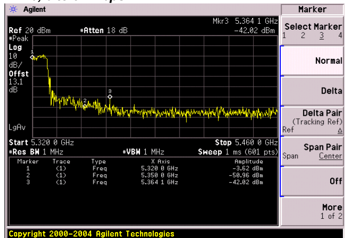
Antenna B
