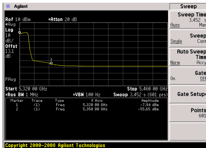
Antenna D
