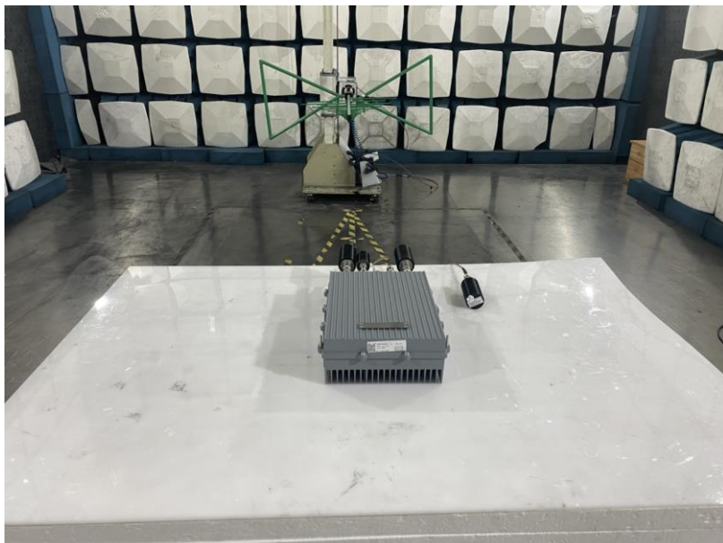
Radiated Spurious Emissions (30MHz-1GHz)
