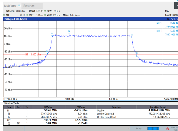
Band13-5MHz-QPSK-23230-25RB#0
