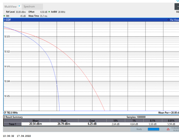
Band13-10MHz-16QAM-23230-50RB#0
