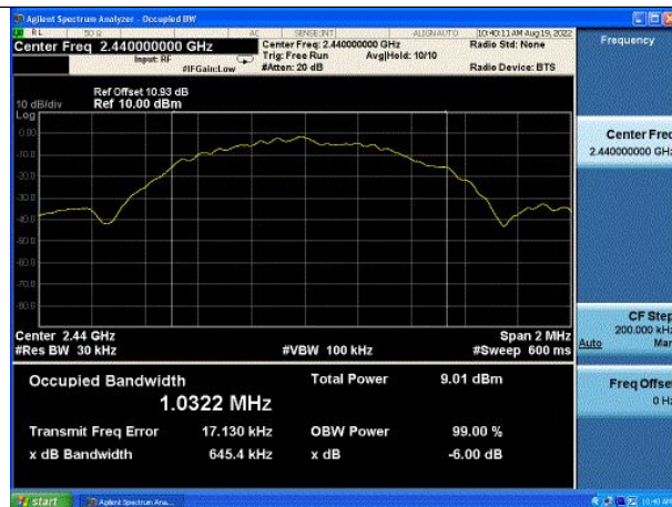
Test Mode:GFSK (LE 1Mbps) 2440 MHz
