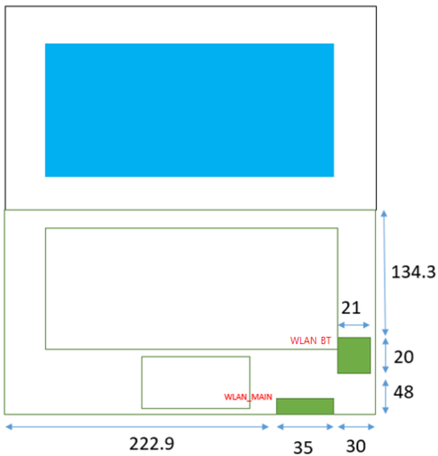
Picture 4 Antenna Locations
