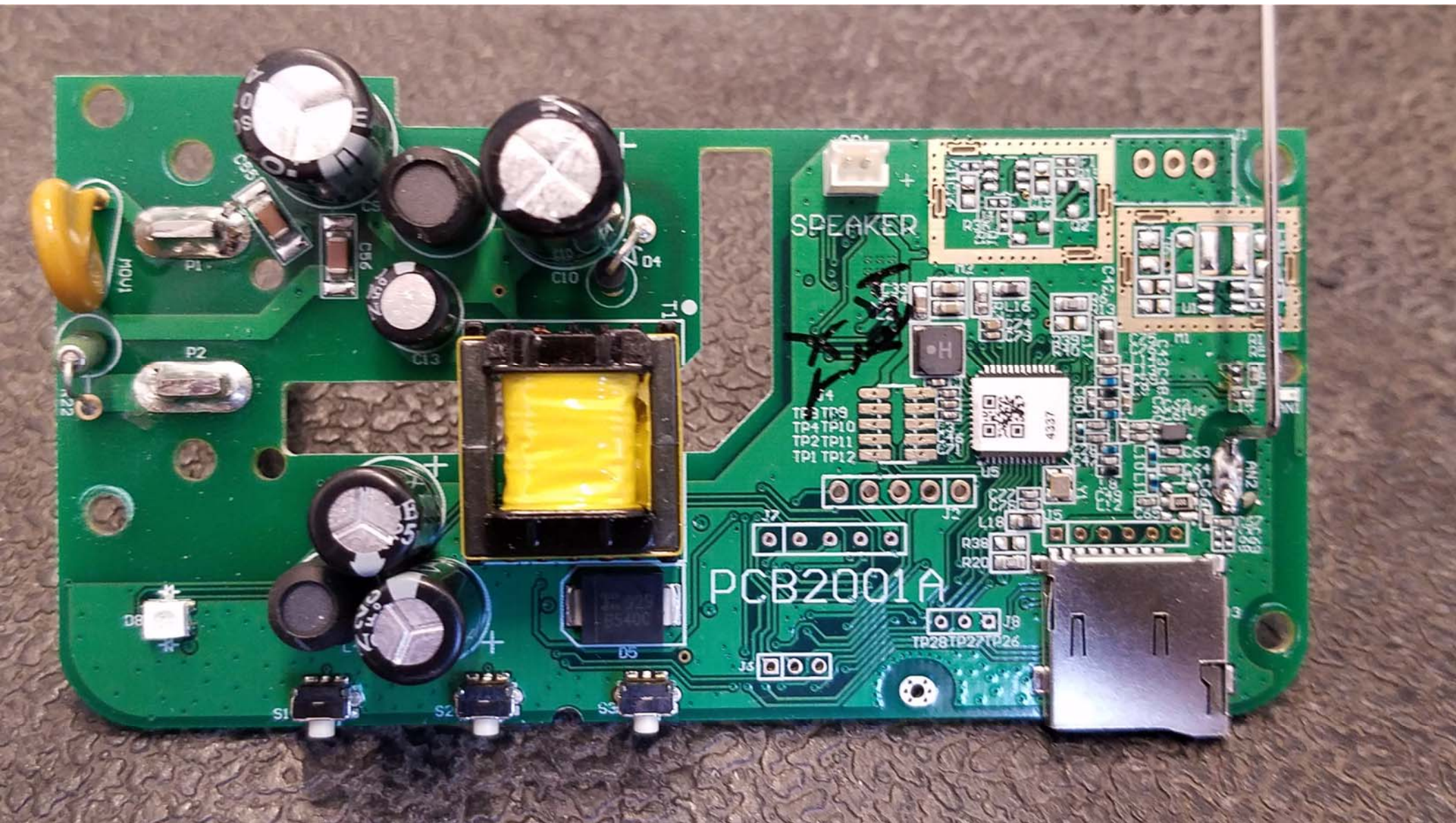
Top View of the PCB - View #1
