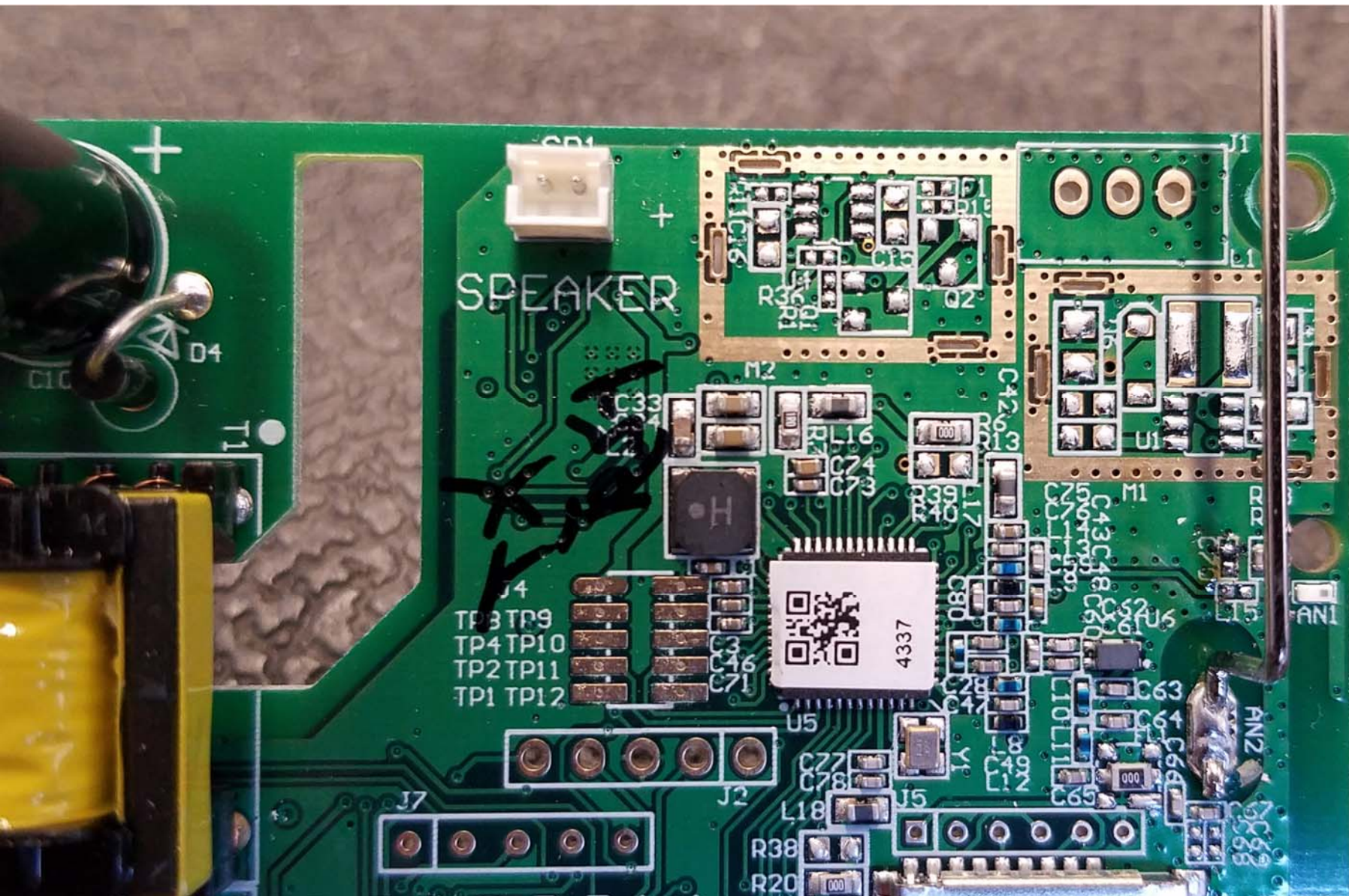
Top View of the PCB - Closeup - View #2
