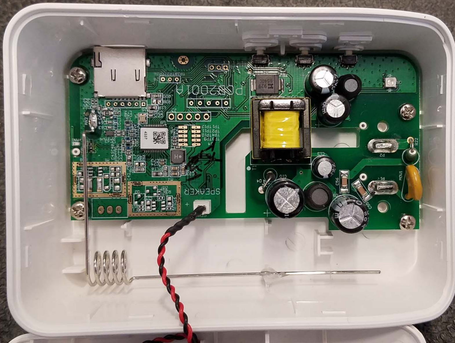
Inside View #6 of the EUT
