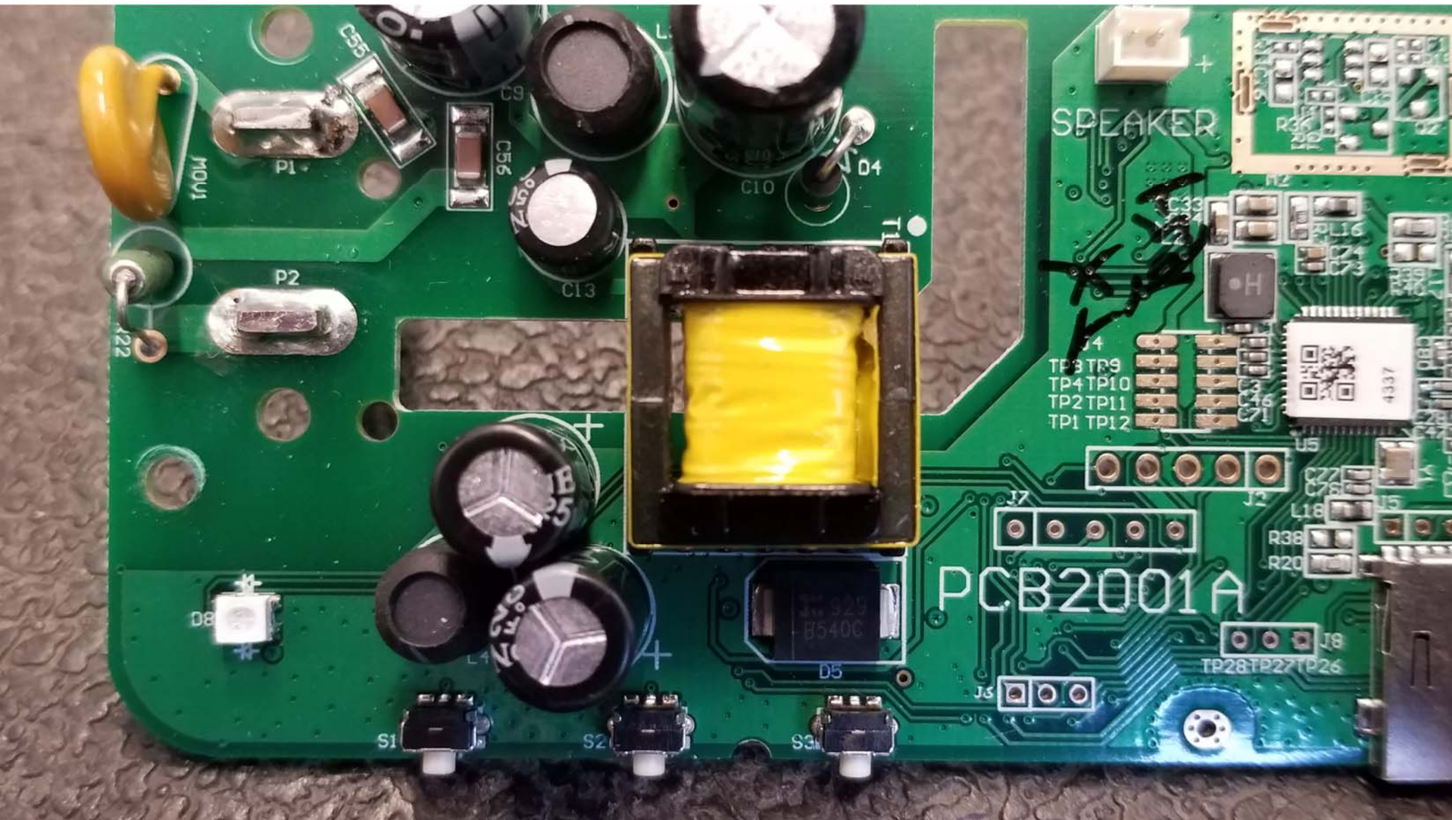
Top View of the PCB - View #3
