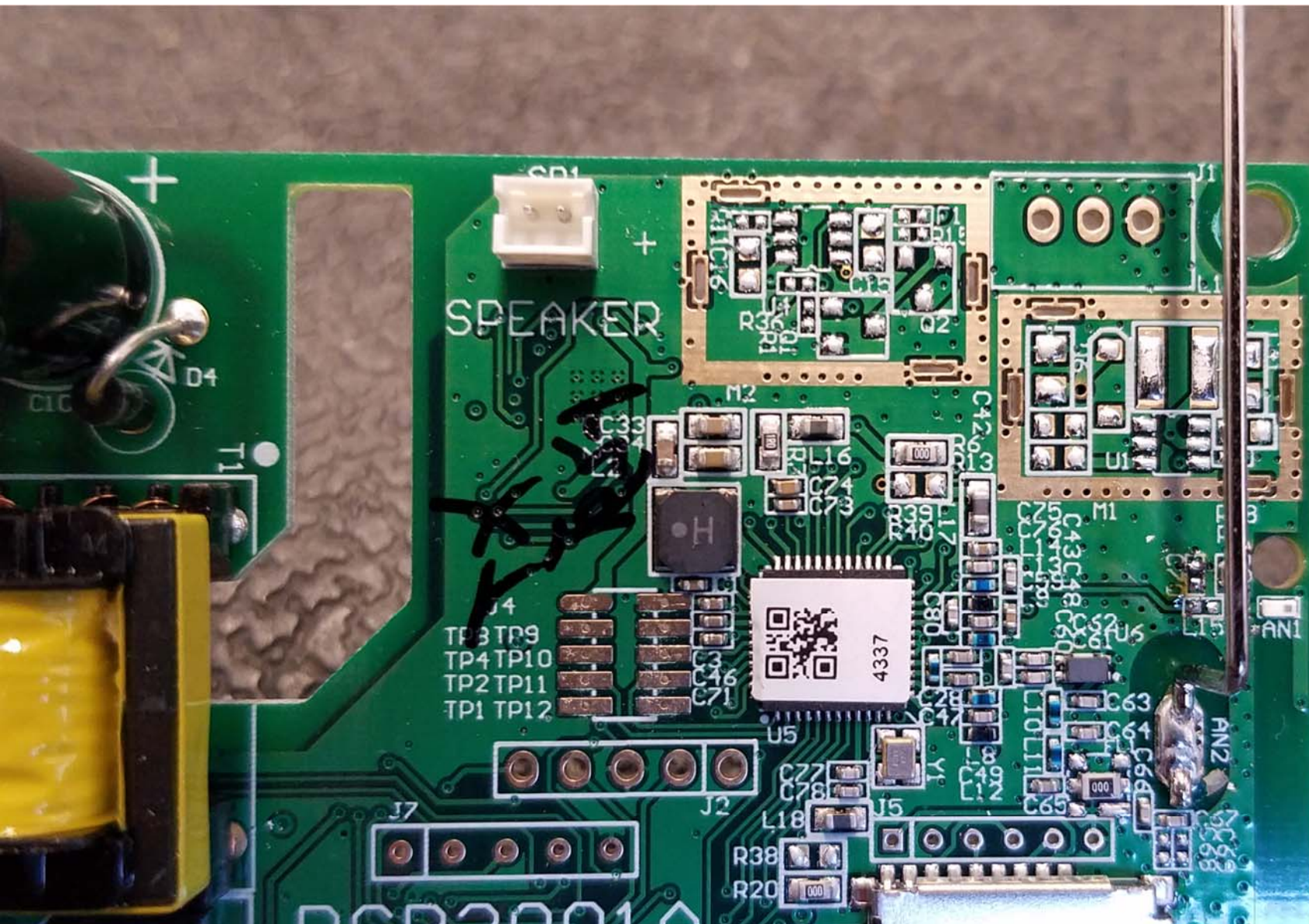
Top View of the PCB - Closeup - View #1
