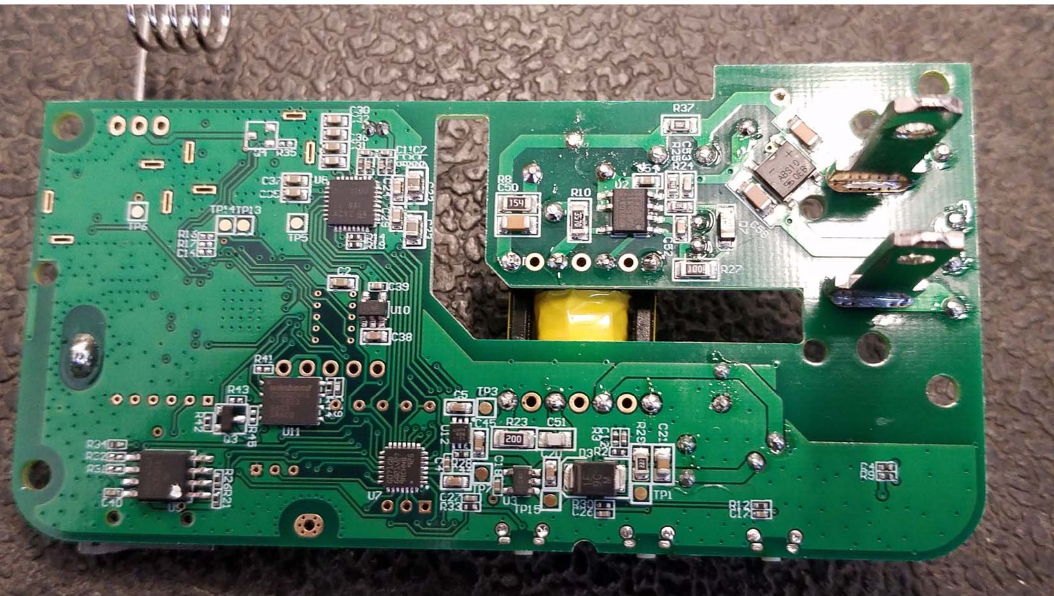
Bottom View of the PCB - View #4
