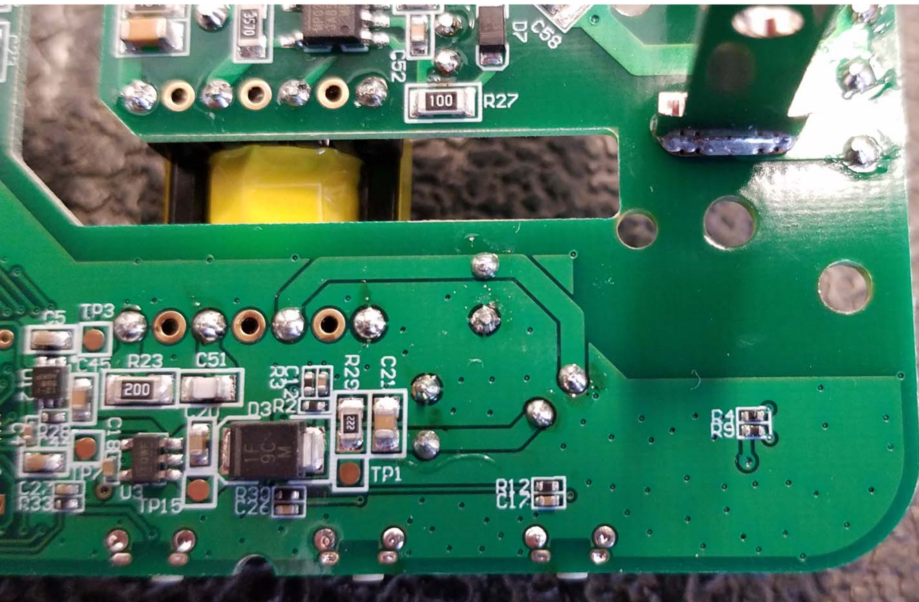
Bottom View of the PCB - Closeup #8
