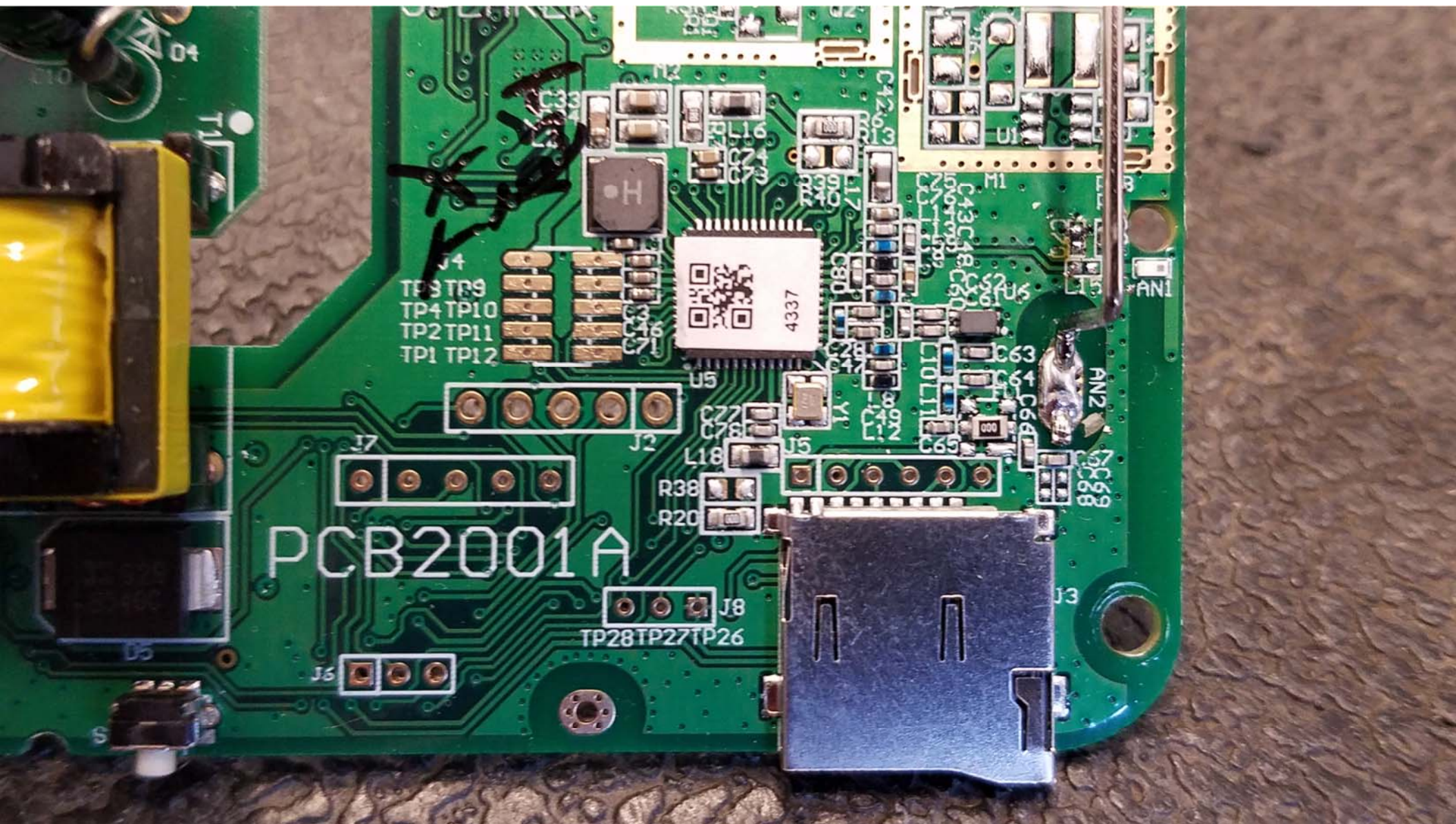
Top View of the PCB - Closeup - View #3
