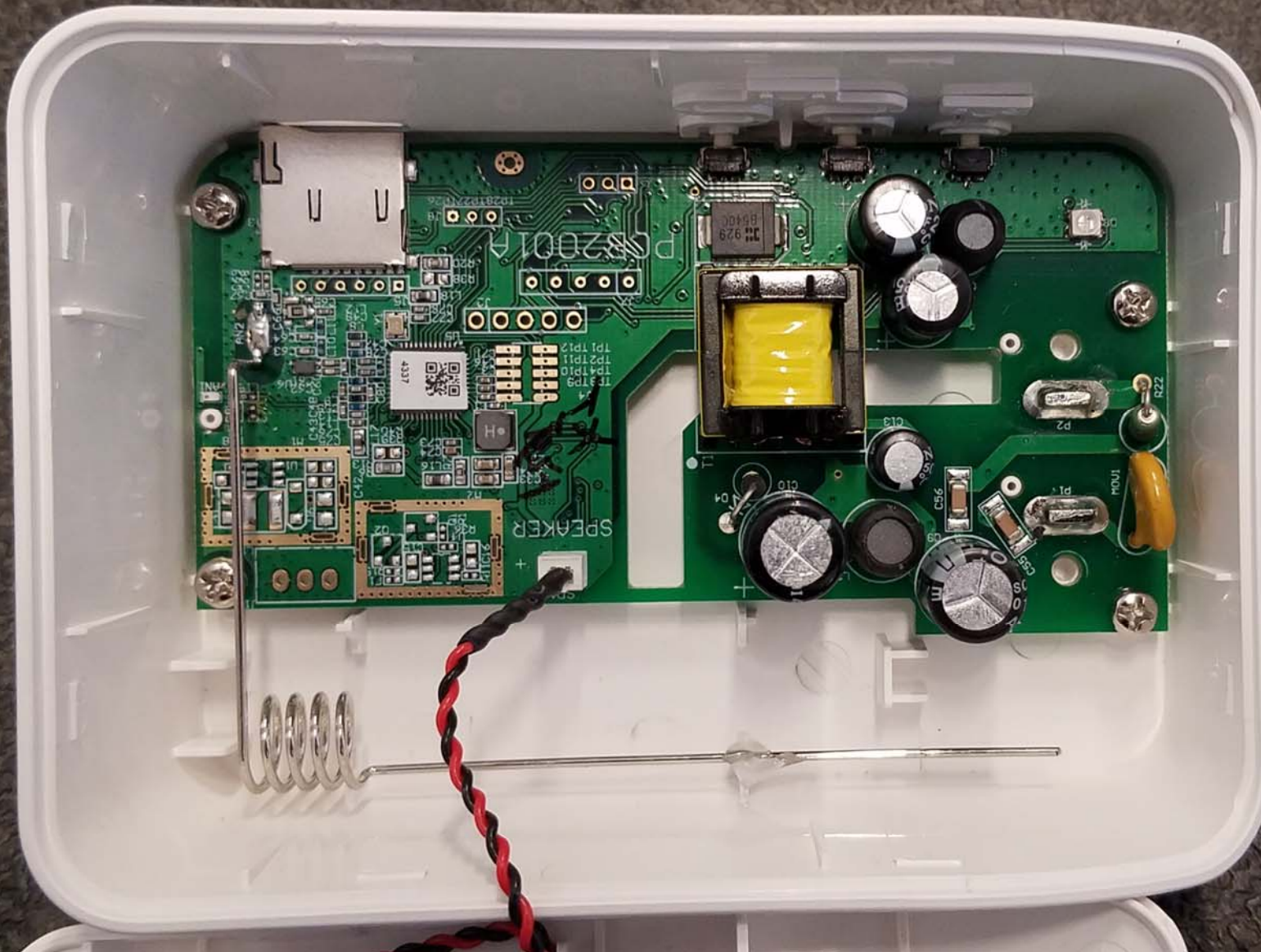
Inside View #5 of the EUT
