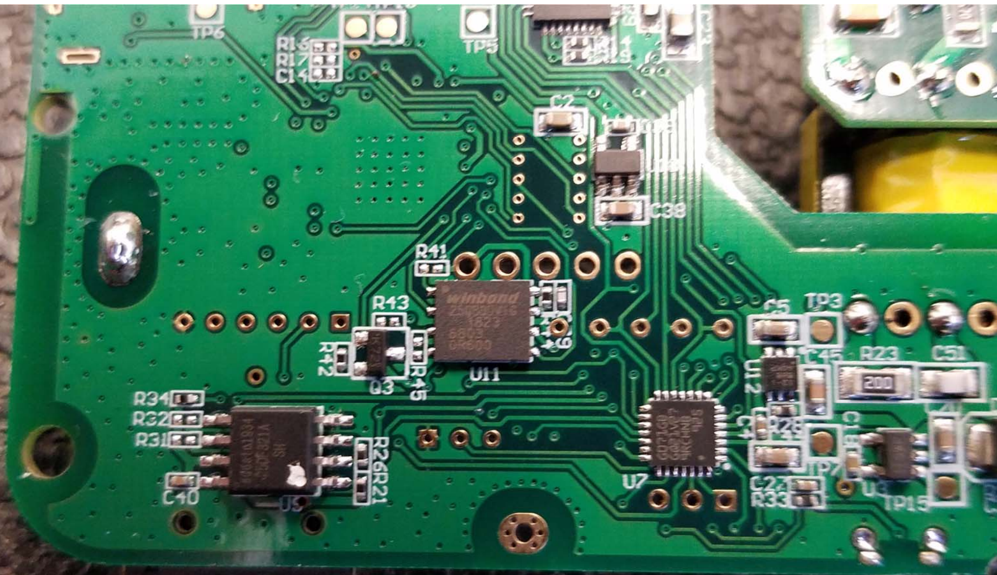
Bottom View of the PCB - Closeup #1
