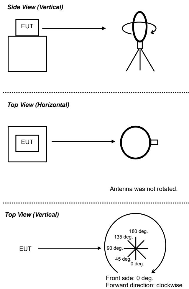
Figure 1: Direction of the Loop Antenna
