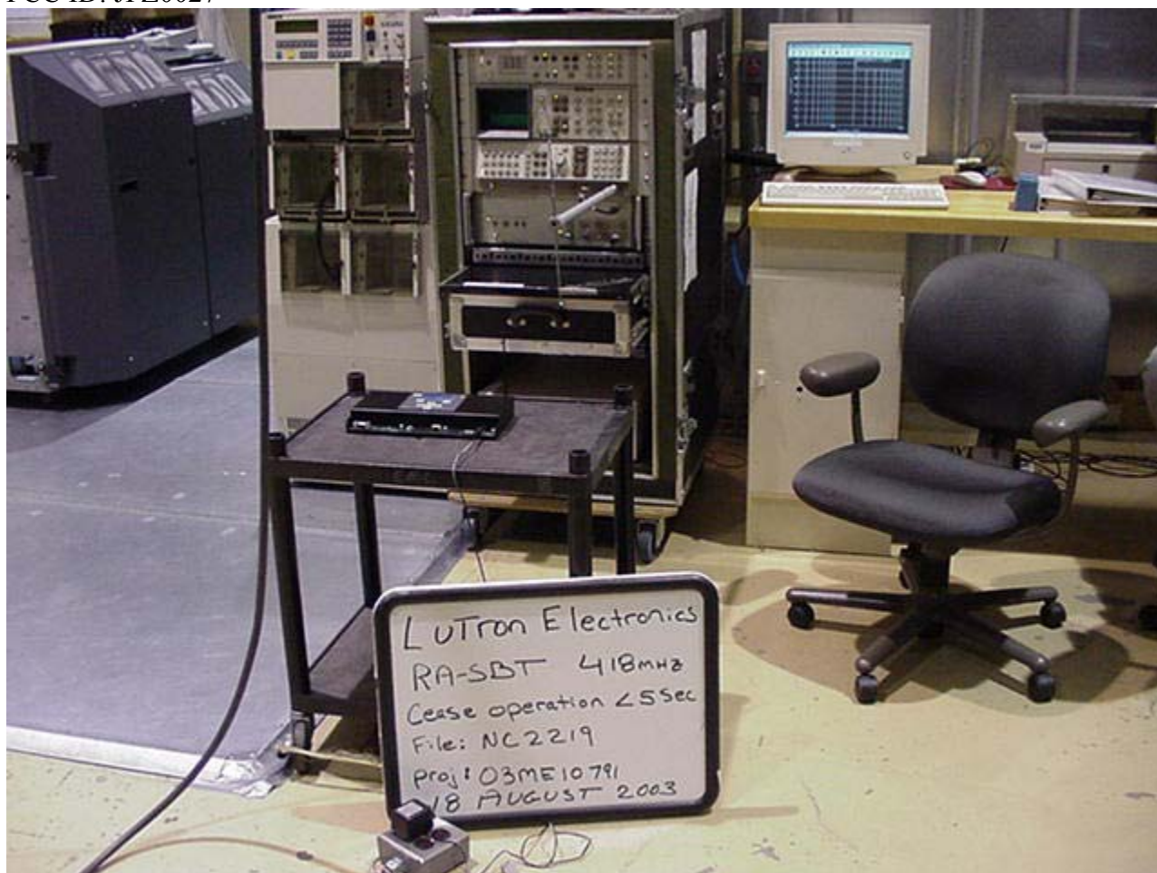
Cease Operation in Less Than 5 seconds Test Set-Up Note: The test photo depicted states RA-SBT 418 MHz. This is actually the RB-SBT, which operates at 433.9 MHz
