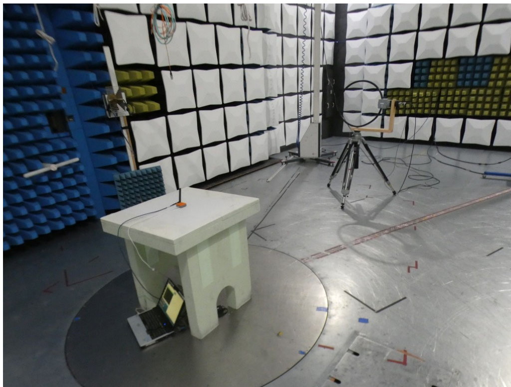
Photo 3: Test photos for radiated measurements below 30 MHz
