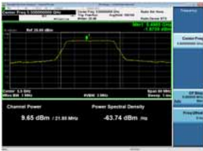
Antenna C
