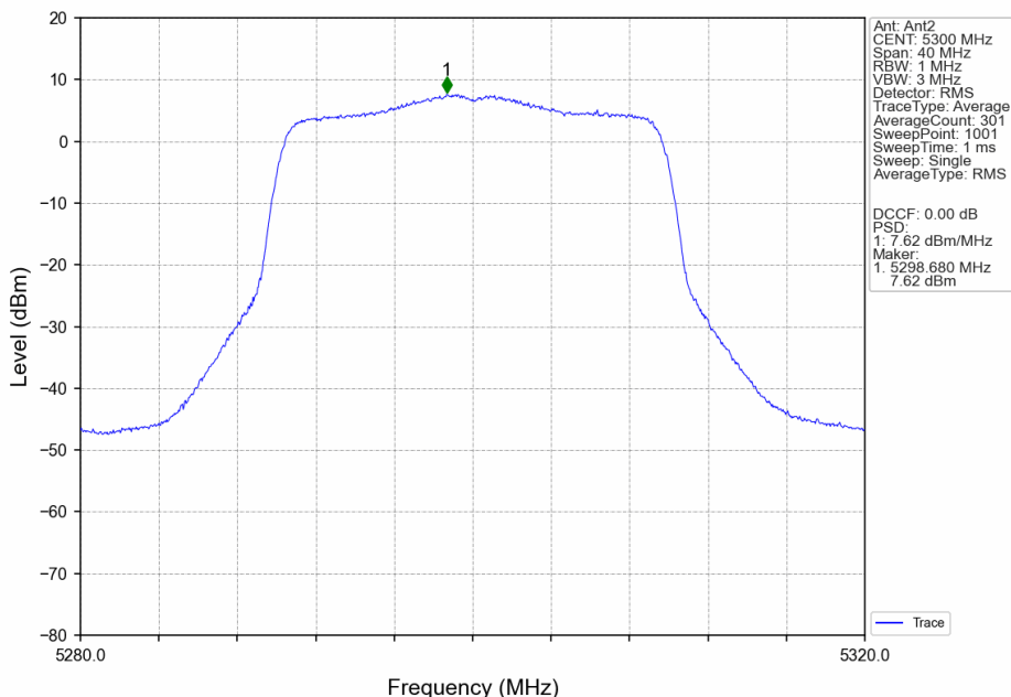
802.11ax(HEW20)_MCH_5300MHz_RU242_Left_MIMO_NTNV
