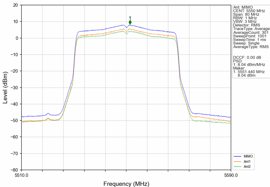
802.11ax(HEW40)_MCH_5550MHz_RU484_Left_MIMO_NTNV
