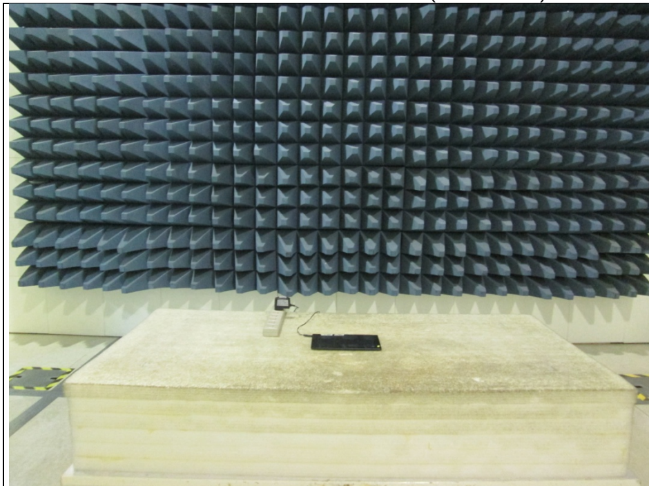
Radiated Emissions below 1 GHz Test (Test Mode A)
