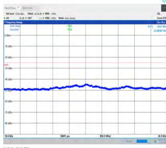
1-N41-PC2-30-100-M-1-DFT-QPSK-Edge_1RB_Left- 1@0-18000-26500-Ant1-22248.87--43.61--25-PASS
