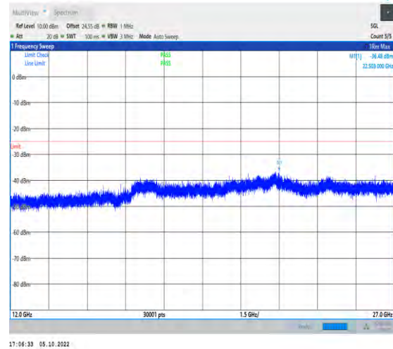
1-N41-PC2-30-100-H-1-DFT-QPSK-Inner_1RB_Left- 1@1-12000-27000-Ant1-22503.00--36.48--25-PASS
