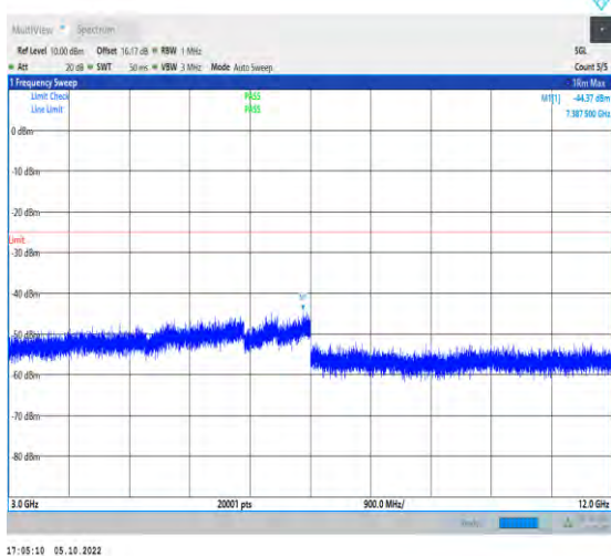
1-N41-PC2-30-100-M-1-DFT-QPSK-Inner_1RB_Left -1@1-3000-12000-Ant1-7387.50--44.37--25-PASS
