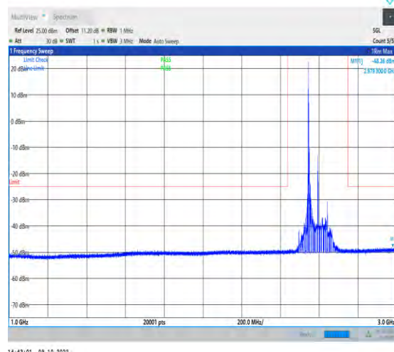
1-N41-PC2-30-100-M-1-DFT-QPSK-Edge_1RB_Left- 1@0-1000-3000-Ant1-2979.30--48.26--25-PASS
