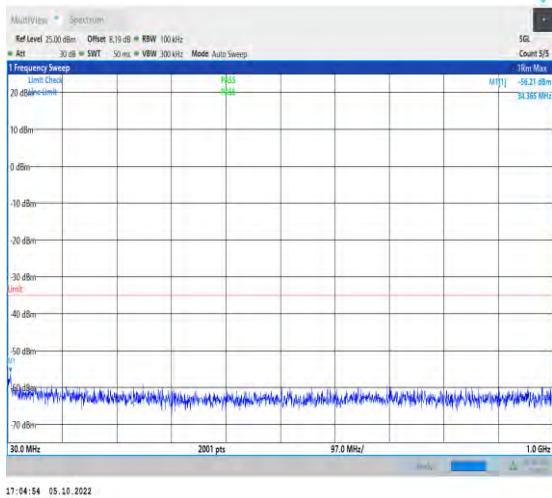
1-N41-PC2-30-100-M-1-DFT-QPSK-Inner_1RB_Left -1@1-30-1000-Ant1-34.37--56.21--35-PASS
