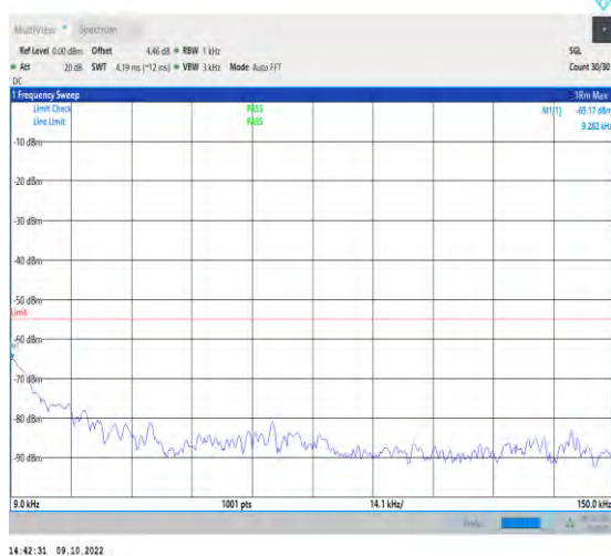
1-N41-PC2-30-100-M-1-DFT-QPSK-Edge_1RB_Left -1@0-0.009-0.15-Ant1-0.01--65.17--55-PASS
