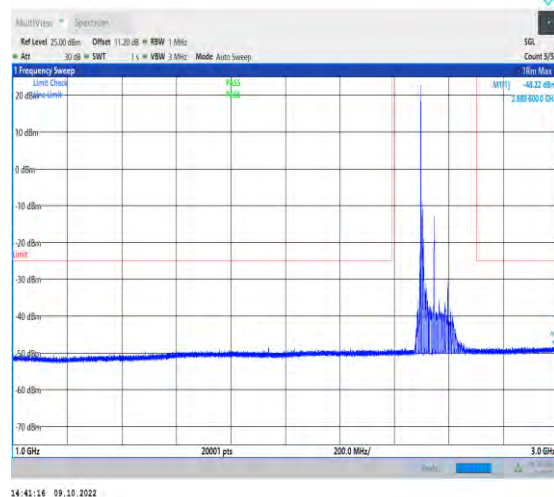
1-N41-PC2-30-100-L-1-DFT-QPSK-Edge_1RB_Left- 1@0-1000-3000-Ant1-2978.40--48.22--25-PASS
