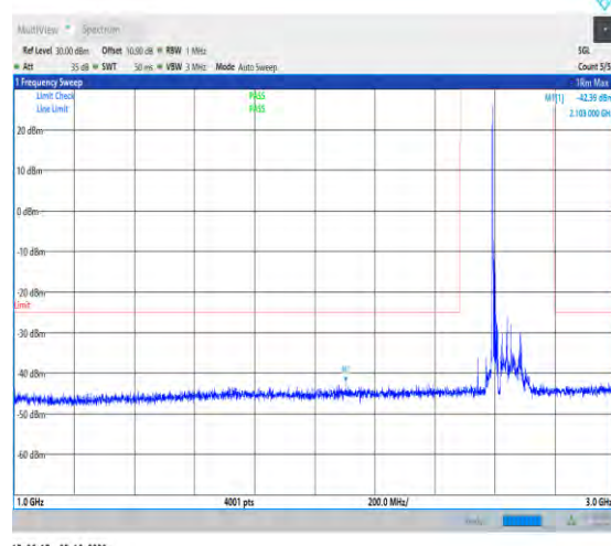
1-N41-PC2-30-100-H-1-DFT-QPSK-Inner_1RB_Left- 1@1-1000-3000-Ant1-2103.00--42.39--25-PASS
