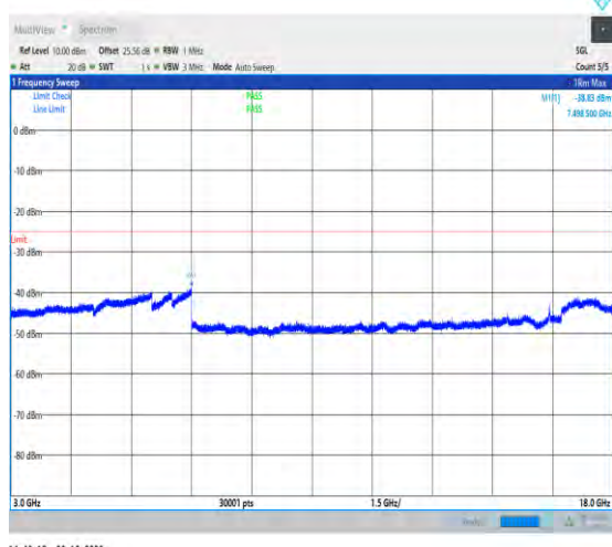
1-N41-PC2-30-100-M-1-DFT-QPSK-Edge_1RB_Left -1@0-3000-18000-Ant1-7498.50--38.83--25-PASS
