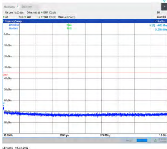
1-N41-PC2-30-100-L-1-DFT-QPSK-Edge_1RB_Left -1@0-30-1000-Ant1-33.49--66.01--35-PASS
