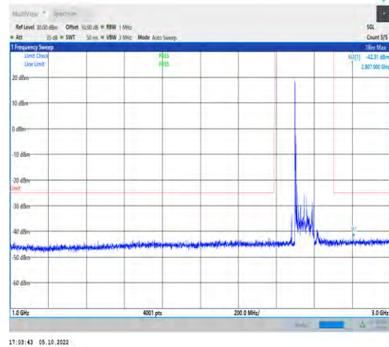
1-N41-PC2-30-100-M-1-DFT-QPSK-Inner_1RB_Left- 1@1-1000-3000-Ant1-2842.50--42.51--25-PASS
