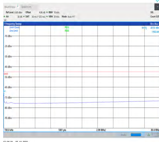
1-N41-PC2-30-100-H-1-DFT-QPSK-Inner_1RB_Left- 1@1-0.15-30-Ant1-0.18--67.51--45-PASS
