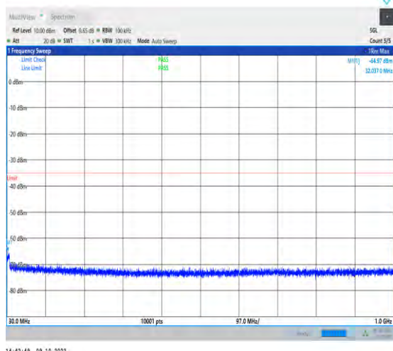
1-N41-PC2-30-100-M-1-DFT-QPSK-Edge_1RB_Left -1@0-30-1000-Ant1-32.04--64.97--35-PASS
