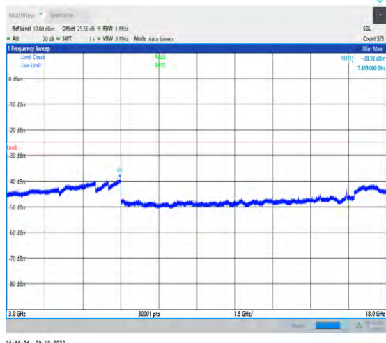
1-N41-PC2-30-100-H-1-DFT-QPSK-Edge_1RB_Left -1@0-3000-18000-Ant1-7453.00--38.92--25-PASS
