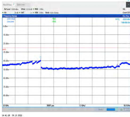
1-N41-PC2-30-100-L-1-DFT-QPSK-Edge_1RB_Left -1@0-3000-18000-Ant1-7489.00--38.99--25-PASS
