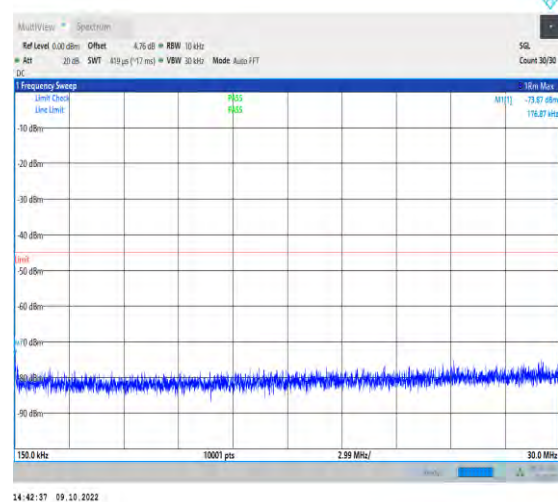
1-N41-PC2-30-100-M-1-DFT-QPSK-Edge_1RB_Left- 1@0-0.15-30-Ant1-0.18--73.87--45-PASS
