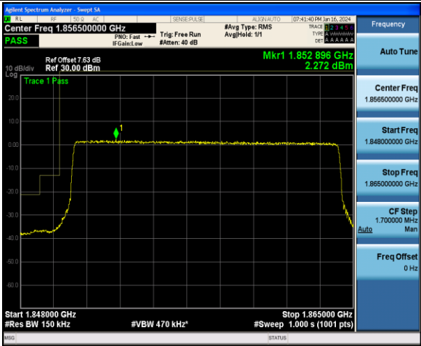
Band2_15MHz_QPSK_18675_75RB#0
