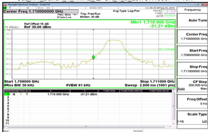
Cat_M1_Band4_1_4MHz_QPSK_1_0_LowCH19957-1710.7
