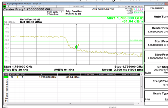
Cat_M1_Band4_1_4MHz_QPSK_6_0_HighCH20393-1754.3
