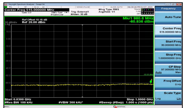
Band40_5MHz_16QAM_38775_1RB#0_30~1000_30~1000
