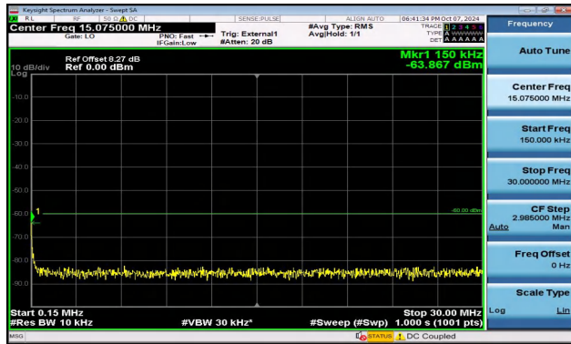
Band40_10MHz_16QAM_38750_1RB#0_0.15~30_0.15~30
