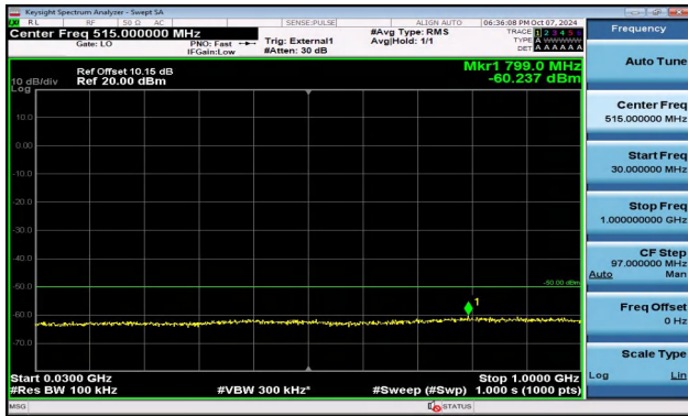
Band40_5MHz_QPSK_38750_1RB#0_30~1000_30~1000
