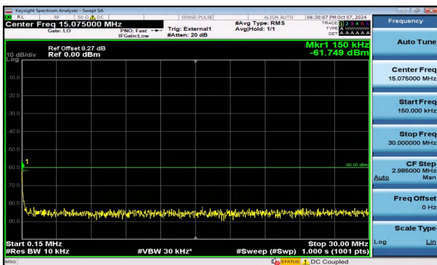
Band40_5MHz_16QAM_38775_1RB#0_0.15~30_0.15~30
