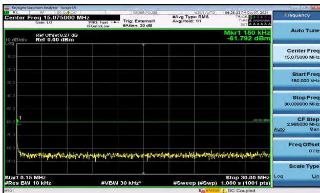
Band40_5MHz_16QAM_38750_1RB#0_0.15~30_0.15~30
