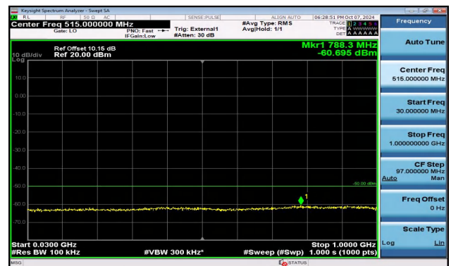
Band40_5MHz_16QAM_38750_1RB#0_30~1000_30~1000
