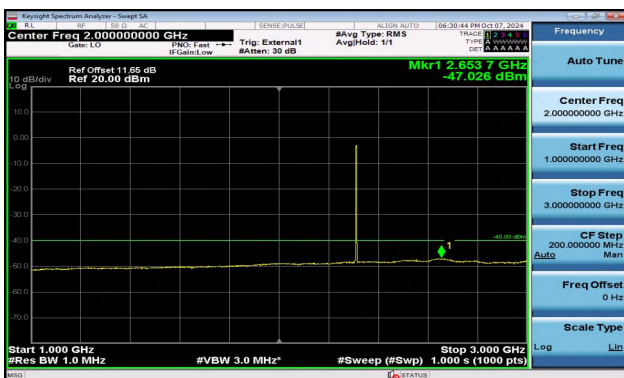
Band40_5MHz_16QAM_38775_1RB#0_1000~3000_1000~3000
