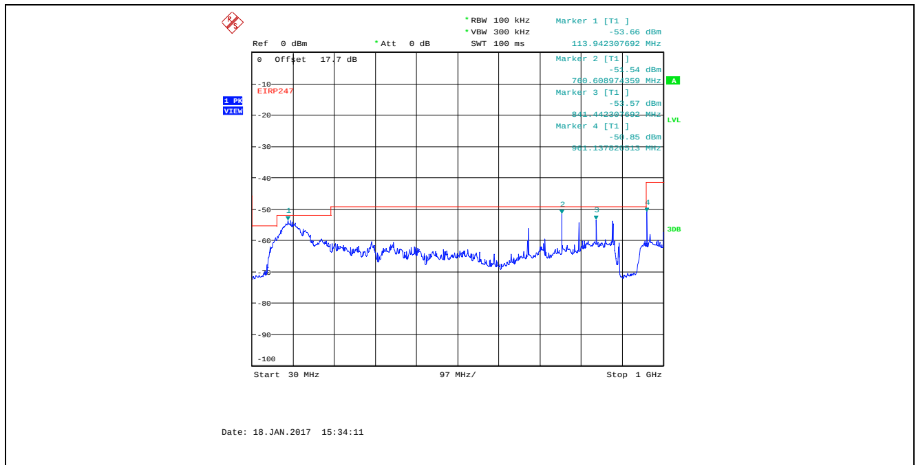
Plot 5.4.4.23. Conducted Spurious Emissions in Restricted Frequency Bands Bandwidth: 8 MHz, TX Gain Setting 23, Data Rate 4, 915 MHz, 30 MHz - 1 GHz, Peak Detector
