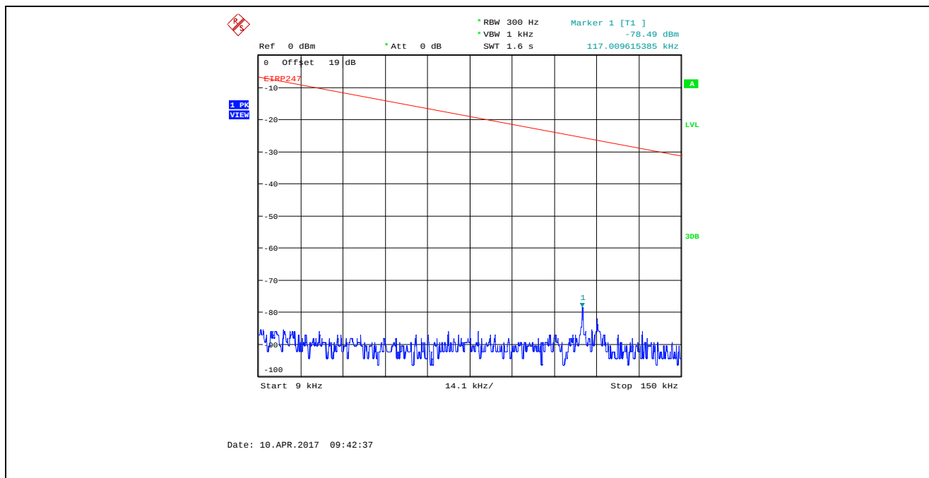
Plot 5.4.4.25. Conducted Spurious Emissions in Restricted Frequency Bands Bandwidth: 8 MHz, TX Gain Setting 23, Data Rate 4, 923 MHz, 9 kHz - 150 kHz, Peak Detector
