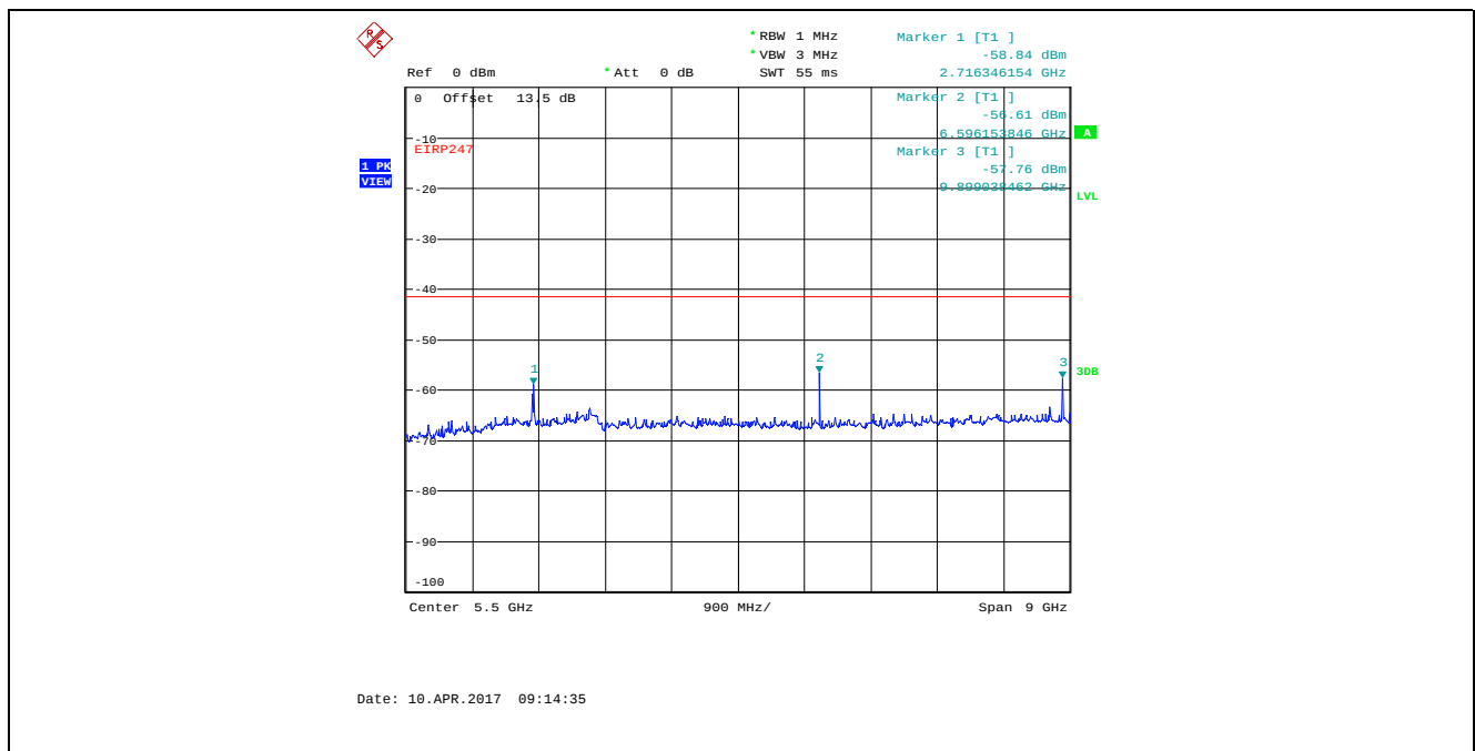
Plot 5.4.4.3.20. Conducted Spurious Emissions in Restricted Frequency Bands Bandwidth: 8 MHz, TX Gain Setting 36, Data Rate 4, 907 MHz, 1 GHz - 10 GHz, Peak Detector
