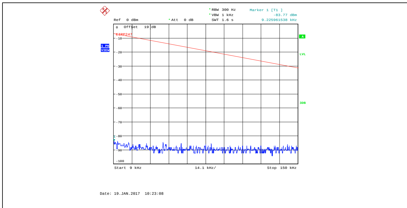
Plot 5.4.4.4.6. Conducted Spurious Emissions in Restricted Frequency Bands Bandwidth: 8 MHz, TX Gain Setting 23, Data Rate 1, 915 MHz, 9 kHz - 150 kHz, Peak Detector
