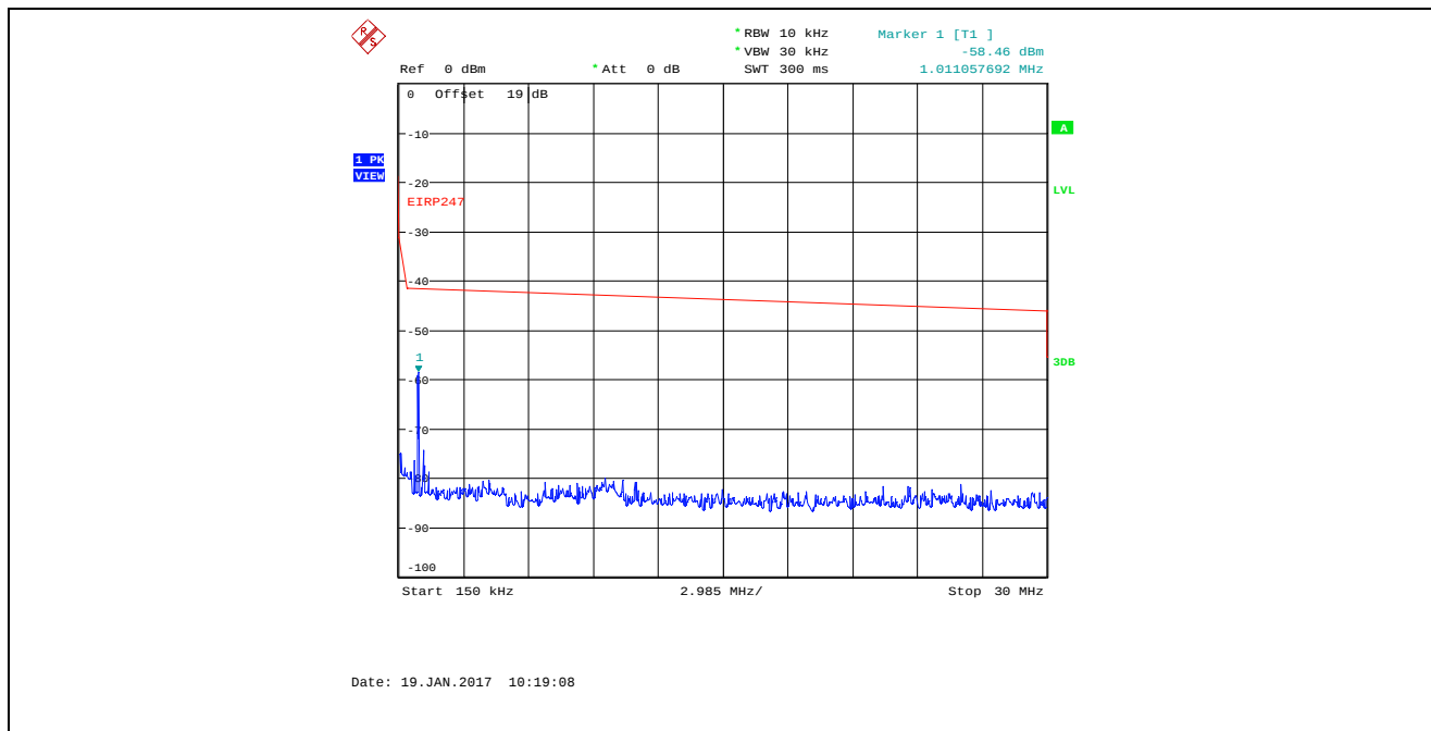
Plot 5.4.4.4.7. Conducted Spurious Emissions in Restricted Frequency Bands Bandwidth: 8 MHz, TX Gain Setting 23, Data Rate 1, 915 MHz, 150 kHz - 30 MHz, Peak Detector
