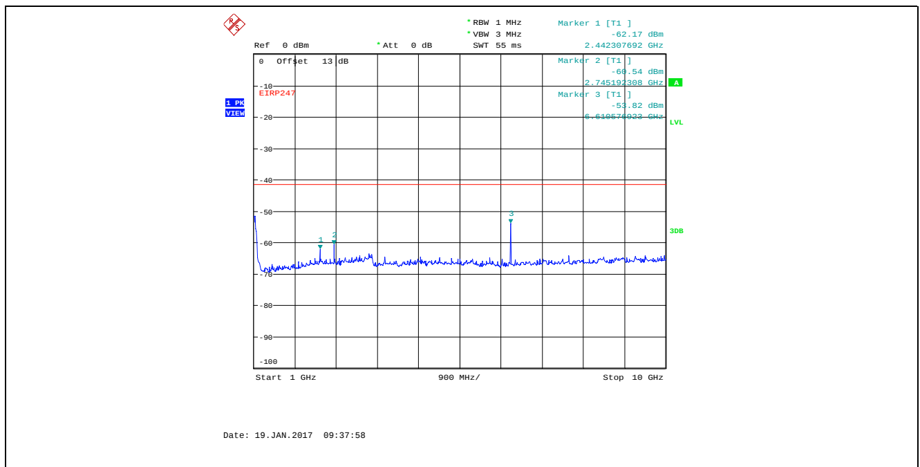
Plot 5.4.4.4.10. Conducted Spurious Emissions in Restricted Frequency Bands Bandwidth: 8 MHz, TX Gain Setting 23, Data Rate 1, 915 MHz, 1 GHz - 10 GHz, Peak Detector
