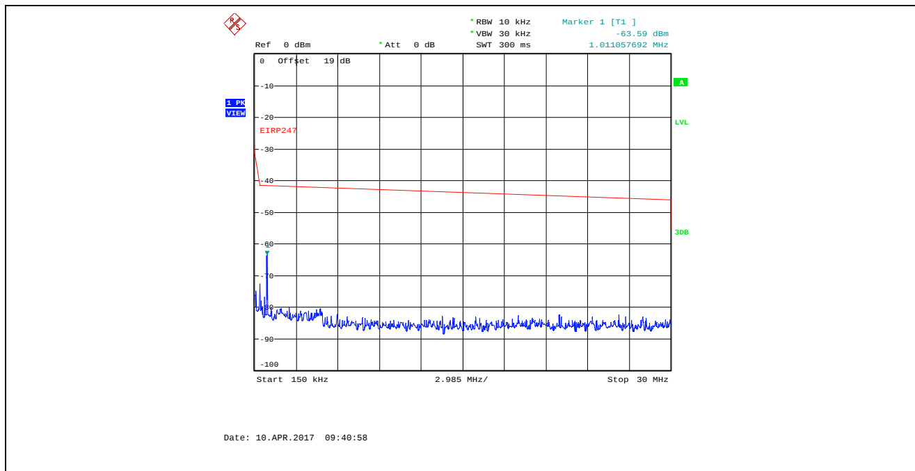
Plot 5.4.4.26. Conducted Spurious Emissions in Restricted Frequency Bands Bandwidth: 8 MHz, TX Gain Setting 23, Data Rate 4, 923 MHz, 150 kHz - 30 MHz, Peak Detector
