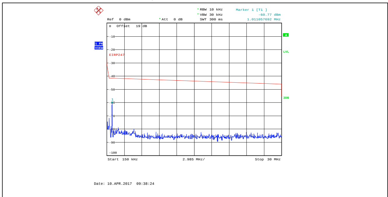
Plot 5.4.4.17. Conducted Spurious Emissions in Restricted Frequency Bands Bandwidth: 8 MHz, TX Gain Setting 23, Data Rate 4, 907 MHz, 150 kHz - 30 MHz, Peak Detector
