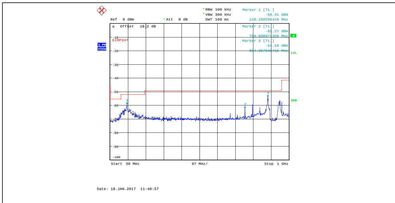
Plot 5.4.4.3.23. Conducted Spurious Emissions in Restricted Frequency Bands Bandwidth: 8 MHz, TX Gain Setting 36, Data Rate 4, 915 MHz, 30 MHz - 1 GHz, Peak Detector
