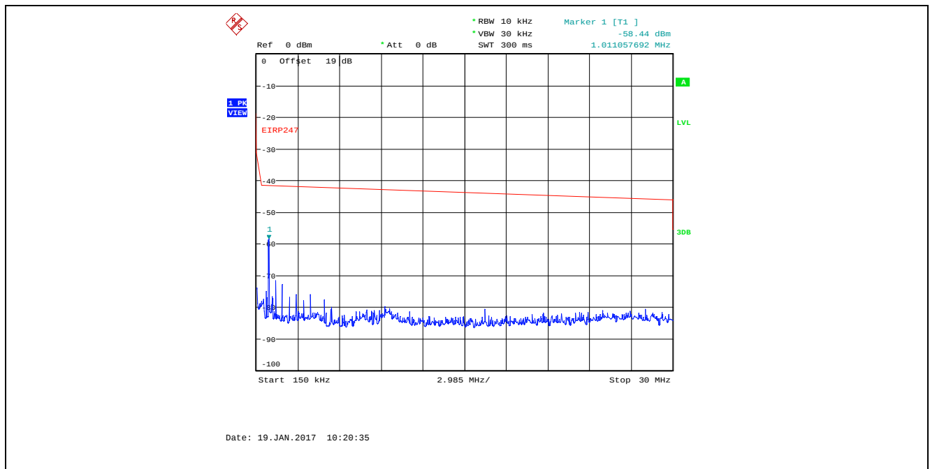
Plot 5.4.4.4.12. Conducted Spurious Emissions in Restricted Frequency Bands Bandwidth: 8 MHz, TX Gain Setting 23, Data Rate 1, 924 MHz, 150 kHz - 30 MHz, Peak Detector
