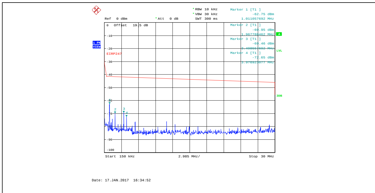
Plot 5.4.4.3.12. Conducted Spurious Emissions in Restricted Frequency Bands Bandwidth: 8 MHz, TX Gain Setting 40, Data Rate 1, 924 MHz, 150 kHz - 30 MHz, Peak Detector
