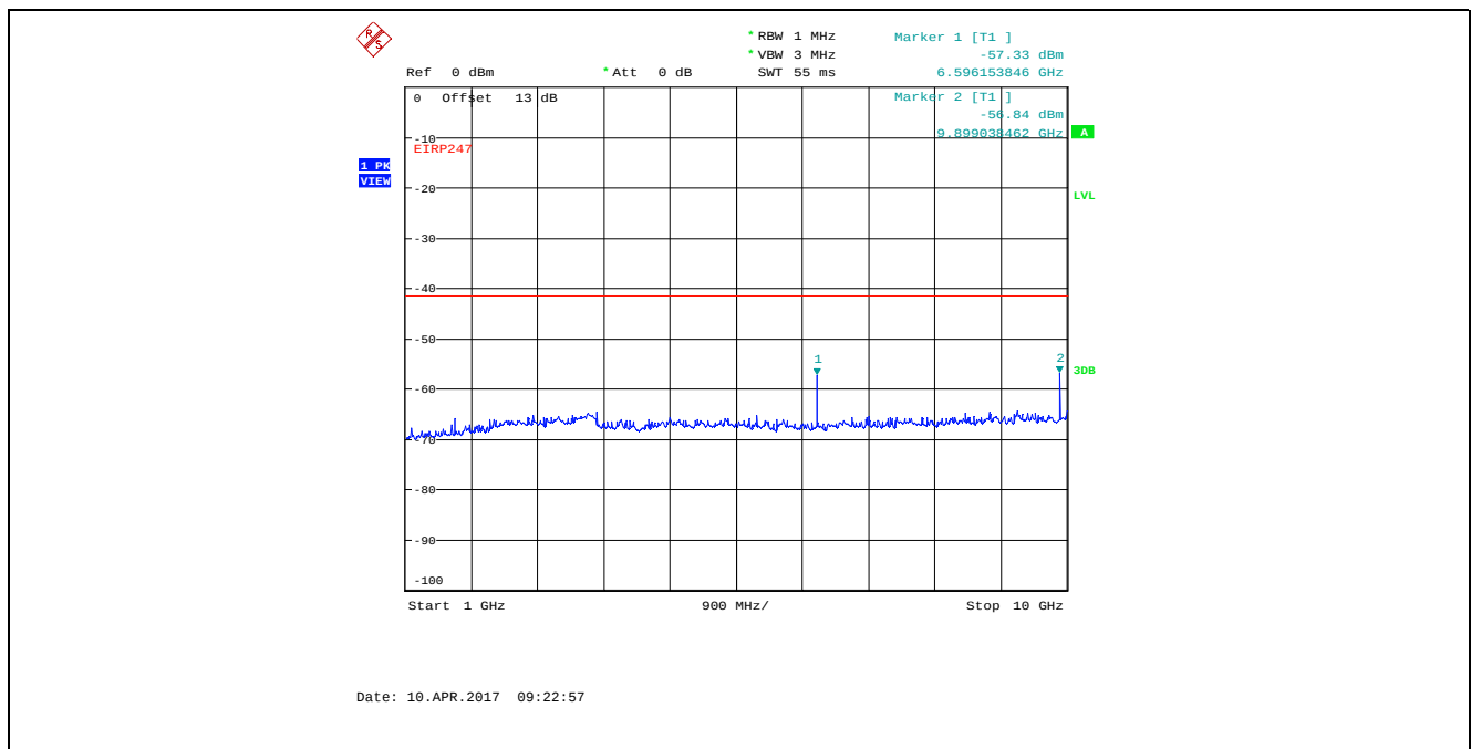
Plot 5.4.4.4.20. Conducted Spurious Emissions in Restricted Frequency Bands Bandwidth: 8 MHz, TX Gain Setting 23, Data Rate 4, 907 MHz, 1 GHz - 10 GHz, Peak Detector
