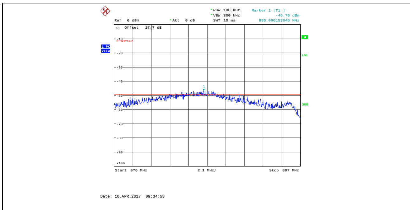
Plot 5.4.4.19. Conducted Spurious Emissions in Restricted Frequency Bands Bandwidth: 8 MHz, TX Gain Setting 23, Data Rate 4, 907 MHz, Peak Detector Emission Band Below is Outside of Restricted Bands
