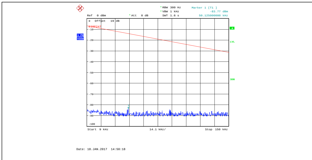
Plot 5.4.4.21. Conducted Spurious Emissions in Restricted Frequency Bands Bandwidth: 8 MHz, TX Gain Setting 23, Data Rate 4, 915 MHz, 9 kHz - 150 kHz, Peak Detector
