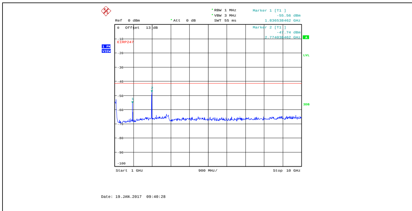
Plot 5.4.4.15. Conducted Spurious Emissions in Restricted Frequency Bands Bandwidth: 8 MHz, TX Gain Setting 23, Data Rate 1, 924 MHz, 1 GHz - 10 GHz, Peak Detector
