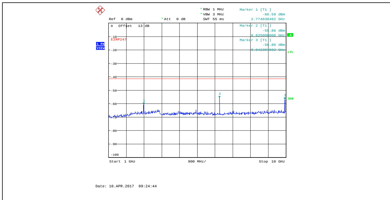
Plot 5.4.4.28. Conducted Spurious Emissions in Restricted Frequency Bands Bandwidth: 8 MHz, TX Gain Setting 23, Data Rate 4, 923 MHz, 1 GHz - 10 GHz, Peak Detector
