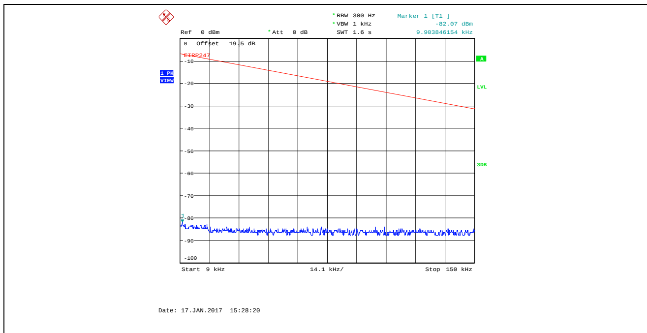
Plot 5.4.4.3.6. Conducted Spurious Emissions in Restricted Frequency Bands Bandwidth: 8 MHz, TX Gain Setting 40, Data Rate 1, 915 MHz, 9 kHz - 150 kHz, Peak Detector
