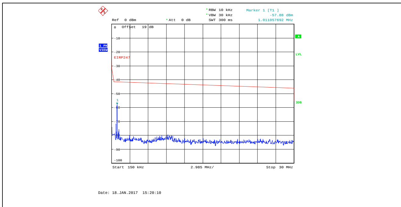
Plot 5.4.4.22. Conducted Spurious Emissions in Restricted Frequency Bands Bandwidth: 8 MHz, TX Gain Setting 23, Data Rate 4, 915 MHz, 150 kHz - 30 MHz, Peak Detector
