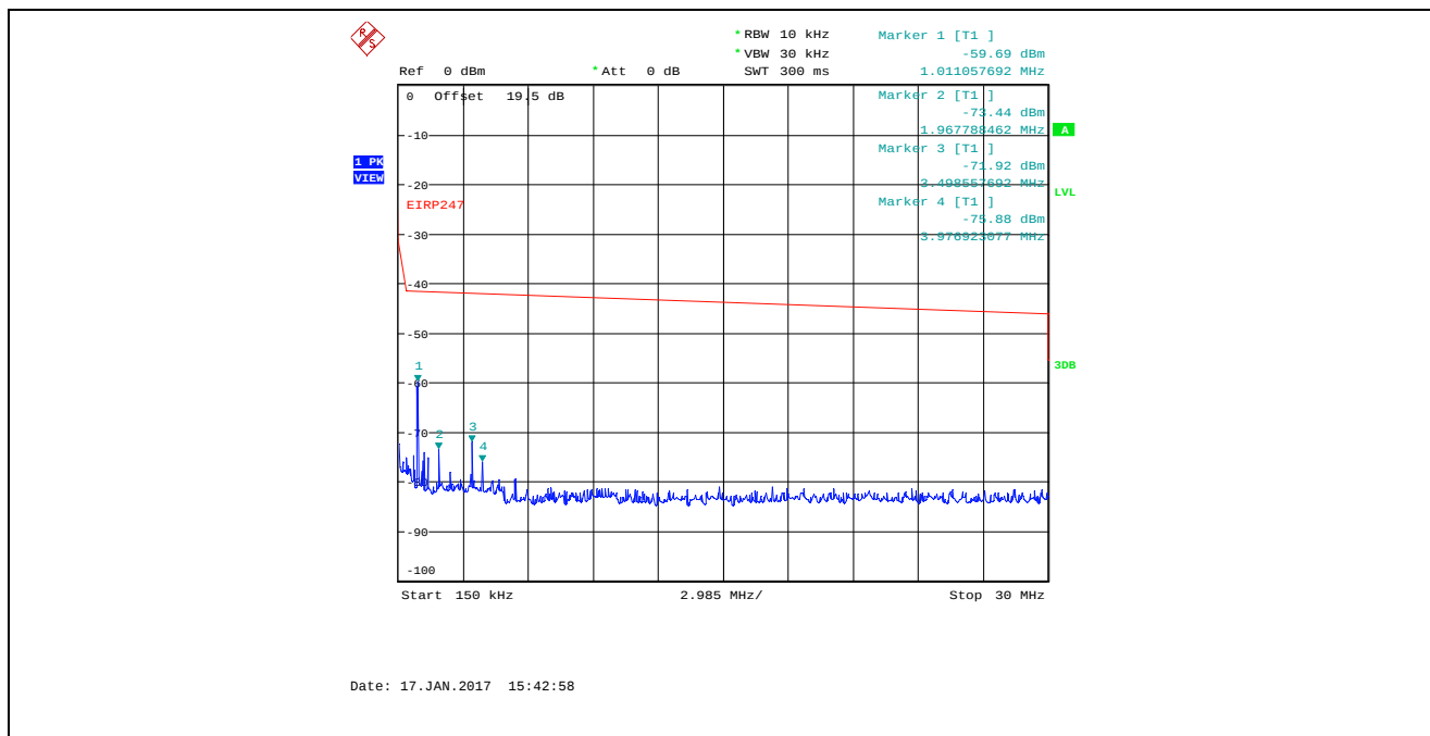
Plot 5.4.4.3.7. Conducted Spurious Emissions in Restricted Frequency Bands Bandwidth: 8 MHz, TX Gain Setting 40, Data Rate 1, 915 MHz, 150 kHz - 30 MHz, Peak Detector
