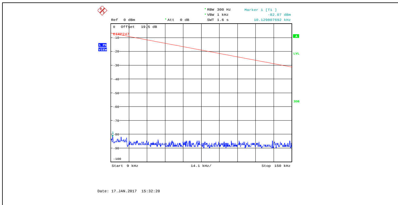
Plot 5.4.4.3.11. Conducted Spurious Emissions in Restricted Frequency Bands Bandwidth: 8 MHz, TX Gain Setting 40, Data Rate 1, 924 MHz, 9 kHz - 150 kHz, Peak Detector
