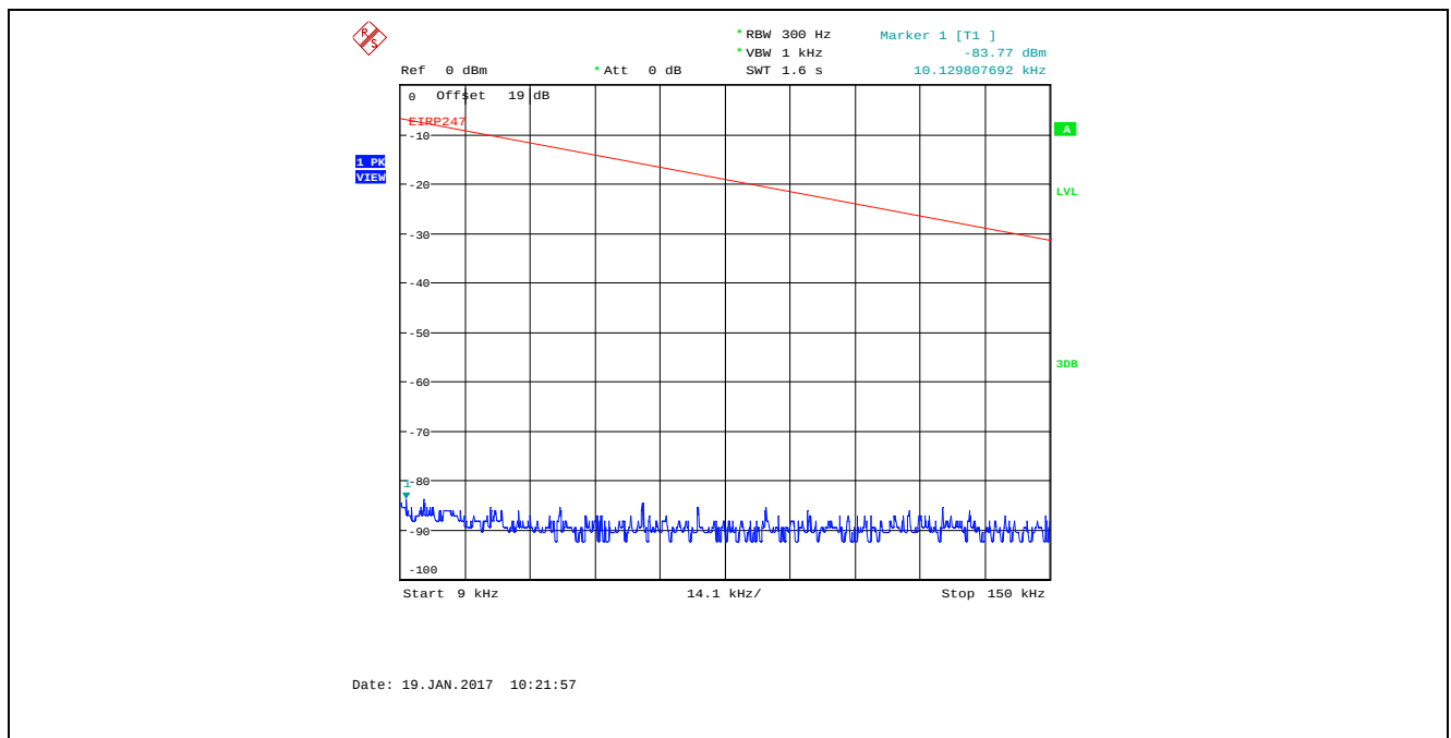
Plot 5.4.4.4.11. Conducted Spurious Emissions in Restricted Frequency Bands Bandwidth: 8 MHz, TX Gain Setting 23, Data Rate 1, 924 MHz, 9 kHz - 150 kHz, Peak Detector
