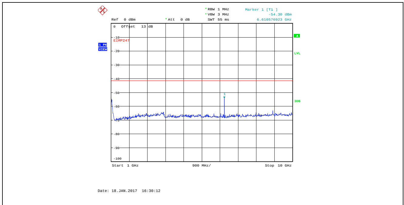
Plot 5.4.4.24. Conducted Spurious Emissions in Restricted Frequency Bands Bandwidth: 8 MHz, TX Gain Setting 23, Data Rate 4, 915 MHz, 1 GHz - 10 GHz, Peak Detector
