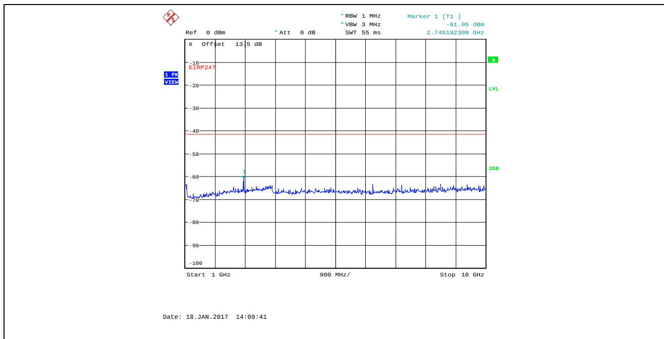
Plot 5.4.4.3.24. Conducted Spurious Emissions in Restricted Frequency Bands Bandwidth: 8 MHz, TX Gain Setting 36, Data Rate 4, 915 MHz, 1 GHz - 10 GHz, Peak Detector
