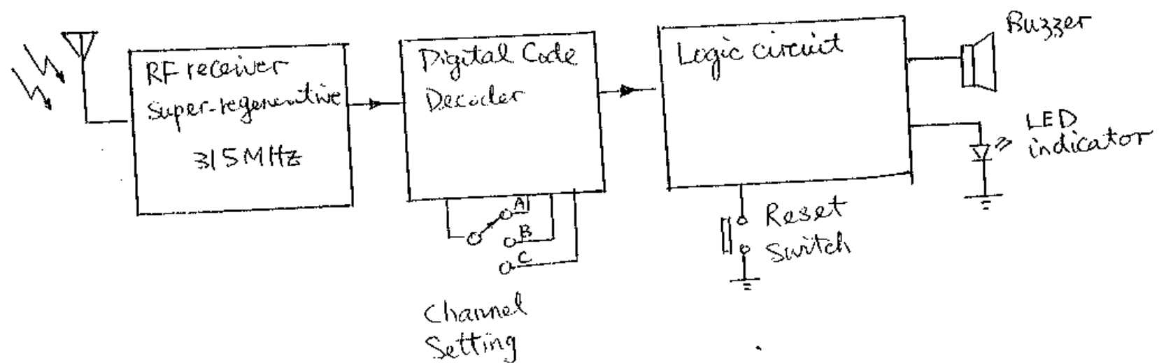
SYSTEM BLOCK DIAGRAM FOR MAIL GUARD
