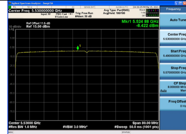
Test Mode:802. 11ax HE80 Ant8
