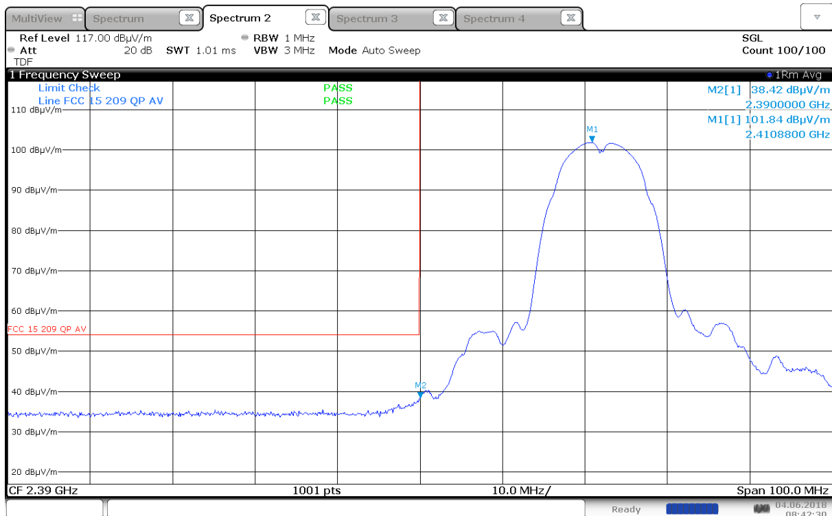
Lower Band Edge, Average, 2412 MHz, 802.11b, 1Mb, (Max: Ant 1, HP)
