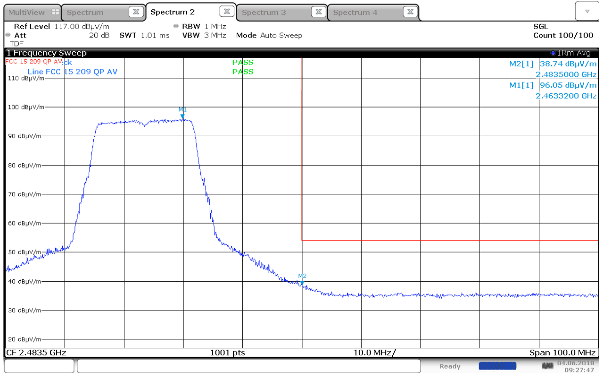
Upper Band Edge, Average, 2457 MHz, 802.11g, 6Mb, (Max: Ant 1, HP)
