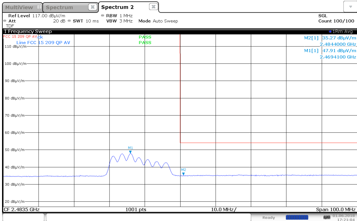
Upper Band Edge, Average, 2472 MHz, 802.11n, MCS0, MIMO (Max: HP)
