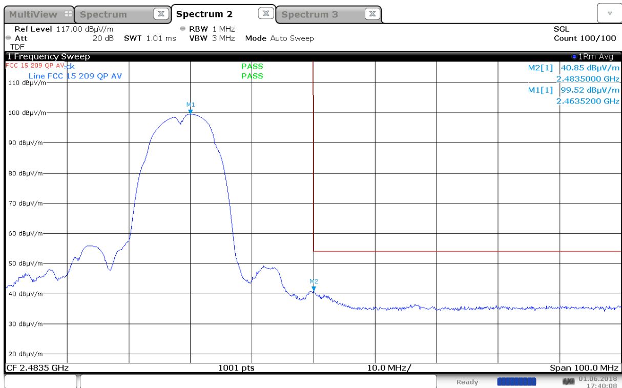
Upper Band Edge, Average, 2462 MHz, 802.11b, 1Mb, (Max: Ant 0, HP)
