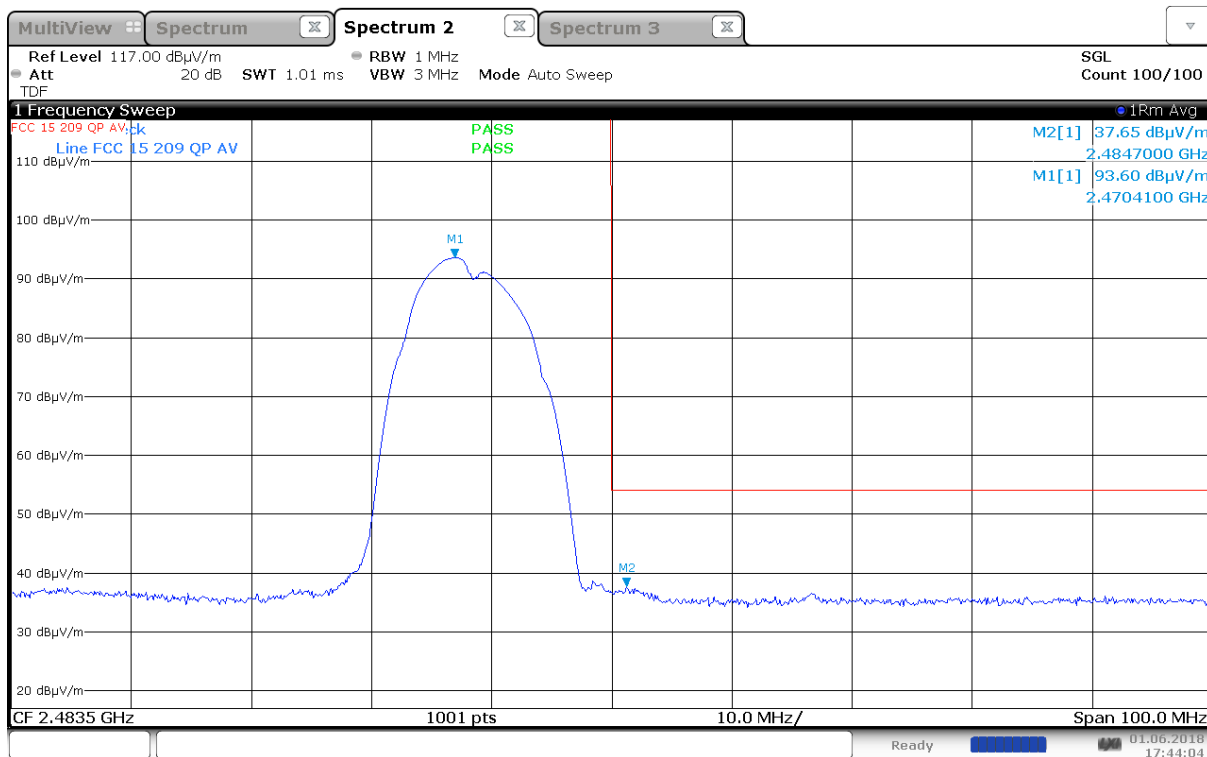
Upper Band Edge, Average, 2472 MHz, 802.11b, 1Mb, (Max: Ant 0, HP)
