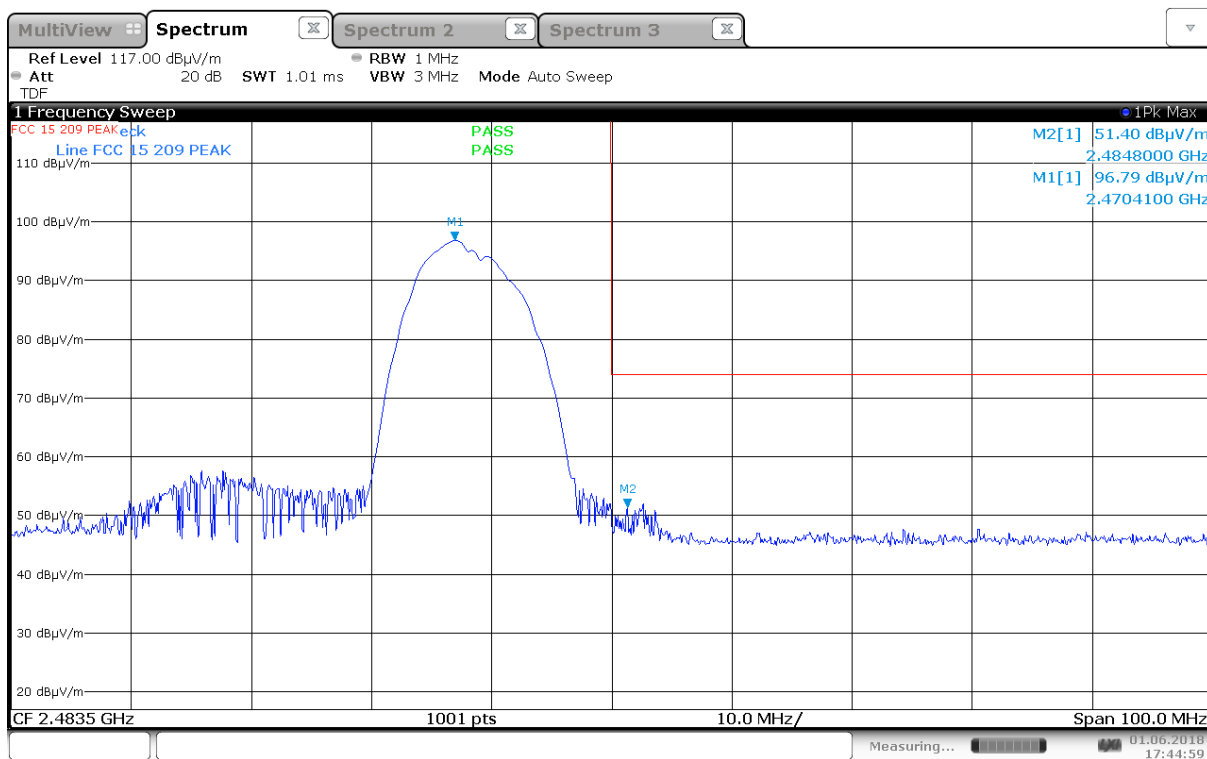
Upper Band Edge, Peak, 2472 MHz, 802.11b, 1Mb, (Max: Ant 0, HP)
