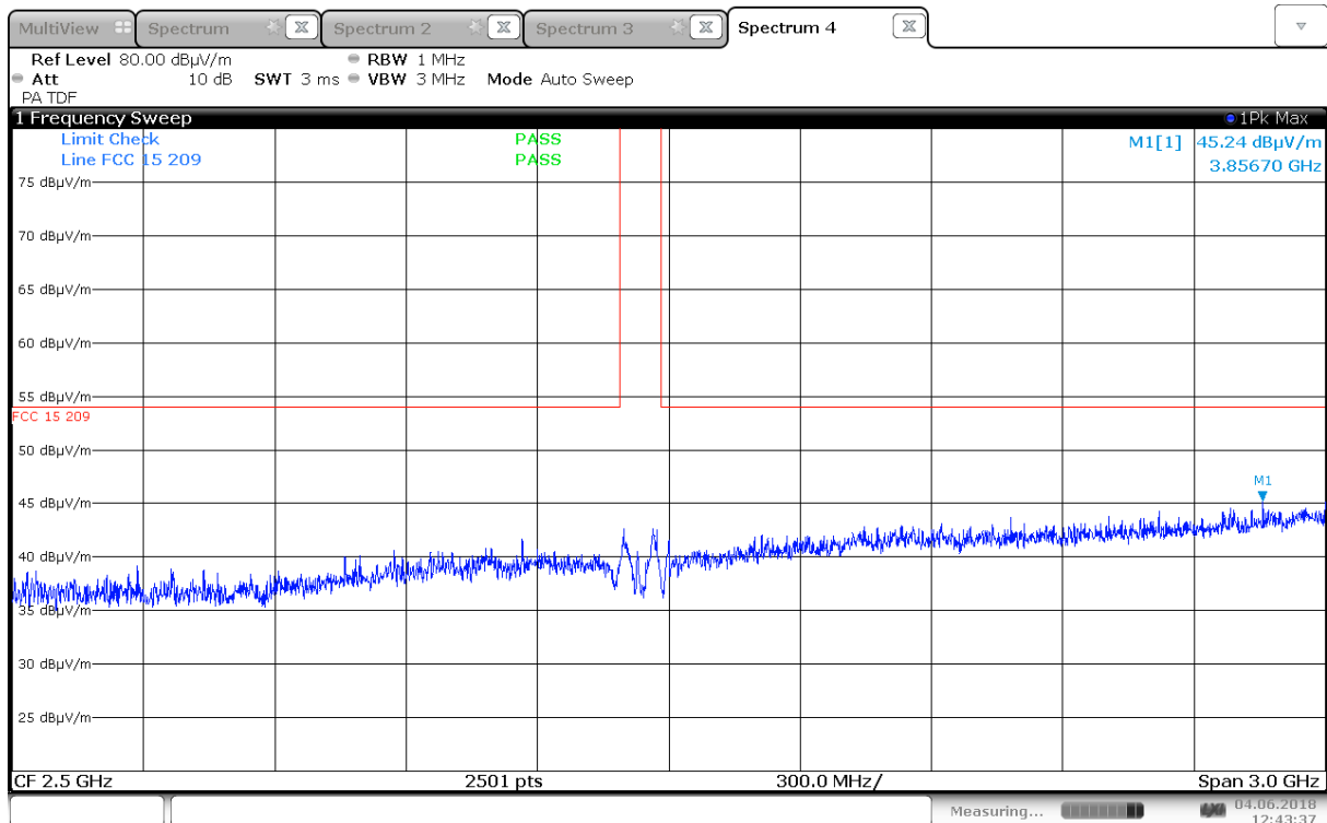
Radiated Emissions, 1000 -4000 MHz, 2462 MHz, 802.11b, 1Mb, Ant1, VP
