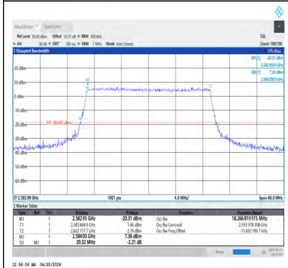
1-N41-30-20-M-7-CP-16QAM-Out_ Full-51@0-Ant1-18.267-20.320-≤20-PASS
