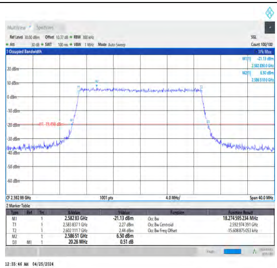
1-N41-30-20-M-6-CP-QPSK-Out_ Full-51@0-Ant1-18.275-20.280-≤20-PASS
