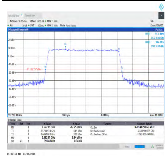
1-N41-30-40-M-1-DFT-QPSK-Outer_Full-100 @0-Ant1-36.015-39.040-≤40-PASS
