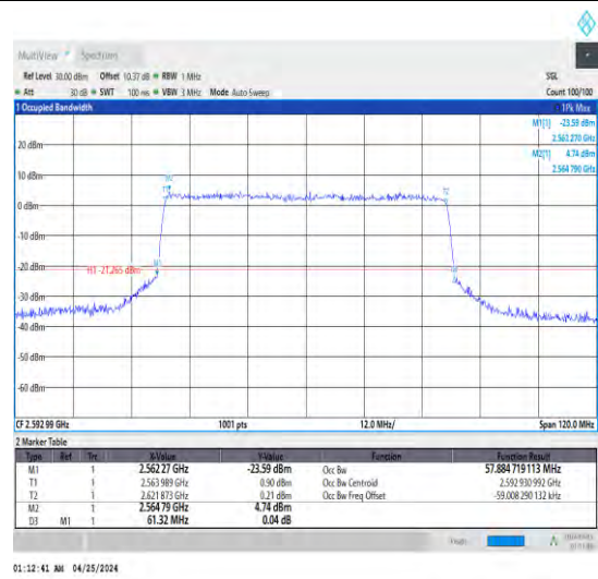
1-N41-30-60-M-8-CP-64QAM-Out_Full-162 @0-Ant1-57.885-61.320-≤60-PASS
