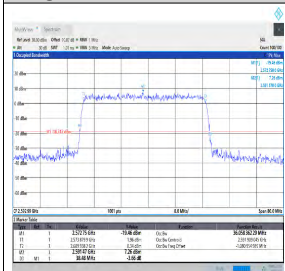
1-N41-30-40-M-3-DFT-16QAM-Outer_Full-10 @0-Ant1-36.058-38.480-≤40-PASS
