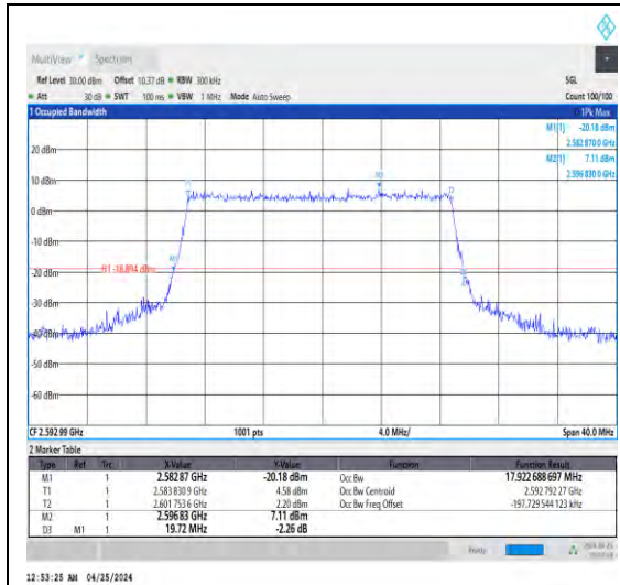
1-N41-30-20-M-1-DFT-QPSK-Outet_Full-50 @0-Ant1-17.923-19.720-≤20-PASS
