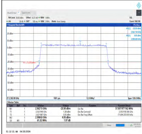
1-N41-30-60-M-7-CP-16QAM-Out_Full-162 @0-Ant1-57.938-61.320-≤60-PASS
