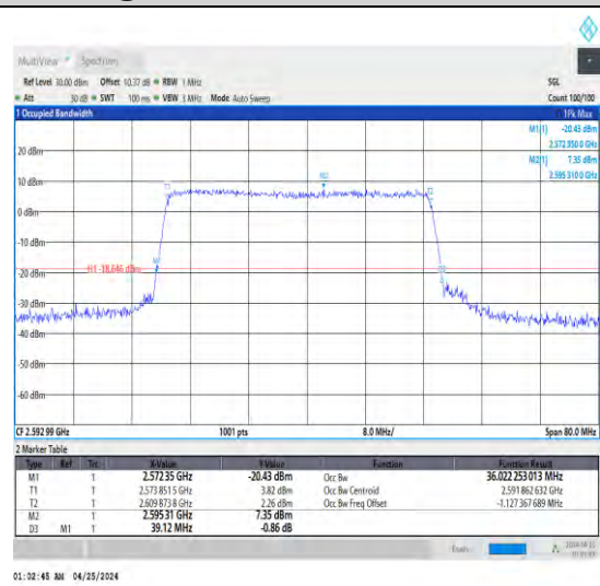
1-N41-30-40-M-4-DFT-64QAM-Outer_Full-10 @0-Ant1-36.022-39.120-≤40-PASS
