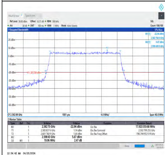
1-N41-30-20-M-3-DFT-16QAM-Outet_Full-50 @0-Ant1-17.923-19.960-≤20-PASS
