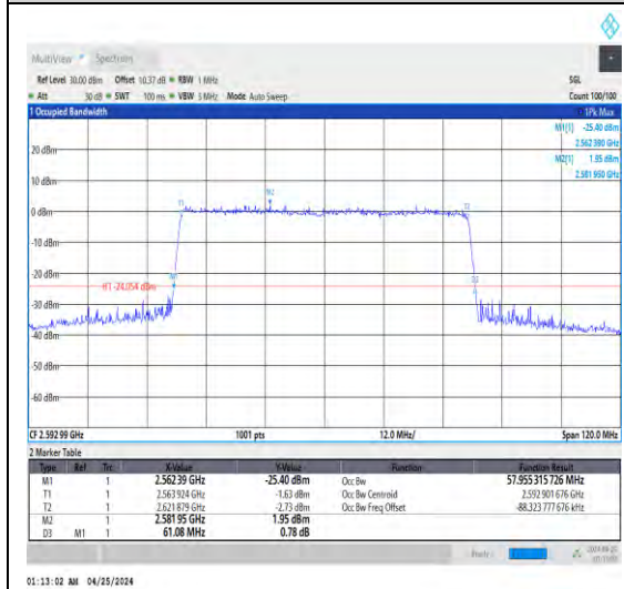
1-N41-30-60-M-9-CP-256QAM-Out_Full-16 2@0-Ant1-57.955-61.080-≤60-PASS
