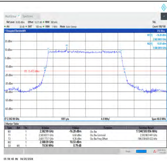
1-N41-30-20-M-2-DFT-PI2BPSK-Outet_Full-50 @0-Ant1-17.941-19.560-≤20-PASS
