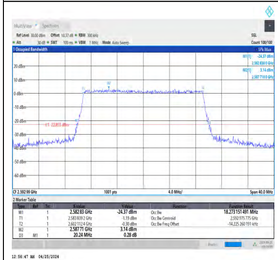
1-N41-30-20-M-9-CP-256QAM-Out_ Full-51@0-Ant1-18.273-20.240-≤20-PASS
