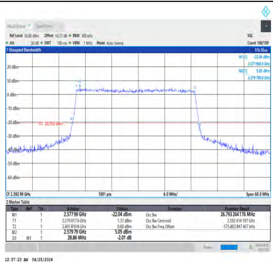
1-N41-30-30-M-1-DFT-QPSK-Out_ Full-75@0-Ant1-26.793-28.860-≤30-PASS
