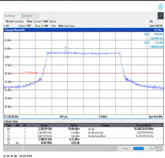
1-N41-30-20-M-8-CP-64QAM-Out_ Full-51@0-Ant1-18.268-20.040-≤20-PASS
