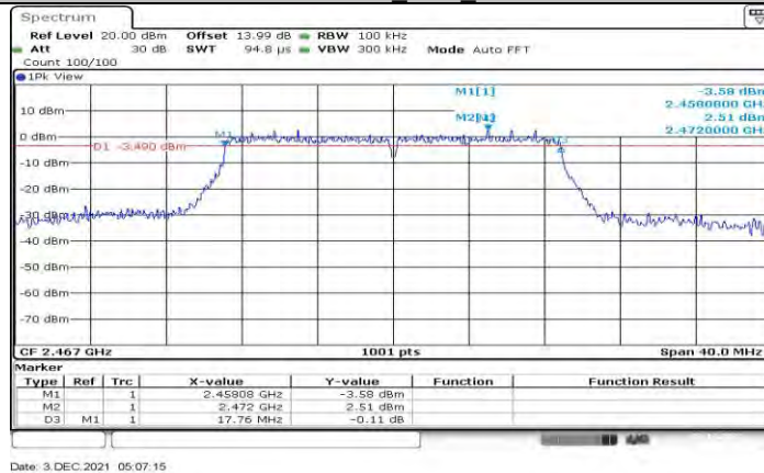
11N20SISO Ant1_2467
