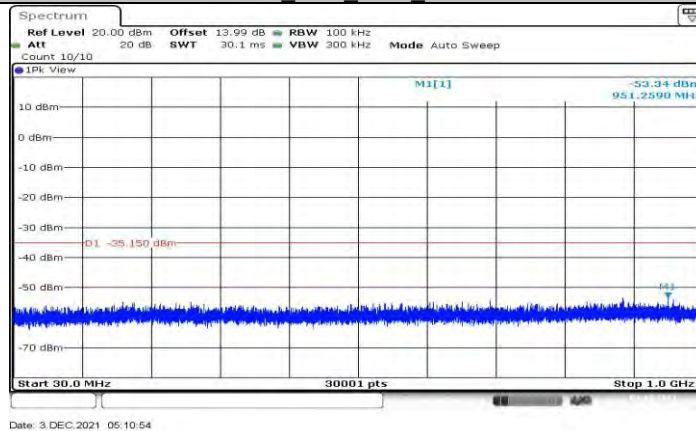
11N20SISO Ant1_2472_30~1000
