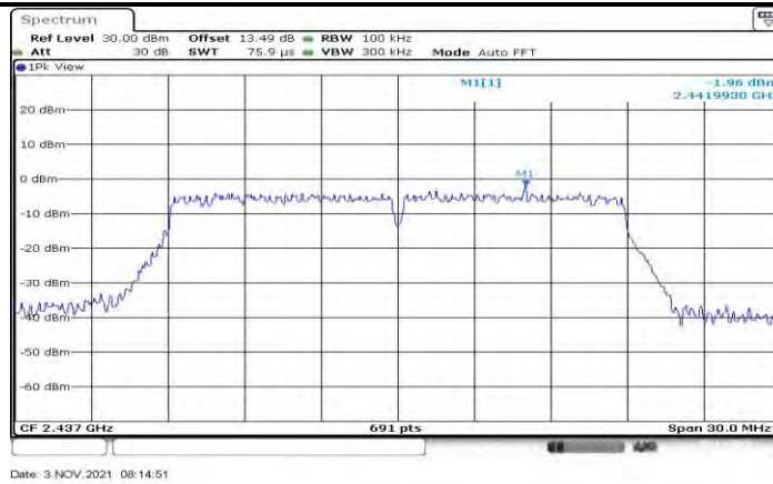
11N20SISO_Ant1_2437_0~Reference
