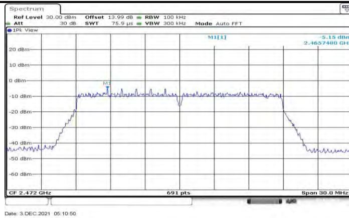
11N20SISO Ant1_2472_0~Reference
