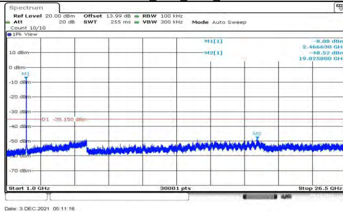
11N20SISO Ant1_2472_1000~26500
