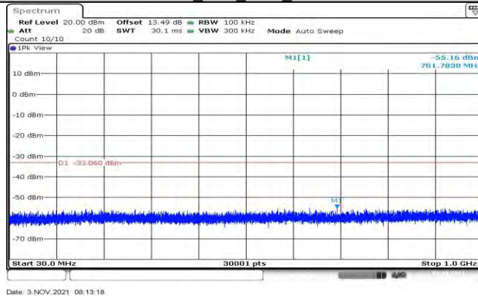
11N20SISO Ant1 2412 30~1000
