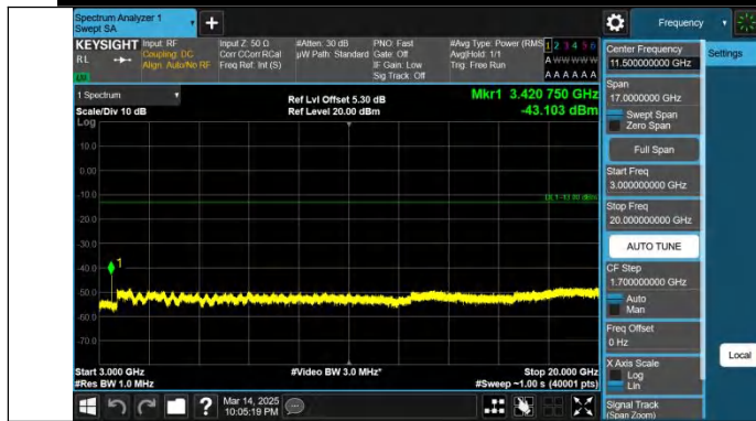
Band66-5MHz-QPSK-131997-1RB#0-3000~20000-PASS
