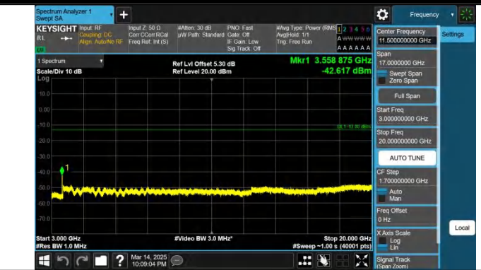
Band66-5MHz-QPSK-132647-1RB#24-3000~20000-PASS
