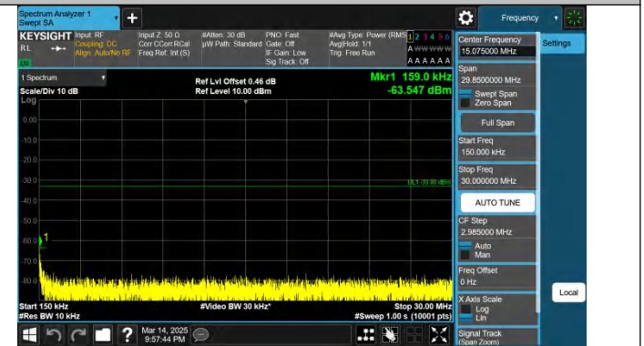
Band66-3MHz-QPSK-132657-1RB#0-0.15~30-PASS
