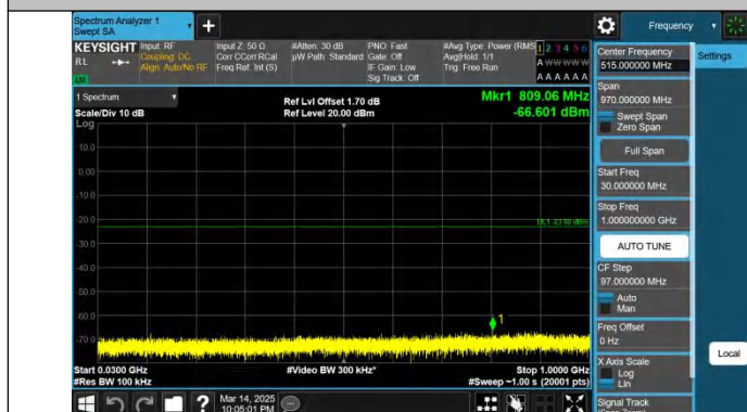
Band66-5MHz-QPSK-131997-1RB#0-30~1000-PASS
