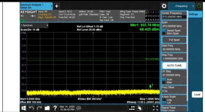
Band66-20MHz-QPSK-132572-1RB#99-30~1000-PASS
