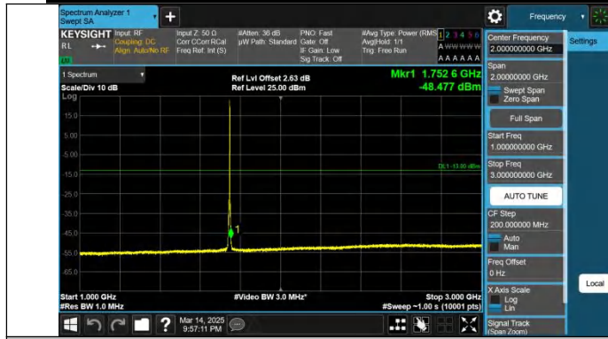
Band66-3MHz-QPSK-132322-1RB#14-1000~3000-PASS
