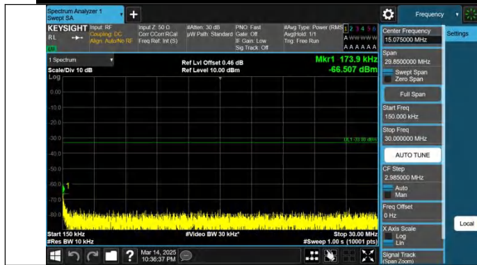
Band66-20MHz-QPSK-132572-1RB#99-0.15~30-PASS
