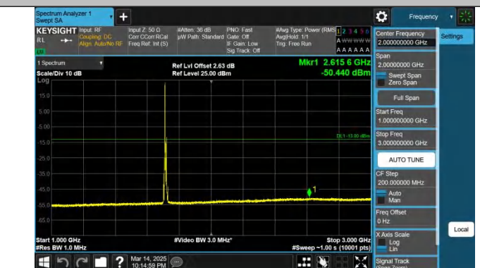
Band66-10MHz-QPSK-132022-1RB#0-1000~3000-PASS
