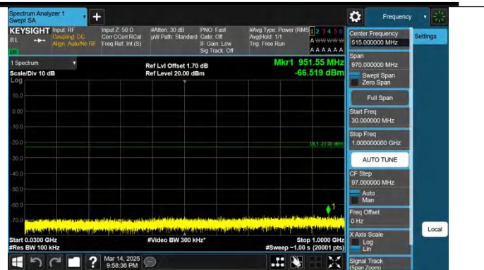
Band66-3MHz-QPSK-132657-1RB#14-30~1000-PASS
