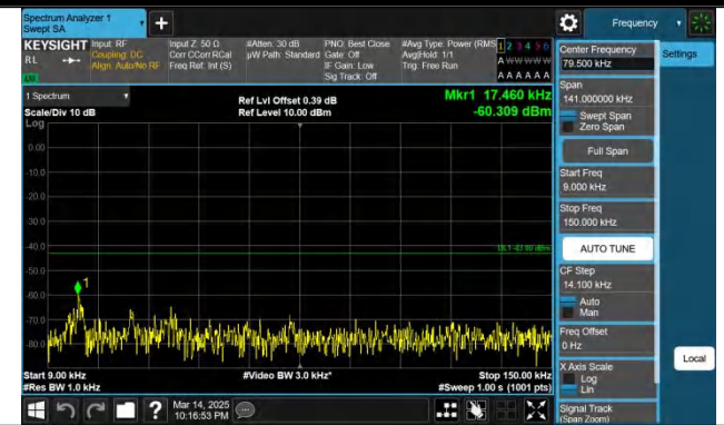
Band66-10MHz-QPSK-132322-1RB#49-0.009~0.15-PASS
