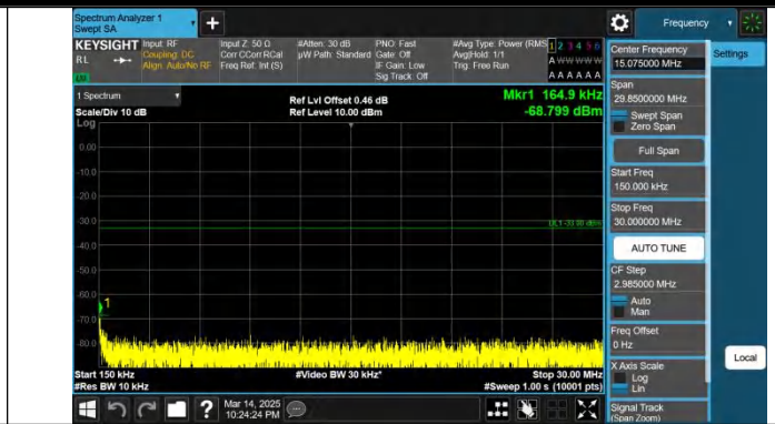
Band66-15MHz-QPSK-132047-1RB#0-0.15~30-PASS
