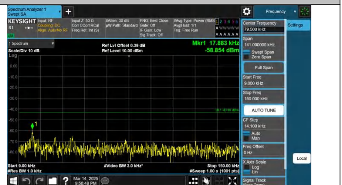
Band66-3MHz-QPSK-132322-1RB#14-0.009~0.15-PASS
