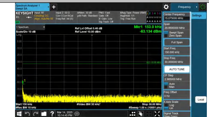
Band66-10MHz-QPSK-132022-1RB#0-0.15~30-PASS
