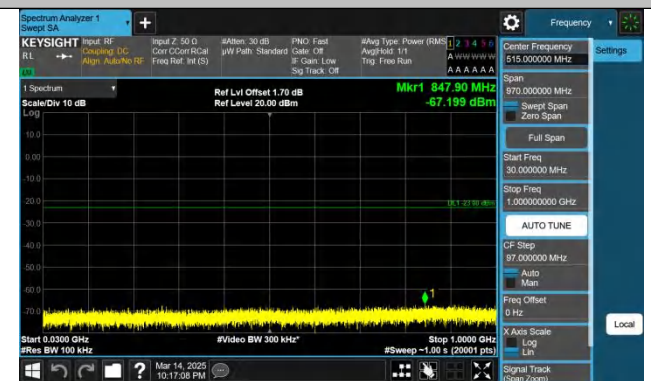
Band66-10MHz-QPSK-132322-1RB#49-30~1000-PASS
