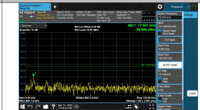
Band66-20MHz-QPSK-132322-1RB#99-0.009~0.15-PASS
