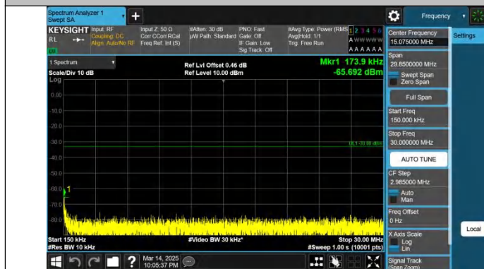
Band66-5MHz-QPSK-131997-1RB#24-0.15~30-PASS
