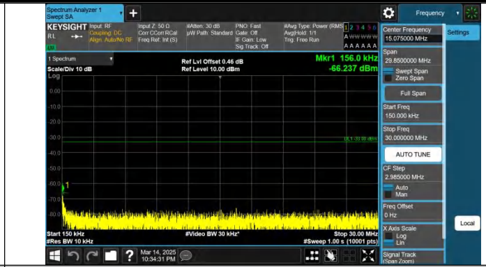
Band66-20MHz-QPSK-132322-1RB#0-0.15~30-PASS
