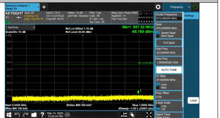
Band66-5MHz-QPSK-131997-1RB#24-30~1000-PASS
