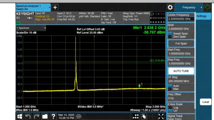
Band66-15MHz-QPSK-132322-1RB#0-1000~3000-PASS
