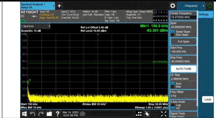
Band66-5MHz-QPSK-132647-1RB#0-0.15~30-PASS
