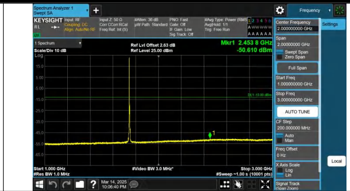
Band66-5MHz-QPSK-132322-1RB#0-1000~3000-PASS
