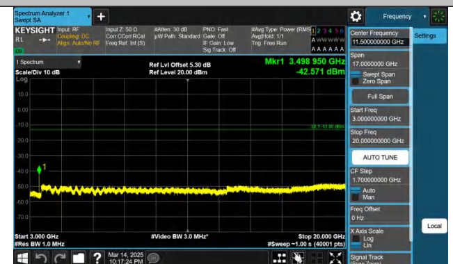
Band66-10MHz-QPSK-132322-1RB#49-3000~20000-PASS
