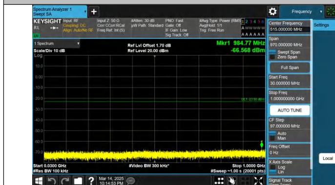
Band66-10MHz-QPSK-132022-1RB#0-30~1000-PASS
