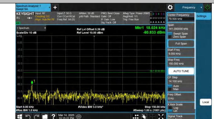
Band66-10MHz-QPSK-132022-1RB#49-0.009~0.15-PASS
