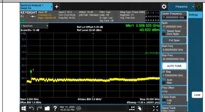
Band66-20MHz-QPSK-132572-1RB#99-3000~20000-PASS
