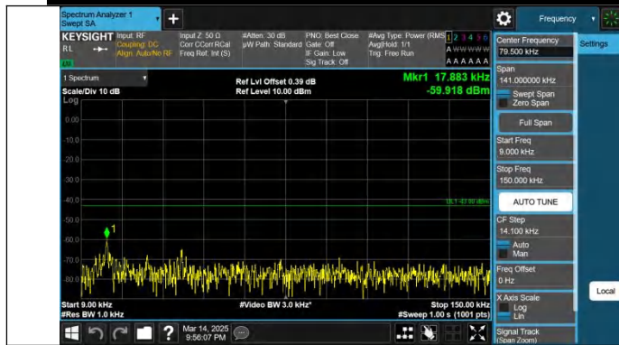
Band66-3MHz-QPSK-132322-1RB#0-0.009~0.15-PASS
