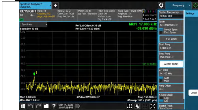
Band66-5MHz-QPSK-132647-1RB#0-0.009~0.15-PASS
