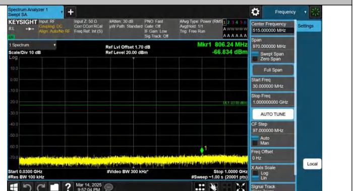
Band66-3MHz-QPSK-132322-1RB#14-30~1000-PASS
