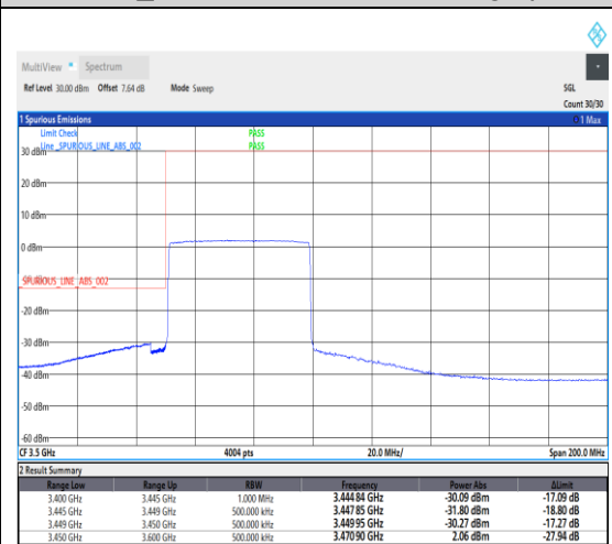
1-N78-3450-3550--30-50-L-6-CP-QPSK-Outer_Full-133@0-Ant1-1---see graph
