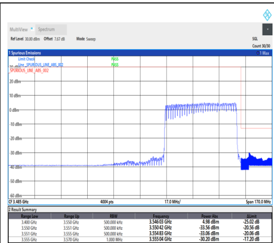
1-N78-3450-3550--30-50-H-3-DFT-PI2BPSK-Outer_Full-128@0-Ant1-1---see graph
