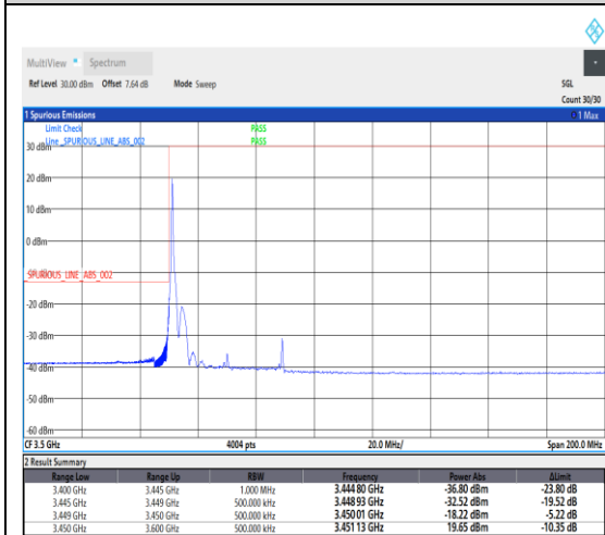
1-N78-3450-3550--30-40-L-4-CP-QPSK-Edge_1RB_Left-1@0-Ant1-1---see graph
