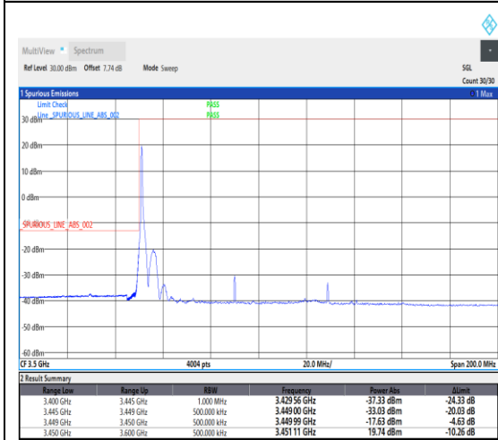
1-N78-3450-3550--30-80-L-4-CP-QPSK-Edge_1RB_Left-1@0-Ant1-1---see graph
