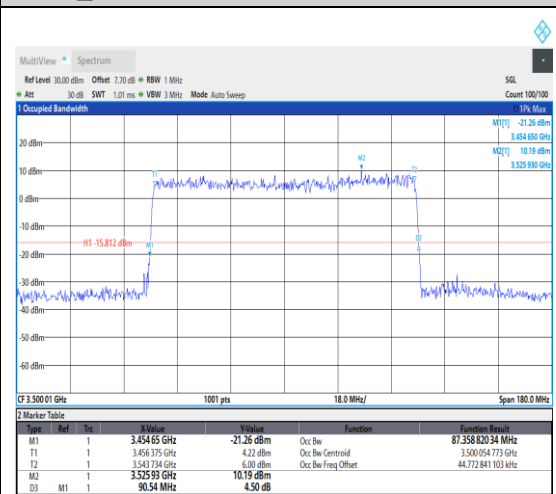
1-N78-3450-3550--30-90-M-9-CP-256QAM-Out_ Full-245@0-Ant1-87.359-90.540-≤90-
