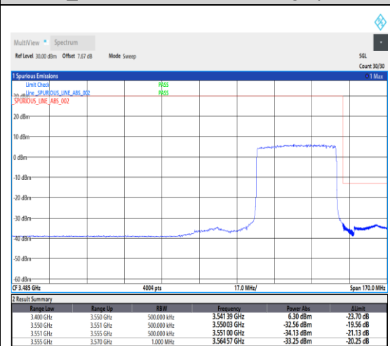
1-N78-3450-3550--30-40-H-3-DFT-PI2BPSK-Outer_Full-100@0-Ant1-1---see graph
