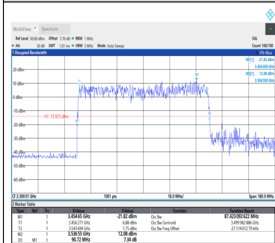
1-N78-3450-3550--30-90-M-6-CP-QPSK-Out_ Full-245@0-Ant1-87.423-90.720-≤90-
