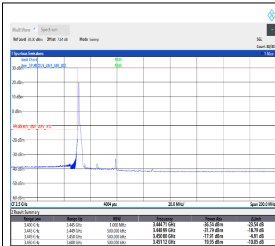
1-N78-3450-3550--30-30-L-4-CP-QPSK-Edge_1RB_Left-1@0-Ant1-1---see graph
