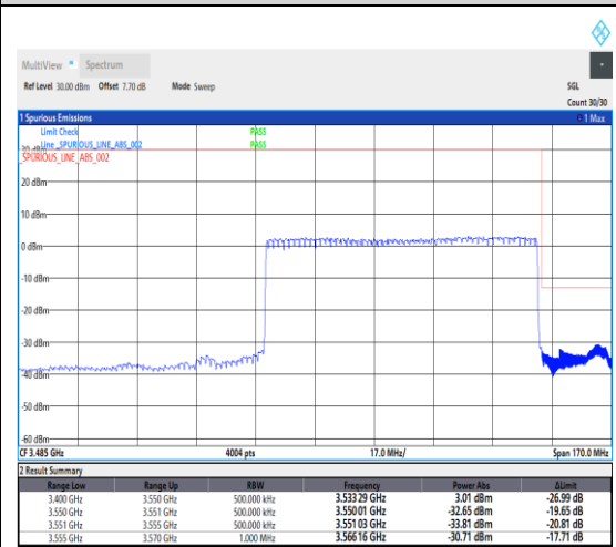
1-N78-3450-3550--30-80-H-3-DFT-PI2BPSK-Outer_Full-216@0-Ant1-1---see graph
