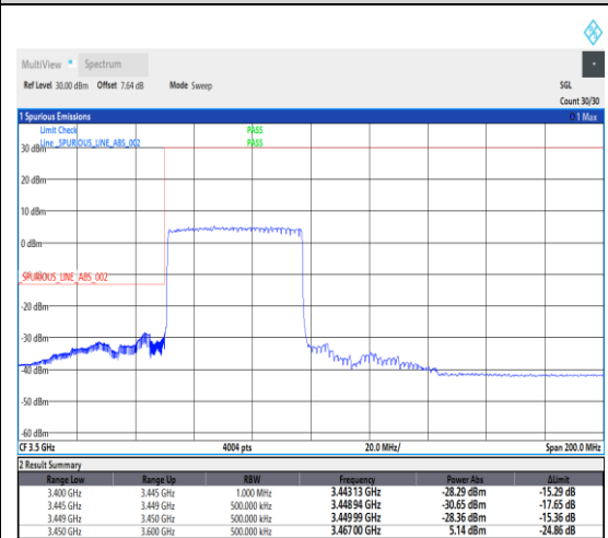
1-N78-3450-3550--30-50-L-3-DFT-PI2BPSK-Outer_Full-128@0-Ant1-1---see graph
