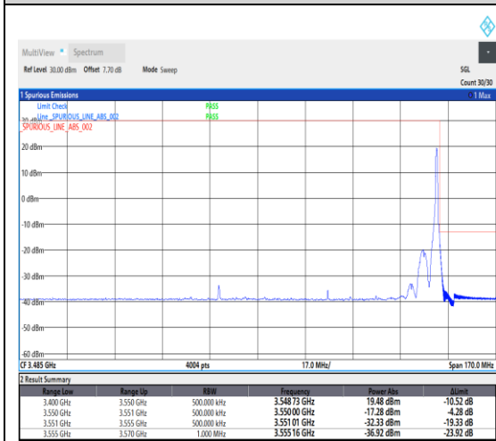
1-N78-3450-3550--30-80-H-2-DFT-PI2BPSK-Edge_1RB_Right-1@216-Ant1-1---see graph
