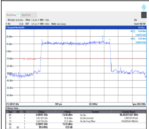
1-N78-3450-3550--30-100-L-2-DFT-PI2BPSK-Outer_Full-270@0-Ant1-96.343-99.600≤100-
