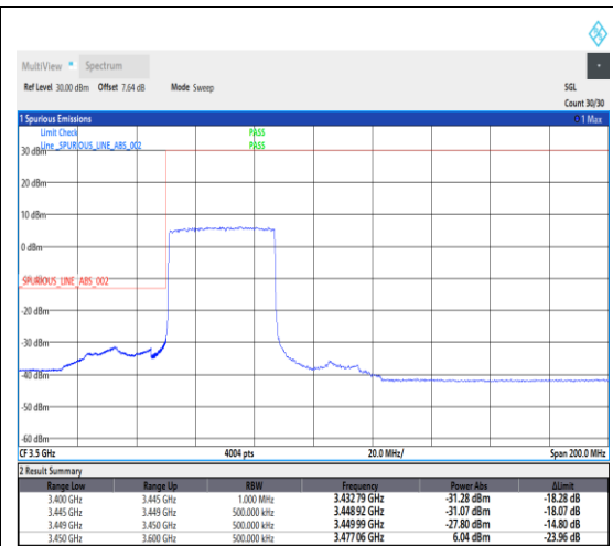
1-N78-3450-3550--30-40-L-3-DFT-PI2BPSK-Outer_Full-100@0-Ant1-1---see graph
