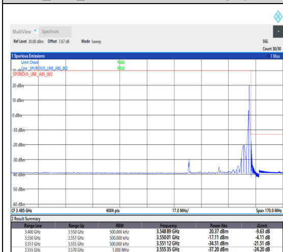
1-N78-3450-3550--30-40-H-2-DFT-PI2BPSK-Edge_1RB_Right-1@105-Ant1-1---see graph
