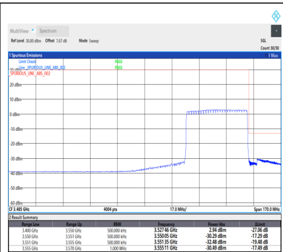
1-N78-3450-3550--30-40-H-6-CP-QPSK-Out_er_Full-106@0-Ant1-1---see graph
