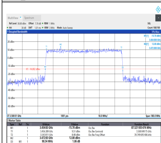
1-N78-3450-3550--30-90-M-8-CP-64QAM-Out_ Full-245@0-Ant1-87.522-90.540-≤90-
