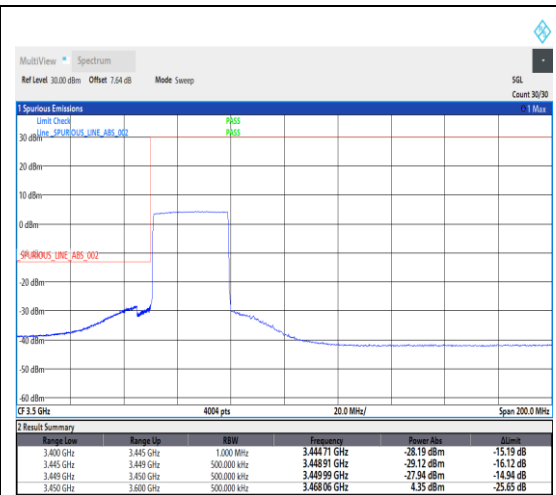
1-N78-3450-3550--30-30-L-6-CP-QPSK-Outer_Full-78@0-Ant1-1---see graph
