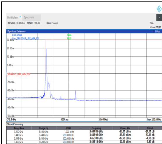
1-N78-3450-3550--30-40-L-1-DFT-PI2BPSK-Edge_1RB_Left-1@0-Ant1-1---see graph
