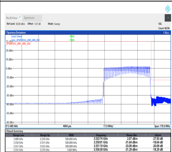
1-N78-3450-3550--30-50-H-6-CP-QPSK-Outer_Full-133@0-Ant1-1---see graph
