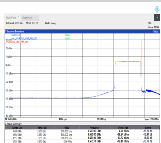
1-N78-3450-3550--30-30-H-6-CP-QPSK-Outer_Full-78@0-Ant1-1---see graph
