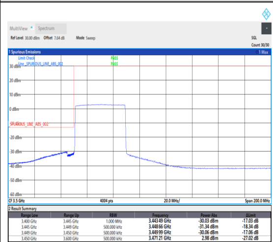
1-N78-3450-3550--30-40-L-6-CP-QPSK-Outer_Full-106@0-Ant1-1---see graph
