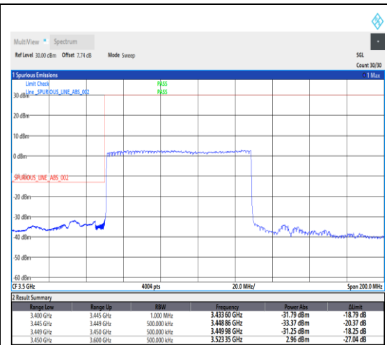
1-N78-3450-3550--30-80-L-3-DFT-PI2BPSK-Outer_Full-216@0-Ant1-1---see graph
