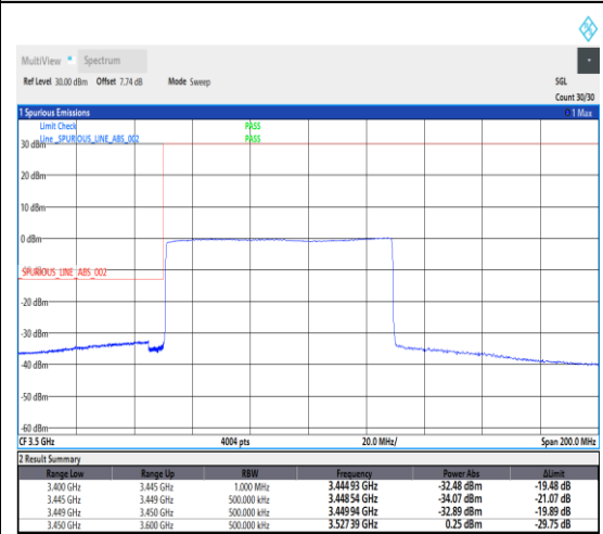
1-N78-3450-3550--30-80-L-6-CP-QPSK-Outer_Full-217@0-Ant1-1---see graph
