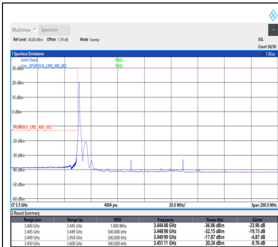
1-N78-3450-3550--30-80-L-1-DFT-PI2BPSK-Edge_1RB_Left-1@0-Ant1-1---see graph
