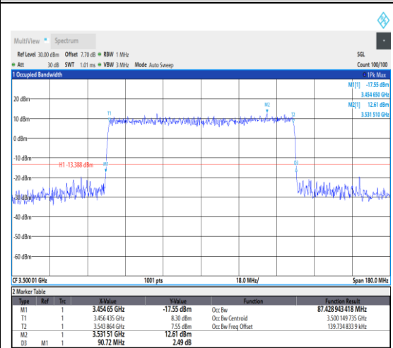
1-N78-3450-3550--30-90-M-7-CP-16QAM-Out_ Full-245@0-Ant1-87.429-90.720-≤90-
