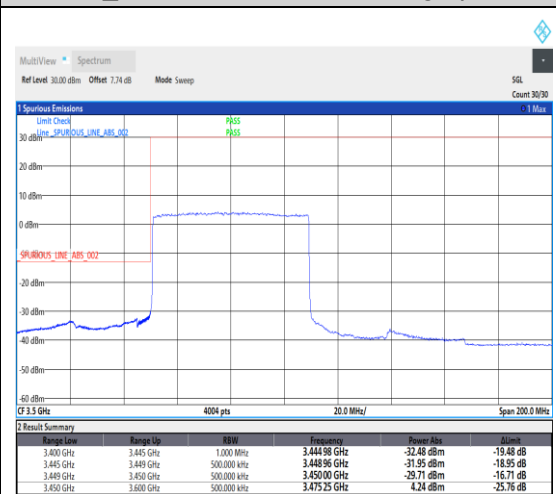
1-N78-3450-3550--30-60-L-3-DFT-PI2BPSK-Outer_Full-162@0-Ant1-1---see graph
