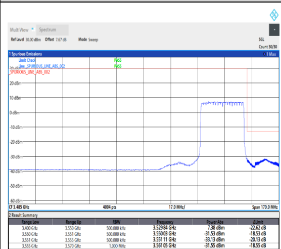
1-N78-3450-3550--30-30-H-3-DFT-PI2BPSK-Outer_Full-75@0-Ant1-1---see graph
