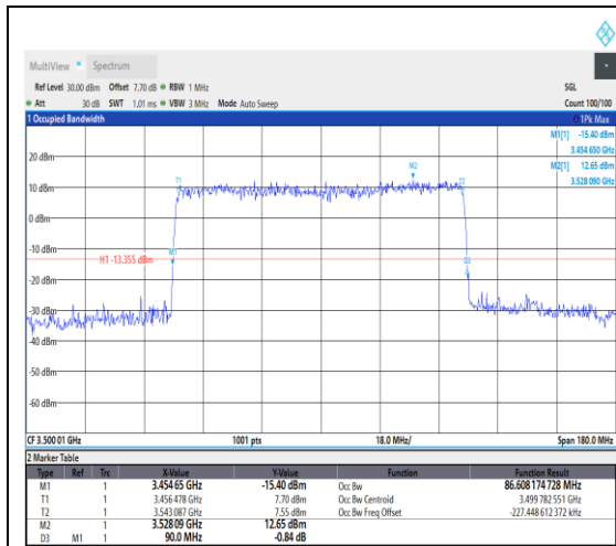
1-N78-3450-3550--30-90-M-4-DFT-64QAM-Outer_Full-243@0-Ant1-86.608-90.000-≤90-
