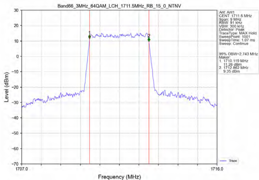
Band66_3MHz_64QAM_LCH_1711.5MHz_RB_15_0_NTNV
