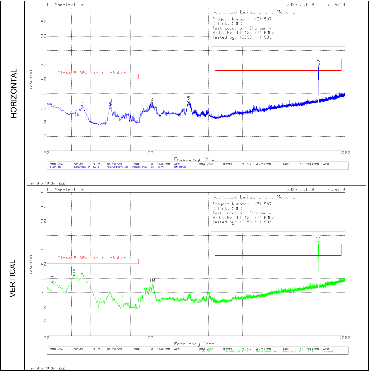
Radiated Emissions Graph
