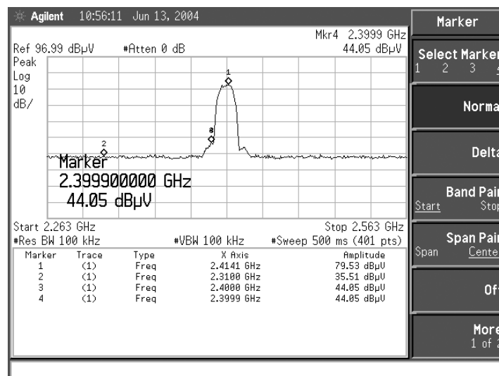
Figure Channel 1: (Horizontal)
