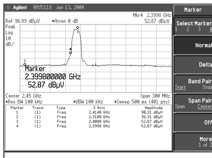
Figure Channel 1: (Vertical)
