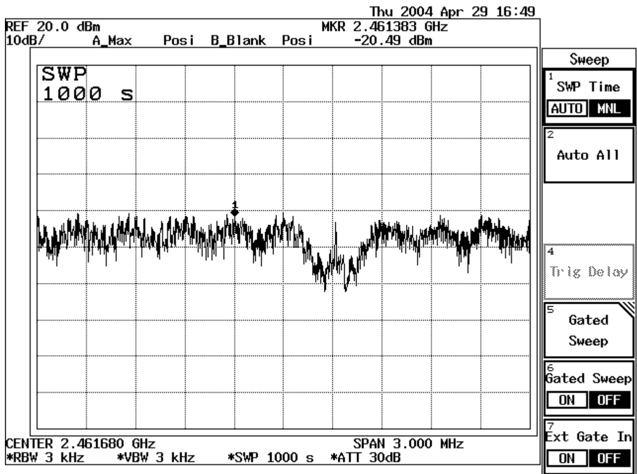
Figure Channel 11: 54Mbps
