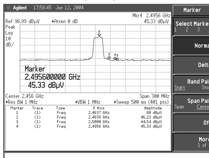
Figure Channel 11: (Vertical)
