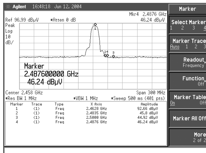
Figure Channel 11: (Vertical)
