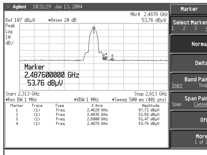
Figure Channel 11: (Vertical)
