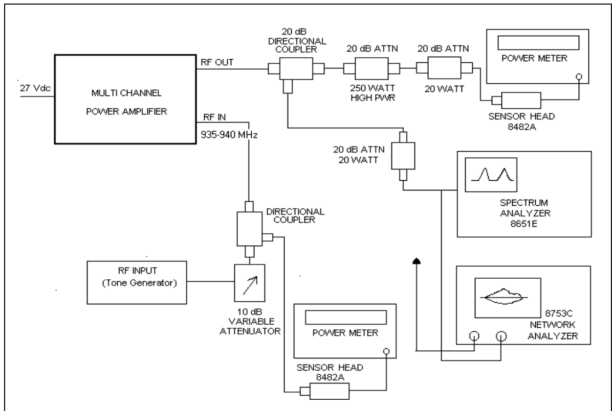
Amplifier Test Setup Diagram
