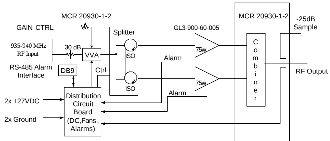
System Block Diagram
