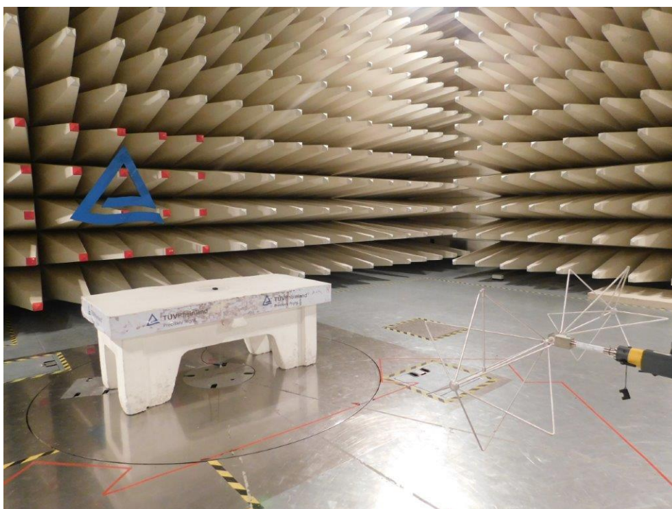
Photo 6: Horizontal polarization
