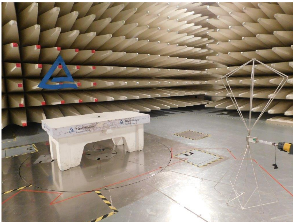
Photo 5: Vertical polarization
