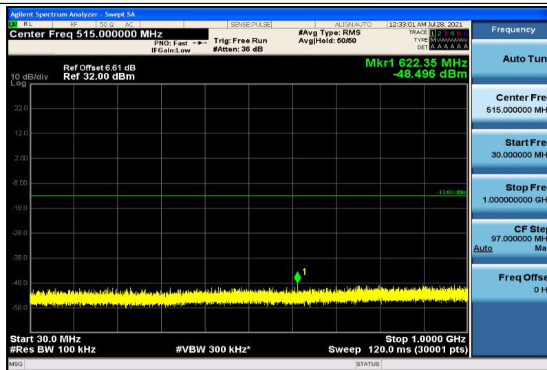
Band2-3MHz-16QAM-18615-1RB#0-30~1000MHz
