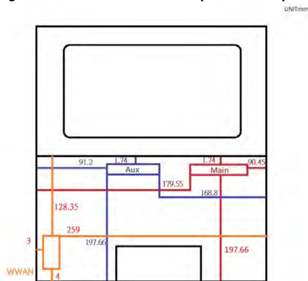
Fig.14 Antenna location of EUT (Tablet mode)
