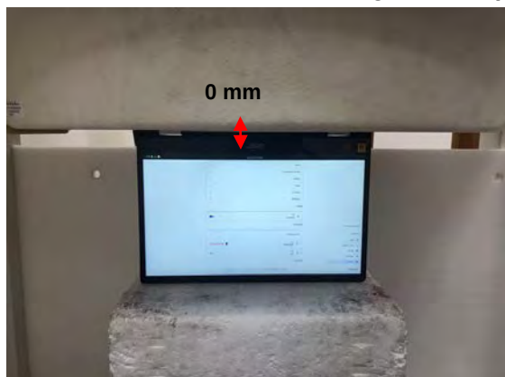
Fig.5 EUT Bottom side (Tablet mode) to flat phantom
