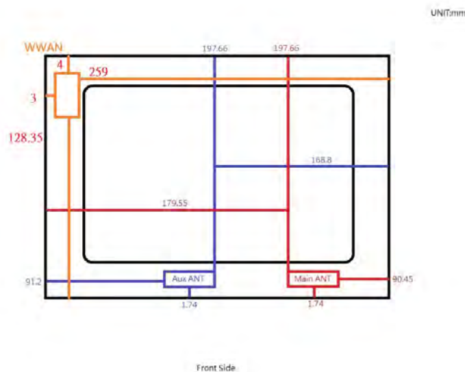
Fig.14 Antenna location of EUT (Tablet mode)
