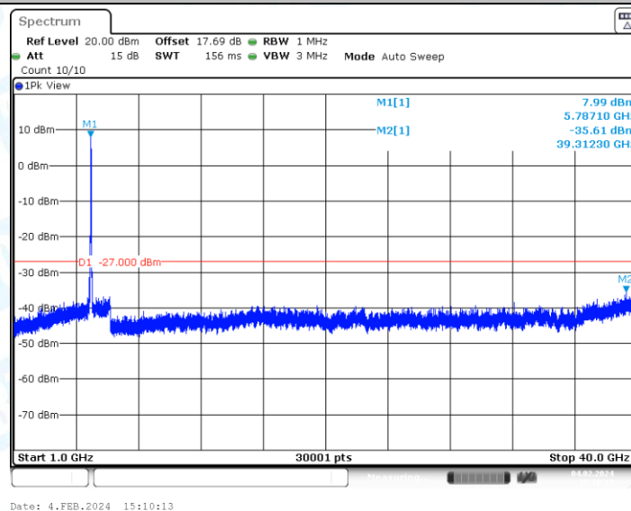
11AX40SISO_Ant1_5795_1000~40000
