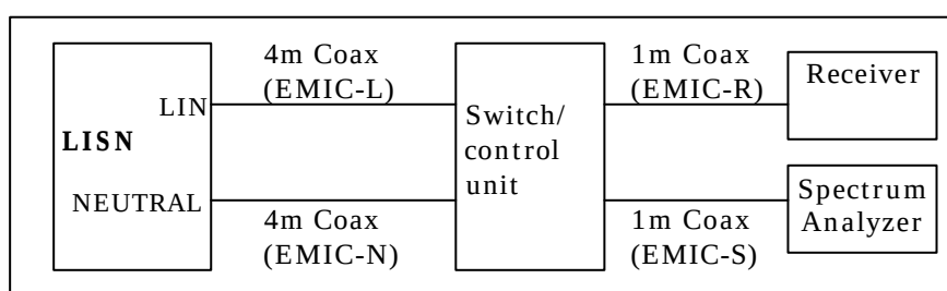
Figure 5. Cables for Conducted Emission Test
