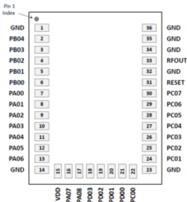
Figure 10: Lyra 24P 36-Pin PCB Module With LF Crystal Device Pinout
