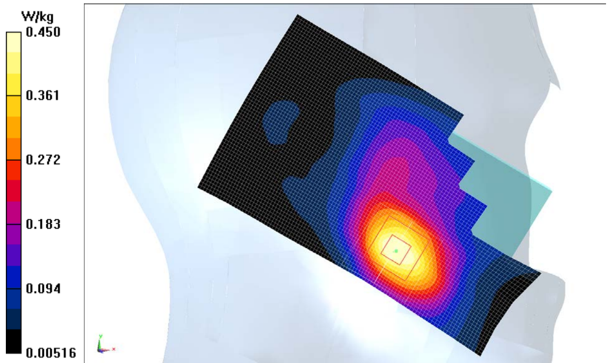
Fig.4 1900 MHz
