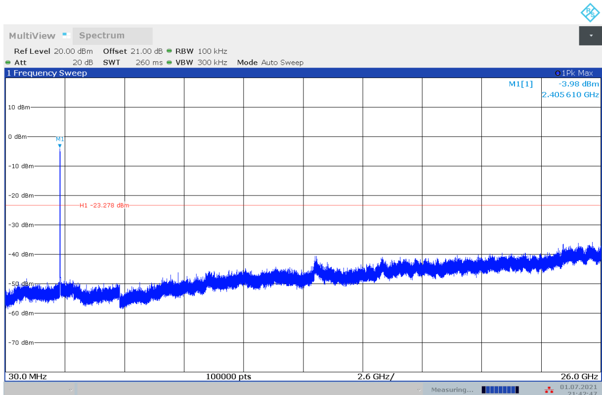
Fig.A.6.1.86 Transmitter Spurious Emission - Conducted (802.11n-HT20, Ch1, 30 MHz-26
