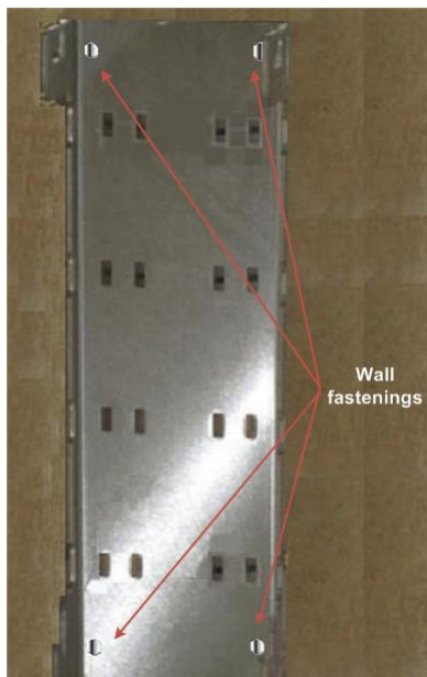
Figure 16 - wall mounting plate fastened on wall
