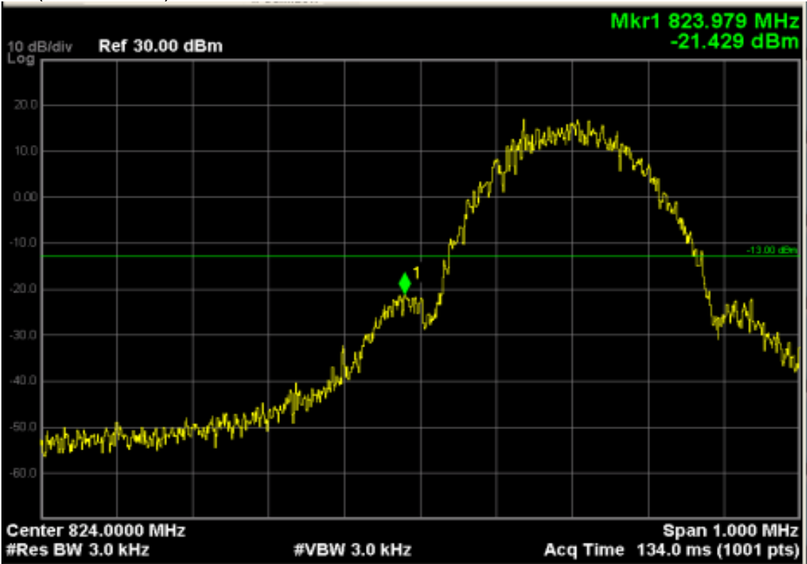
GSM850 (EDGE 8 Link), Channel 128
