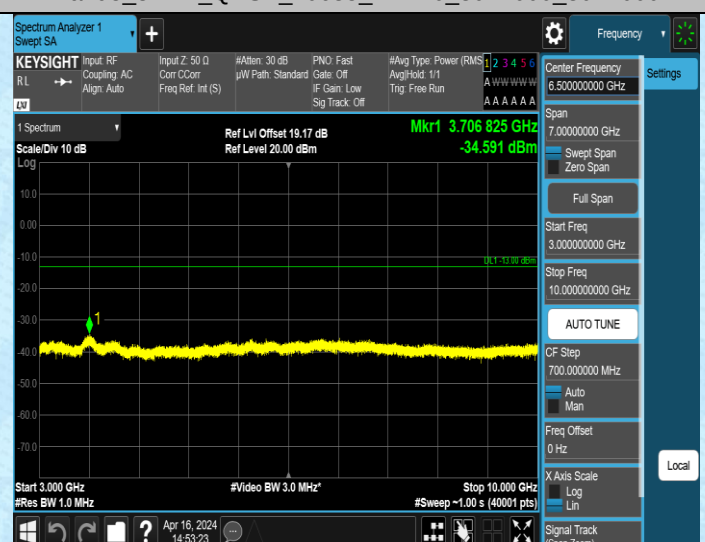
Band5 3MHz QPSK 20635 1RB#0 3000~10000 3000~10000
