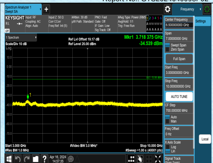
Band5_10MHz_QPSK_20450_1RB#0_3000~10000_3000~1000 0
