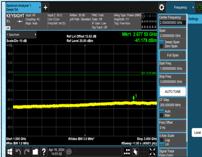
Band5_3MHz_QPSK_20415_1RB#0_1000-3000_1000-3000
