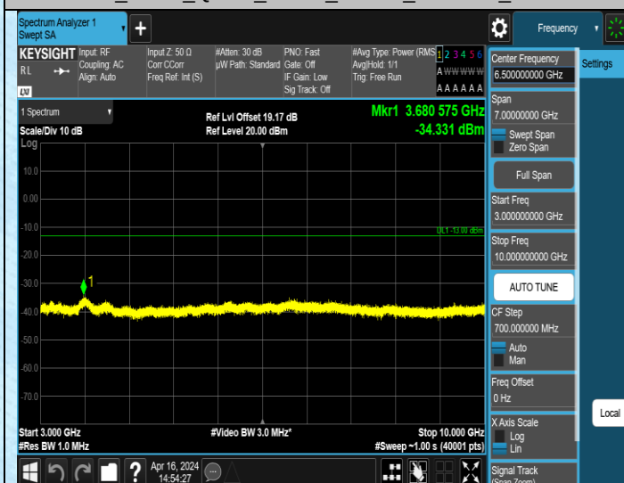
Band5_5MHz_QPSK_20425_1RB#0_3000~10000_3000~10000
