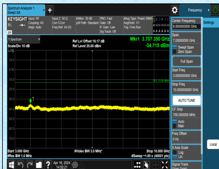
Band5 3MHz QPSK 20525 1RB#0 3000~10000 3000~10000
