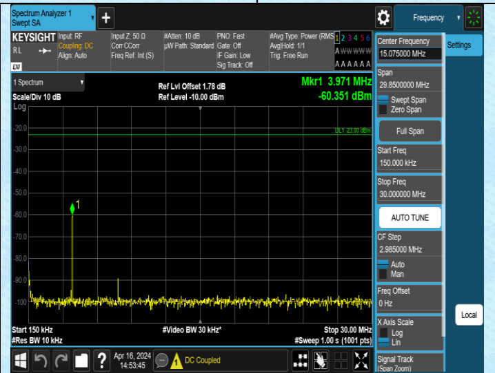
Band5_5MHz_QPSK_20425_1RB#0_0.15~30_0.15~30
