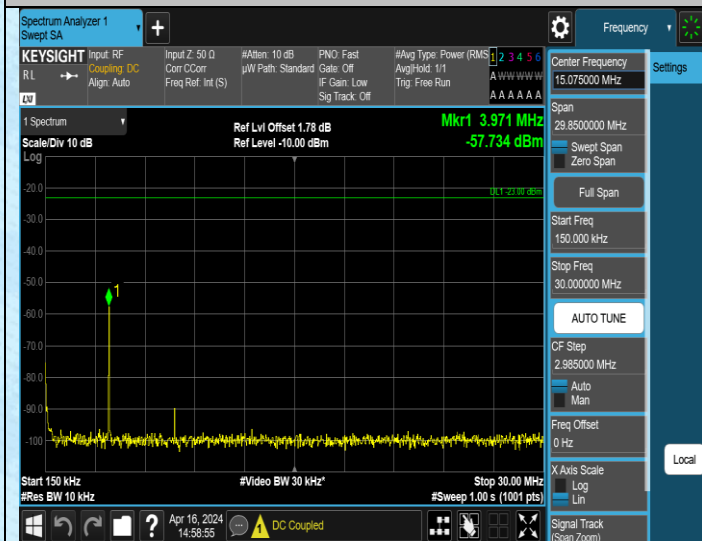
Band5_10MHz_QPSK_20600_1RB#0_0.15~30_0.15~30
