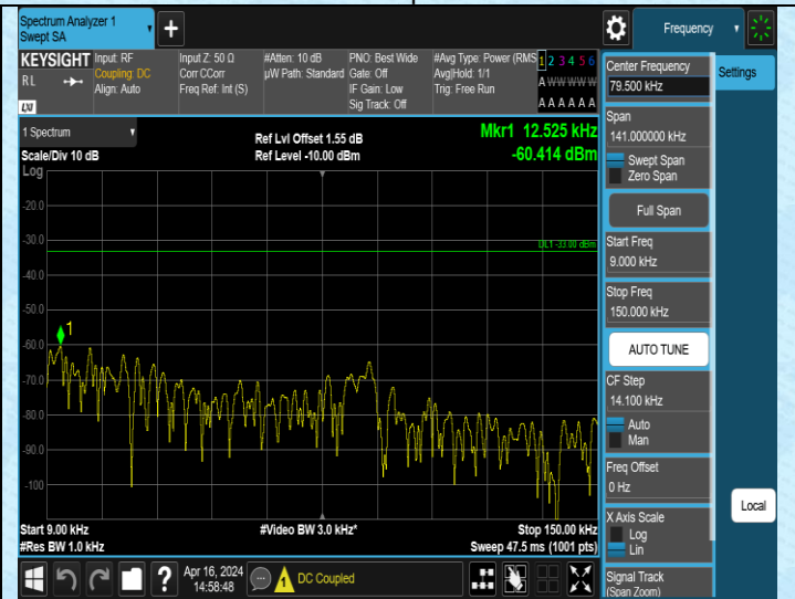
Band5_10MHz_QPSK_20600_1RB#0_0.009~0.15_0.009~0.15
