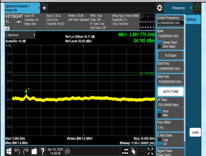
Band5_10MHz_QPSK_20600_1RB#0_3000~10000_3000~1000
