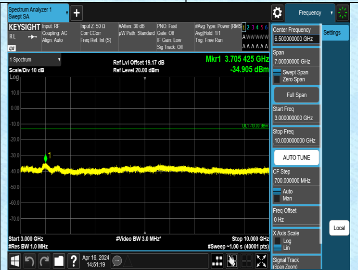
Band5_3MHz_QPSK_20415_1RB#0_3000-10000_3000-10000
