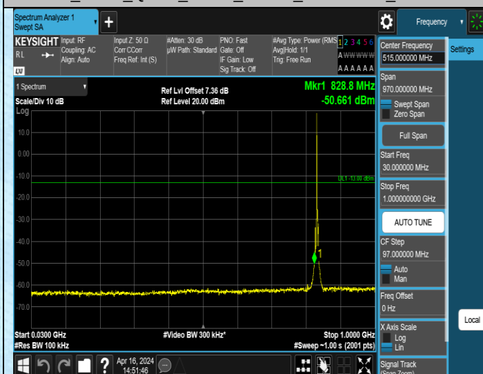
Band5_3MHz_QPSK_20525_1RB#0_30-1000_30-1000
