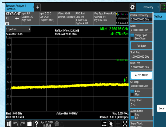
Band5_10MHz_QPSK_20450_1RB#0_1000~3000_1000~3000
