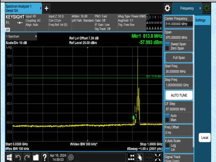
Band5_10MHz_QPSK_20600_1RB#0_30~1000_30~1000
