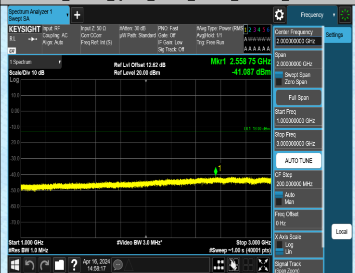
Band5_10MHz_QPSK_20525_1RB#0_1000~3000_1000~3000
