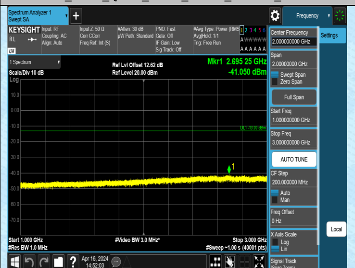
Band5_3MHz_QPSK_20525_1RB#0_1000-3000_1000-3000
