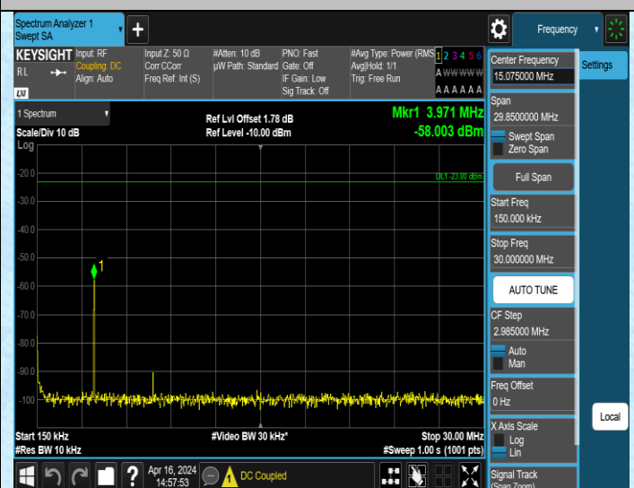
Band5_10MHz_QPSK_20525_1RB#0_0.15~30_0.15~30
