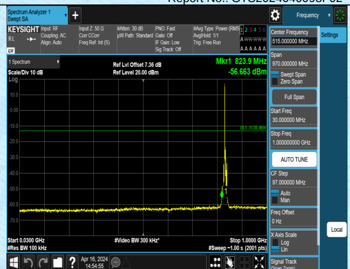
Band5 5MHz QPSK 20525 1RB#0 30~1000 30~1000
