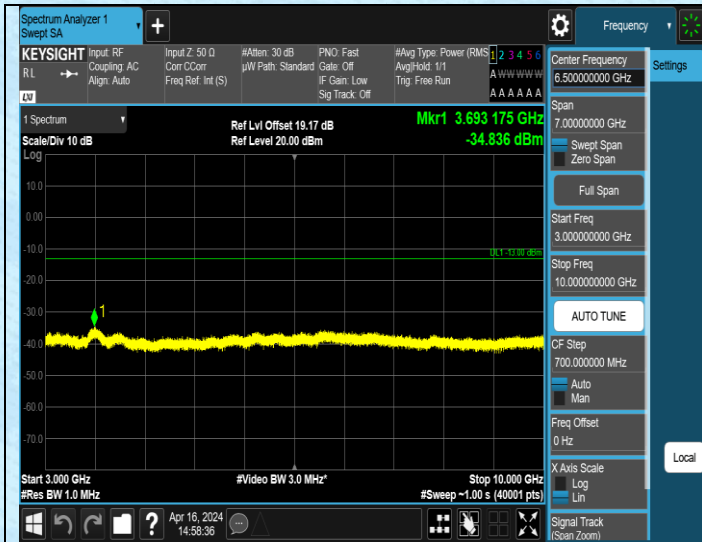
Band5_10MHz_QPSK_20525_1RB#0_3000~10000_3000~1000 0
