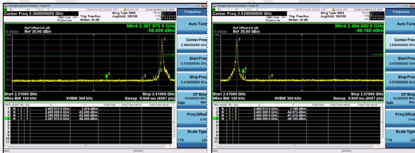
Left bandedge
