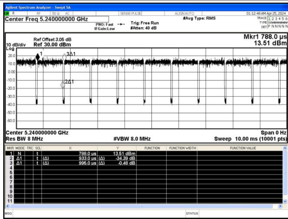
Duty Cycle NVNT n20 5240MHz Ant3
