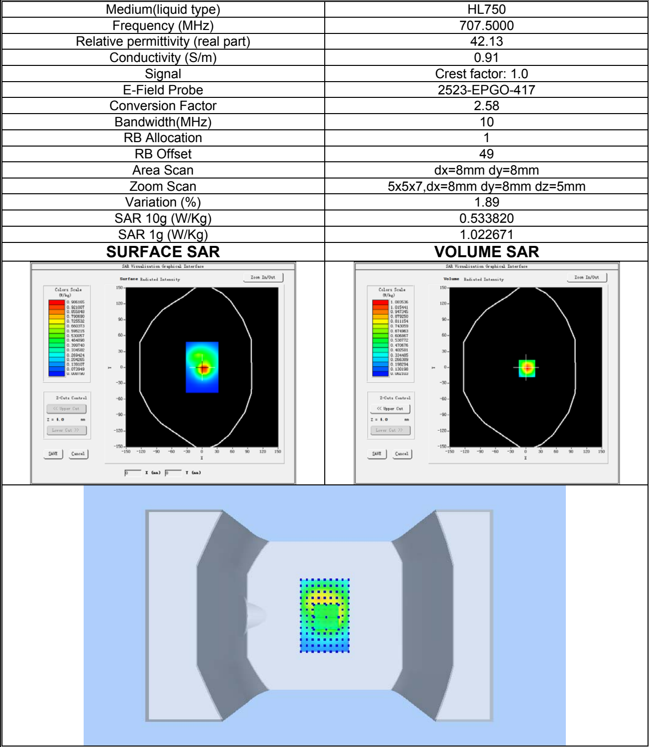
Plot 16: LTE BAND 12, Middle channel (Wrist-worn, Back Side) Product Description: Smart Watch Test Date: 2024-08-20
