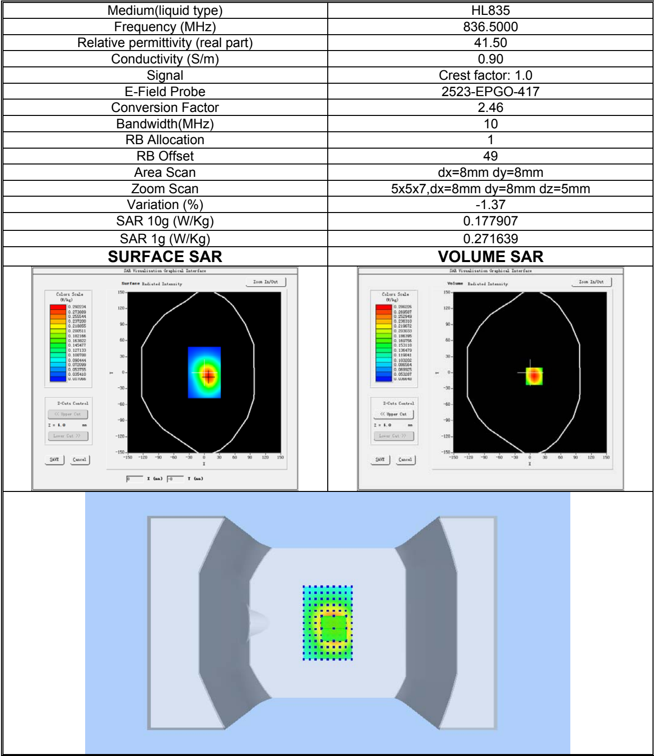
Plot 11:LTE BAND 5, Middle channel (Mouth, Front Side) Product Description: Smart Watch Test Date: 2024-08-20
