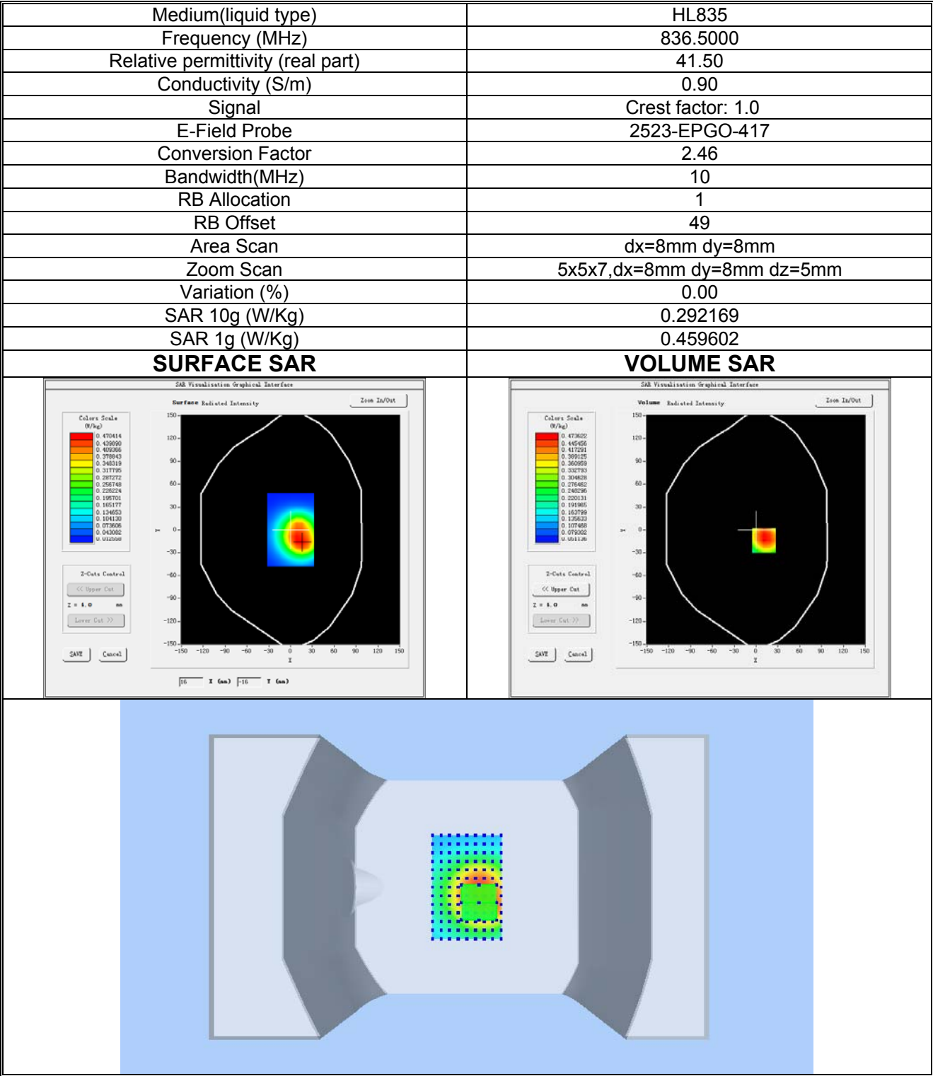
Plot 12: LTE BAND 5, Middle channel (Wrist-worn, Back Side) Product Description: Smart Watch Test Date: 2024-08-20
