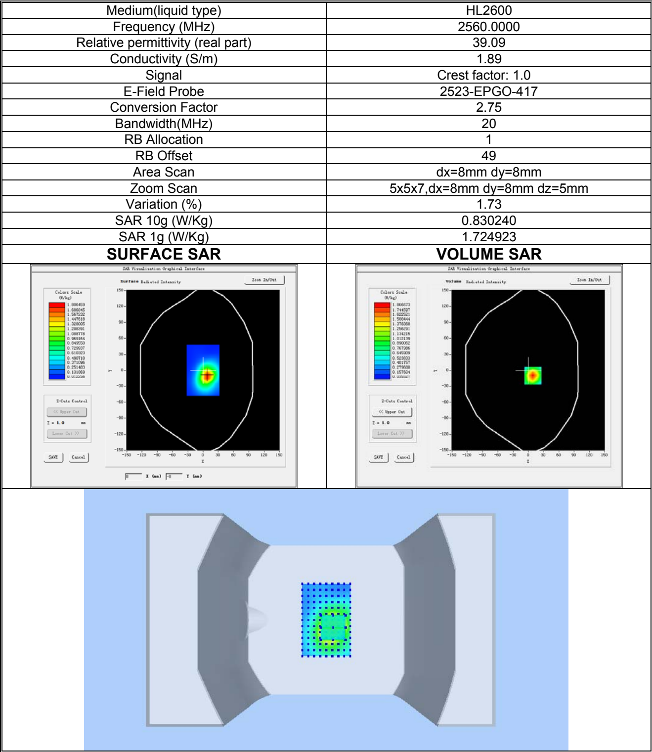
Plot 14: LTE BAND 7, High channel (Wrist-worn, Back Side) Product Description: Smart Watch Test Date: 2024-08-22
