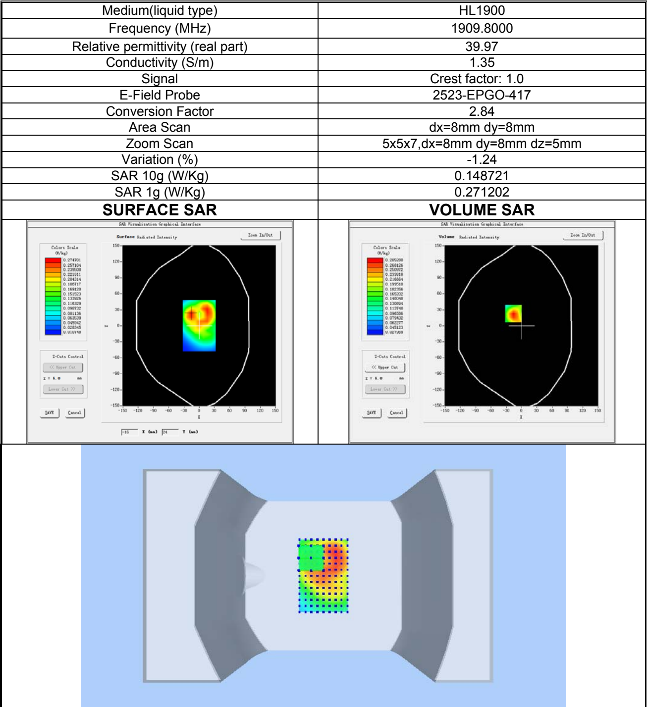
Plot 3: GPRS1900, High channel (Mouth, Front Side) Product Description: Smart Watch Test Date: 2024-08-19
