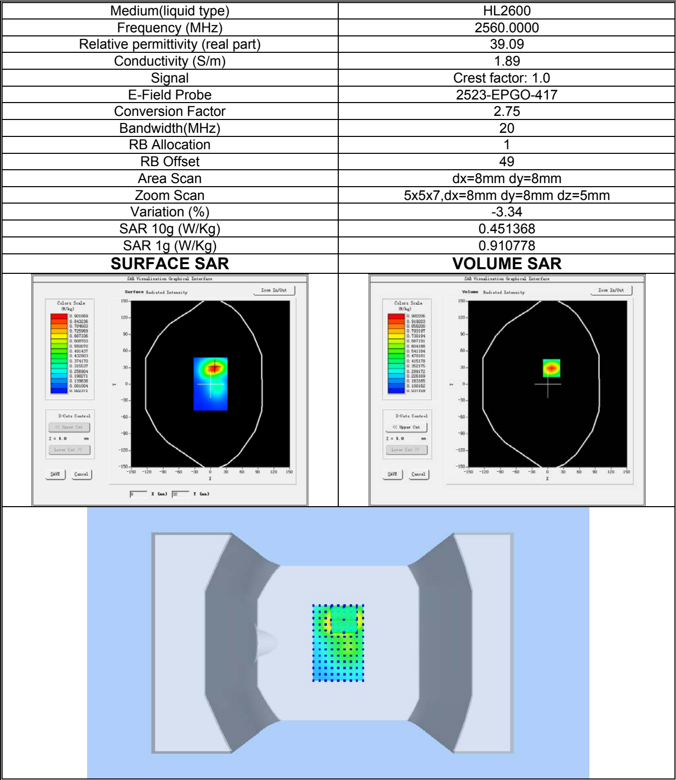
Plot 13:LTE BAND 7, High channel (Mouth, Front Side) Product Description: Smart Watch Test Date: 2024-08-22
