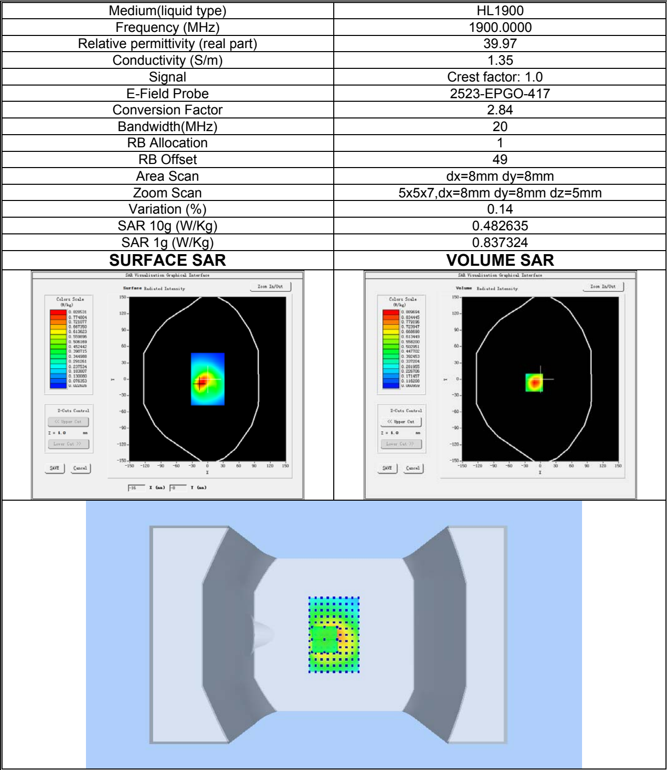
Plot 9:LTE BAND 2, High channel (Mouth, Front Side) Product Description:Smart Watch Test Date: 2024-08-19
