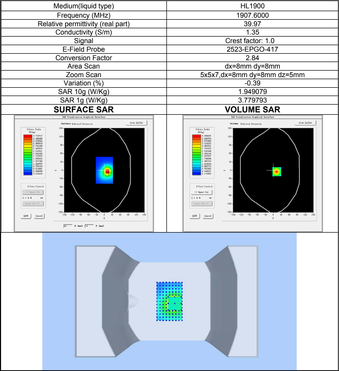
Plot 6: WCDMA BAND II, High channel (Wrist-worn, Back Side) Product Description: Smart Watch Test Date: 2024-08-19
