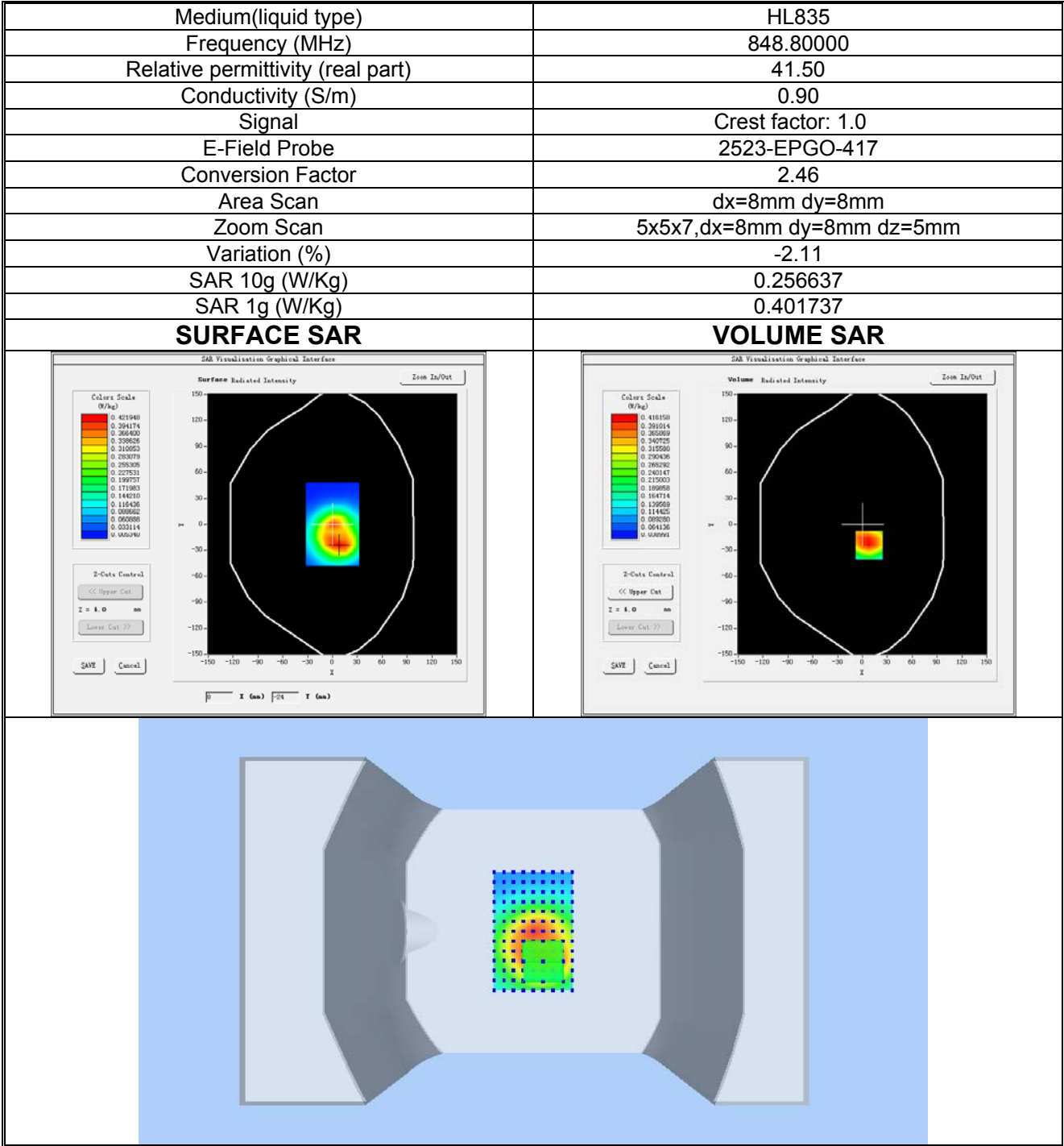
Plot 2: GPRS850MHz, High channel (Wrist-worn, Back Side) Product Description:Smart Watch Test Date: 2024-08-20
