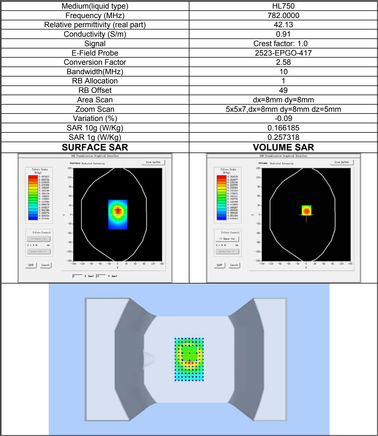
Plot 17:LTE BAND 13, Low channel (Mouth, Front Side) Product Description: Smart Watch Test Date: 2024-08-20
