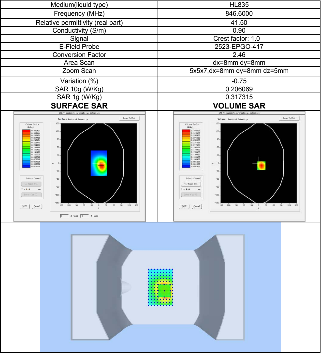
Plot 7: WCDMA BAND V, High channel (Mouth, Front Side) Product Description: Smart Watch Test Date: 2024-08-20
