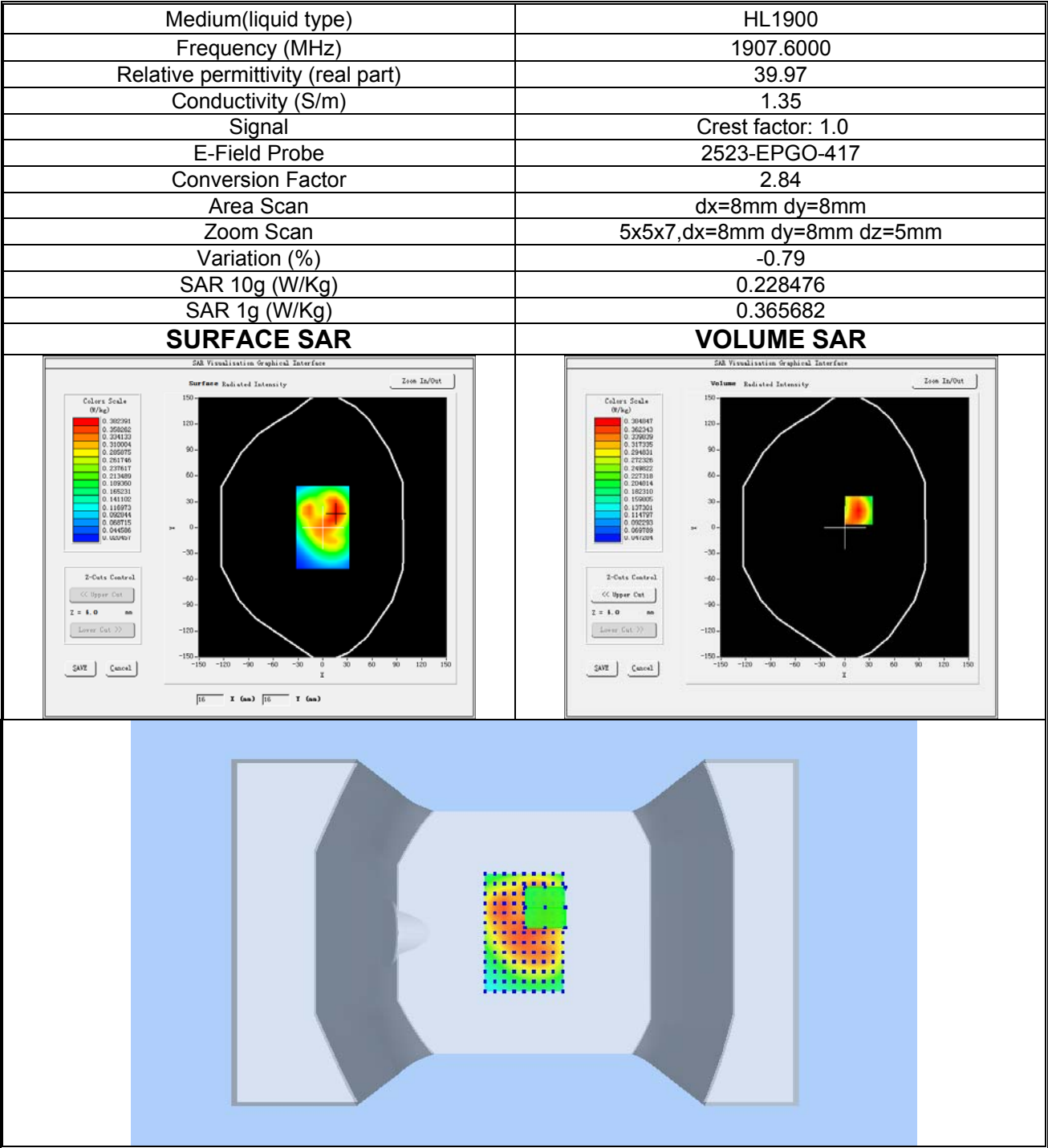
Plot 5: WCDMA BAND II, High channel (Mouth, Front Side) Product Description: Smart Watch Test Date: 2024-08-19
