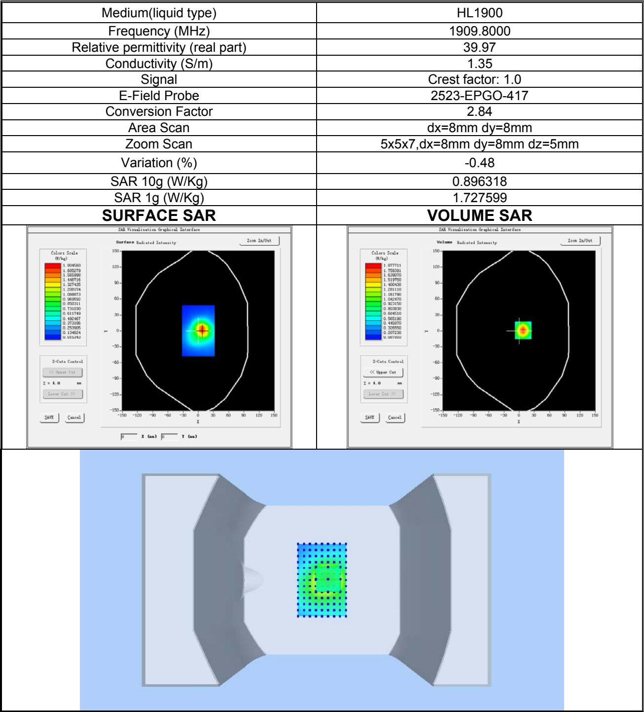
Plot 4: GPRS1900, High channel (Wrist-worn, Back Side) Product Description: Smart Watch Test Date: 2024-08-19
