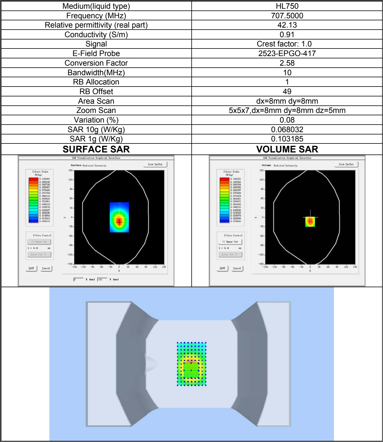
Plot 15:LTE BAND 12, Middle channel (Mouth, Front Side) Product Description: Smart Watch Test Date: 2024-08-20
