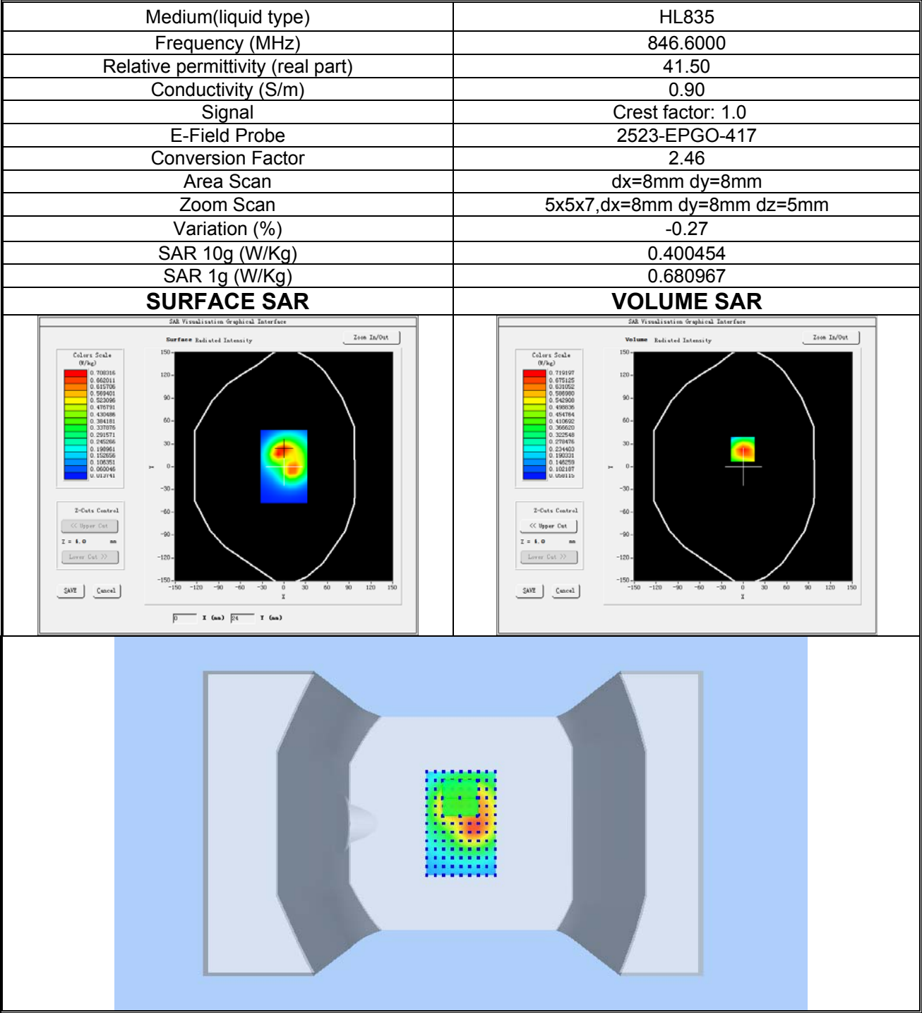
Plot 8: WCDMA BAND V, High channel (Wrist-worn, Back Side) Product Description: Smart Watch Test Date: 2024-08-20
