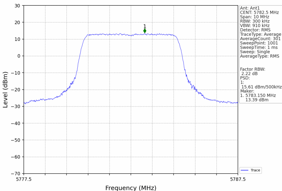
5M_MCH_5782.5MHz_Ant1_NTNV
