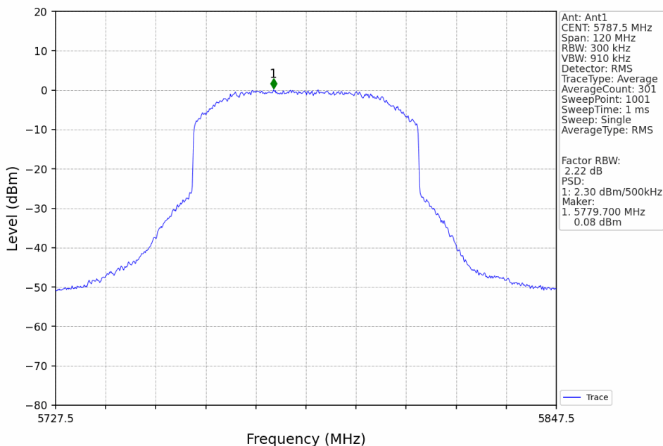
60M_MCH_5787.5MHz_Ant1_NTNV
