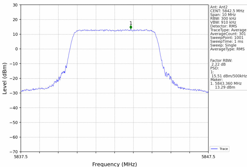
5M_HCH_5842.5MHz_Ant2_NTNV
