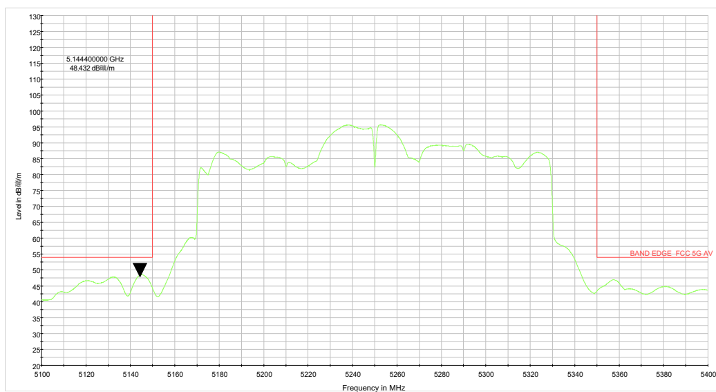
be160 CH50_5.1-5.4GHz_TP14_0320_AV.wmf
