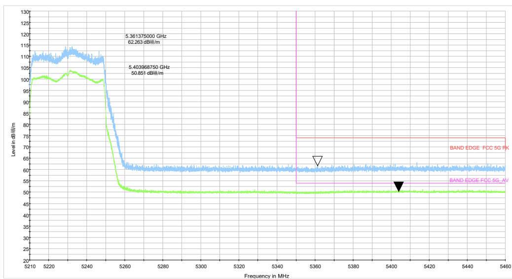
be40 CH46_5.21-5.46GHz_TP14
