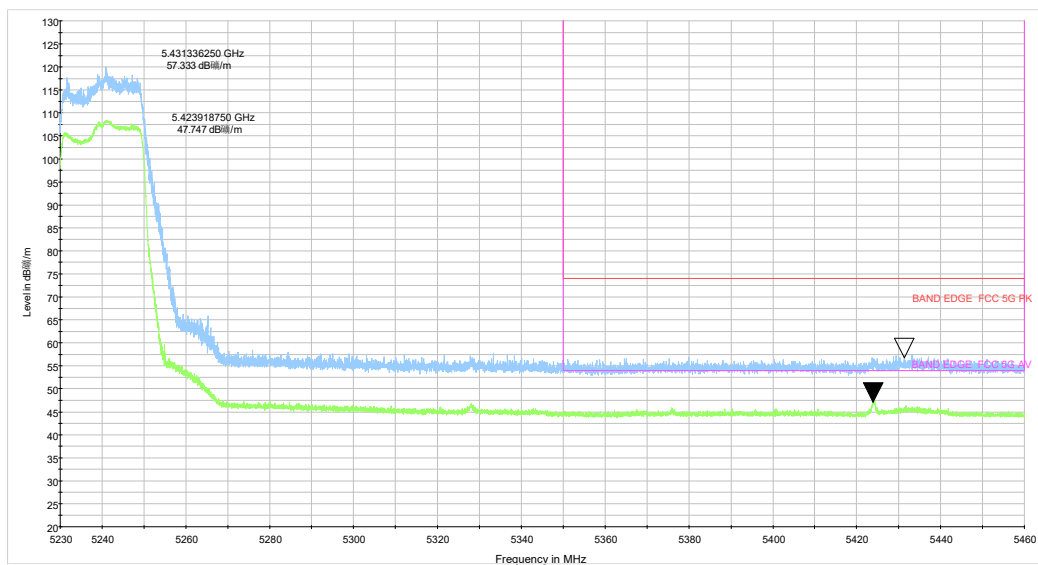
ax20 CH48_5.23-5.46GHz_TP15
