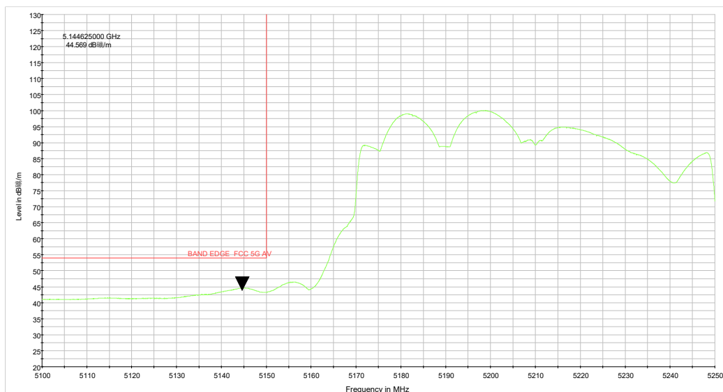
ax80 CH42_5.1-5.25GHz_TP15_0321_AV.wmf
