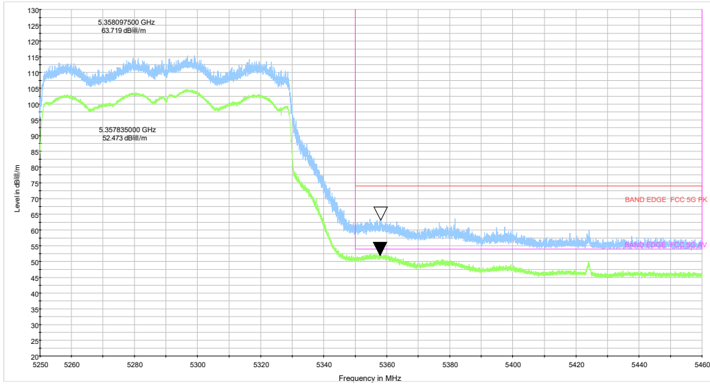
ax80 CH58_5.25-5.46GHz_TP15
