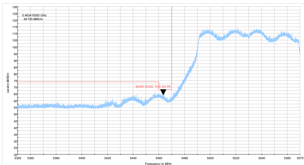
ax80 CH106_5.35-5.57GHz_TP15_0321_PK.wmf
