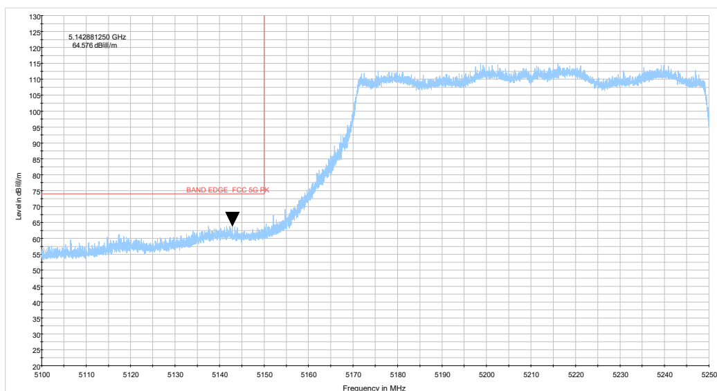
ax80 CH42_5.1-5.25GHz_TP15_0321_PK.wmf
