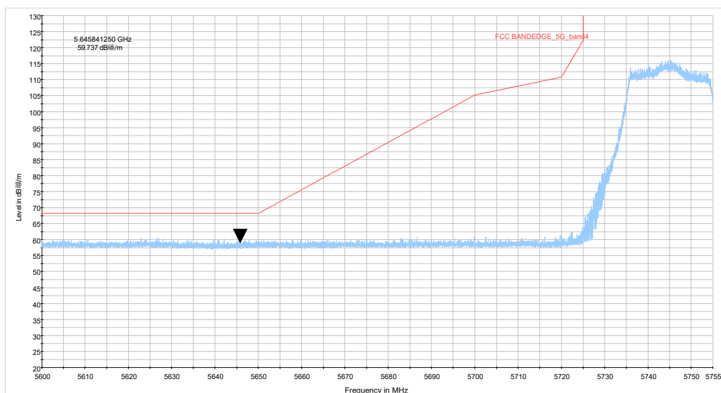
be20 CH149_5.6-5.755GHz_TP14
