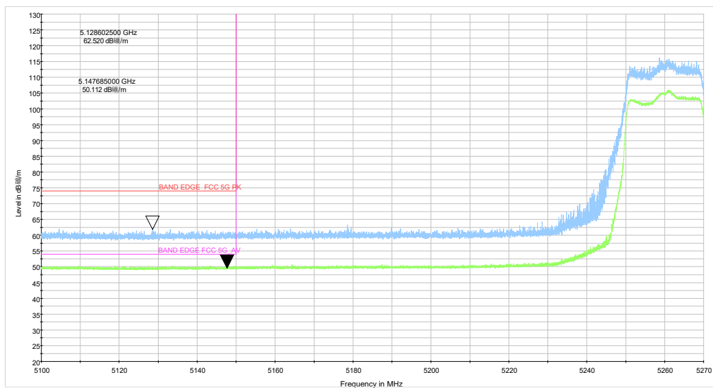
be20 CH52_5.1-5.27GHz_TP14
