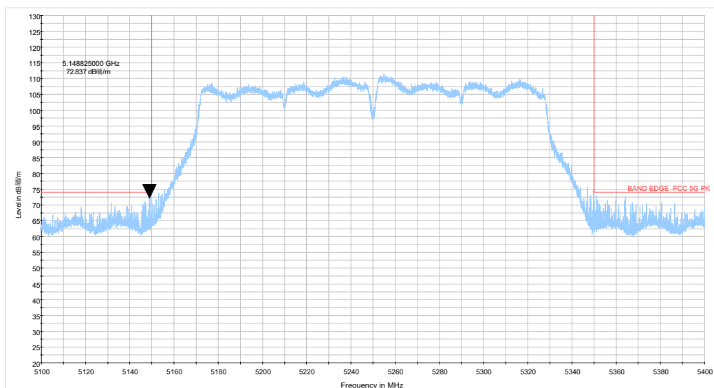
ac160 CH50_5.1-5.4GHz_TP16_0320_PK.wmf
