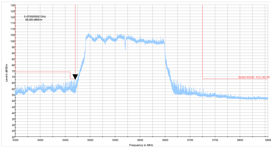
be160 CH114_5.35-5.856GHz_TP12_0320_PK.wmf
