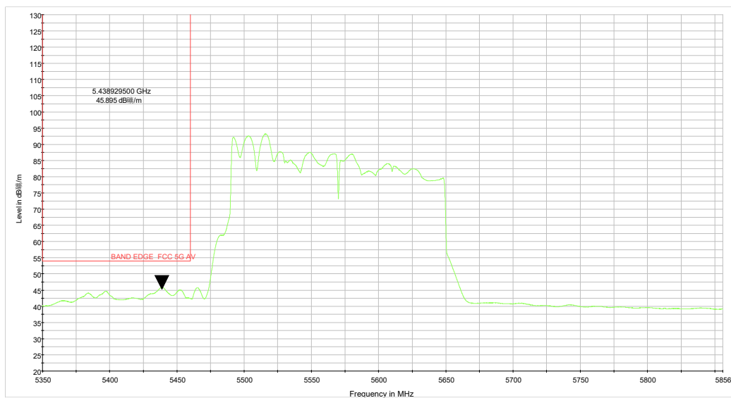
be160 CH114_5.35-5.856GHz_TP13_0320_AV.wmf
