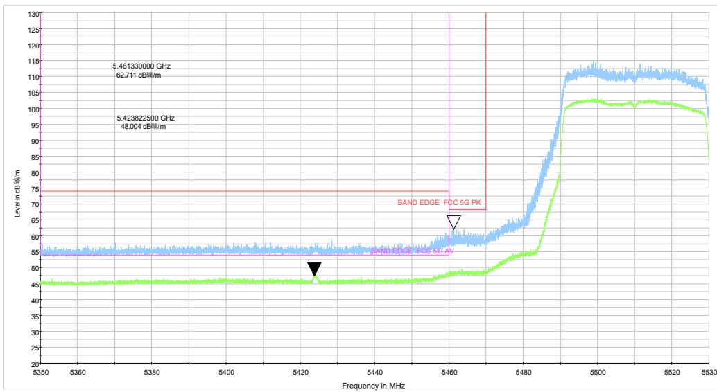
ax40 CH102_5.35-5.53GHz_TP15
