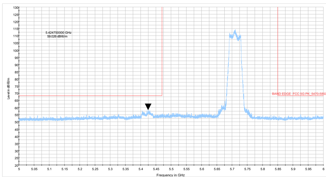
be40 CH142_5-6GHz_TP14
