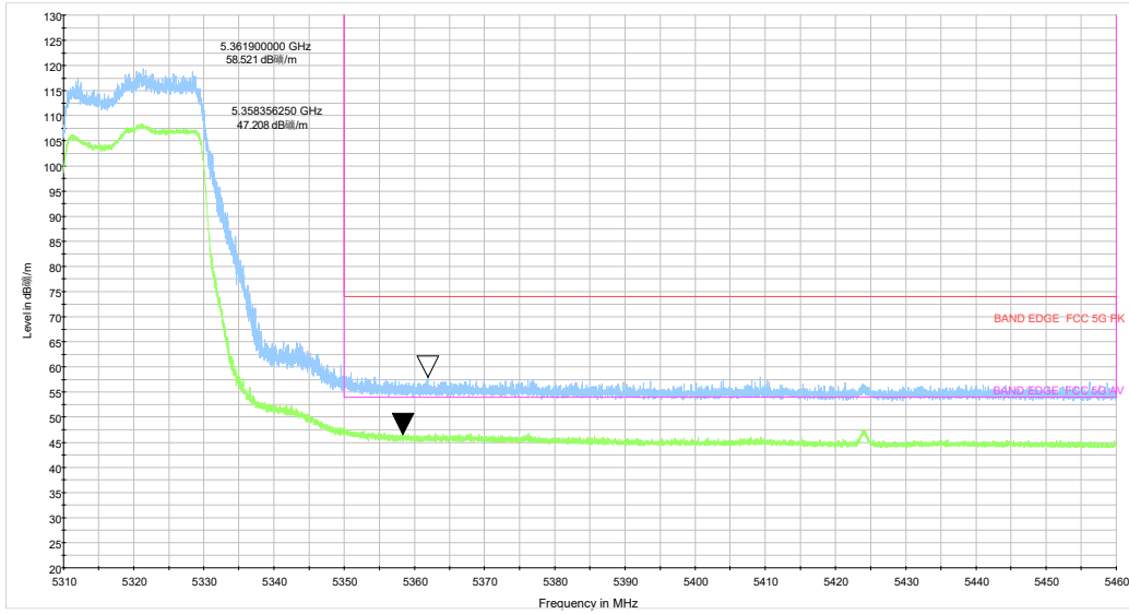
ax20 CH64_5.31-5.46GHz_TP15
