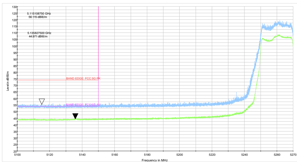
ax20 CH52_5.1-5.27GHz_TP15
