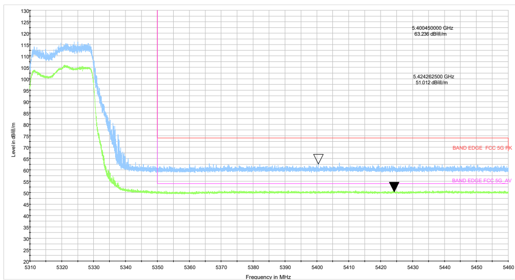
be20 CH64_5.31-5.46GHz_TP14
