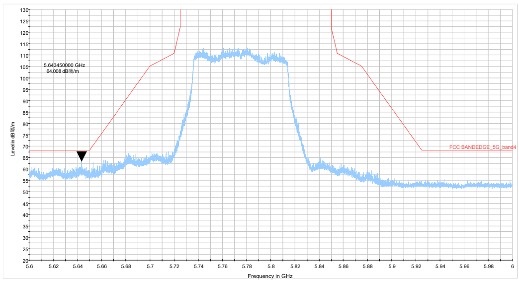
ax80 CH155_5.6-.6GHz_TP15
