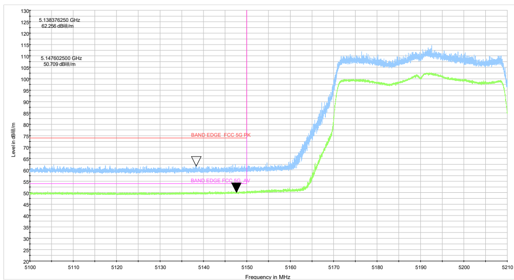
be40 CH38_5.1-5.21GHz_TP14
