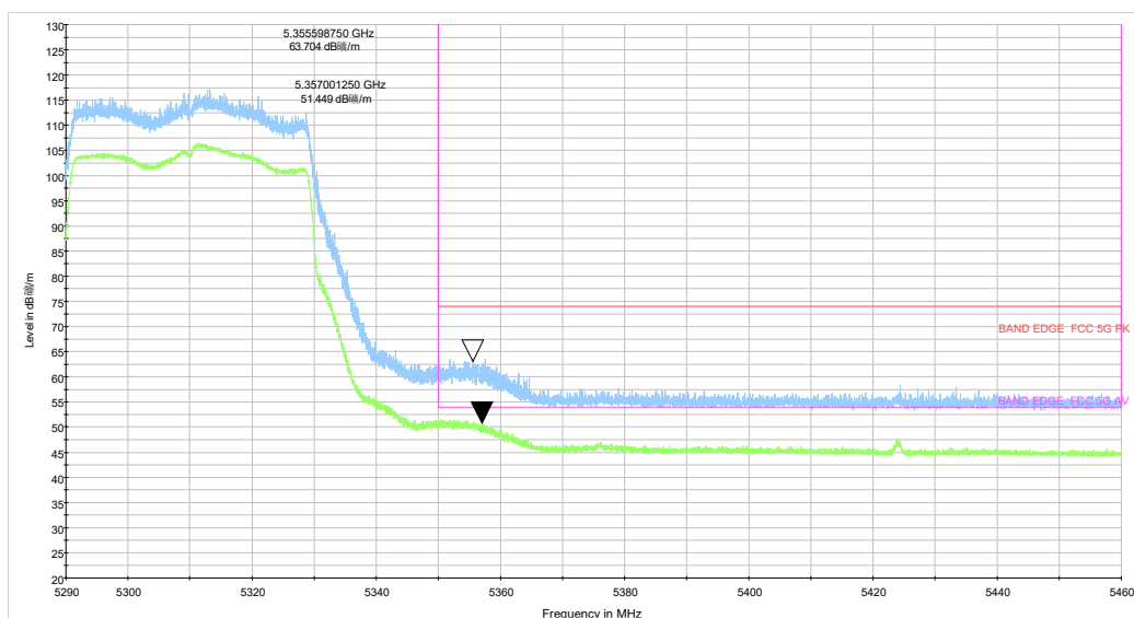
ax40 CH62_5.29-5.46GHz_TP15
