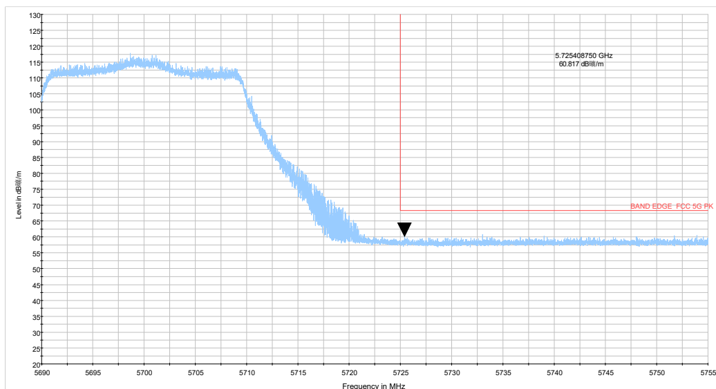
be20 CH140_5.69-5.755GHz_TP14
