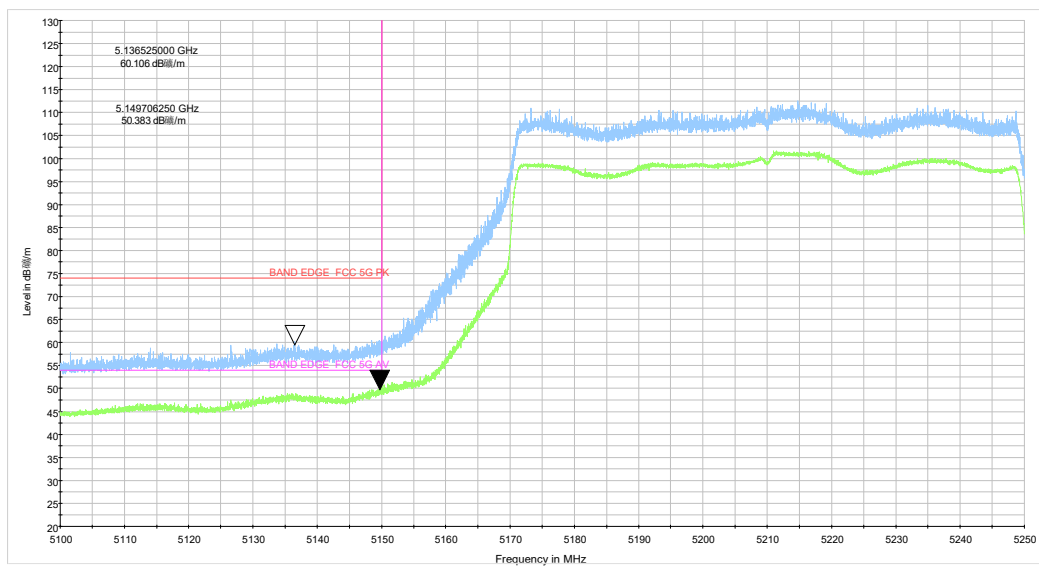
be80 CH42_5.1-5.25GHz_TP14
