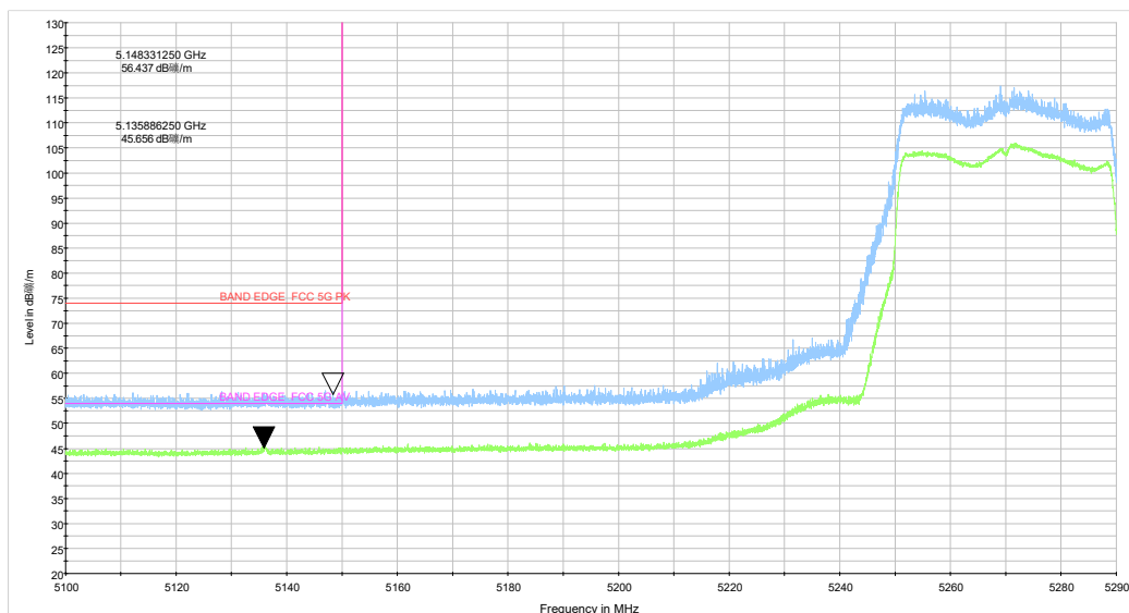
ax40 CH54_5.1-5.29GHz_TP15
