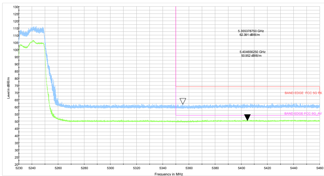
be20 CH48_5.23-5.46GHz_TP14
