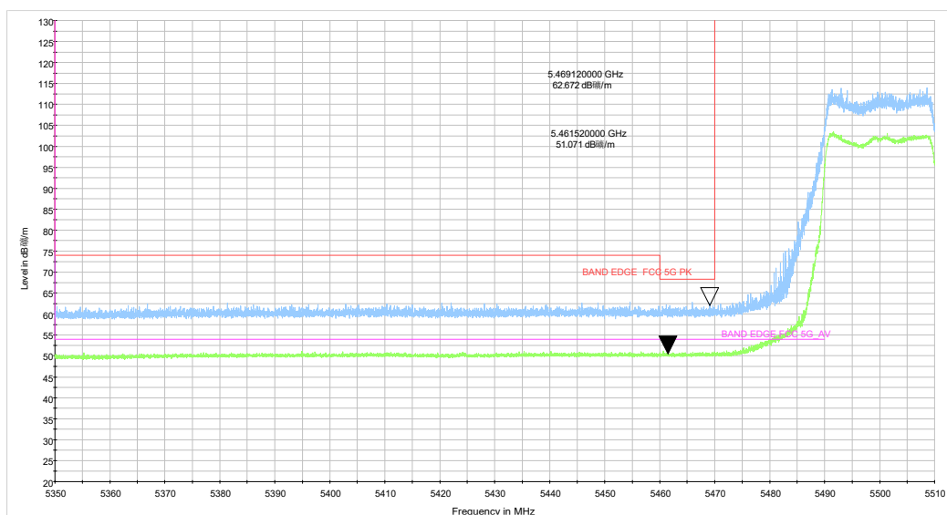
be20 CH100_5.35-5.51GHz_TP14
