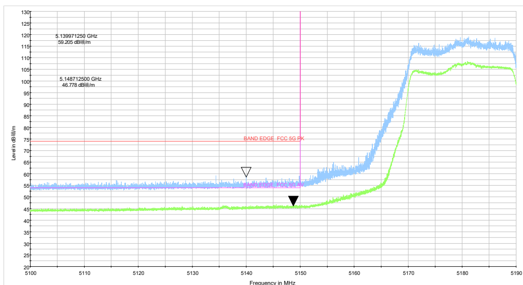
ax20 CH36_5.1-5.19GHz_TP15
