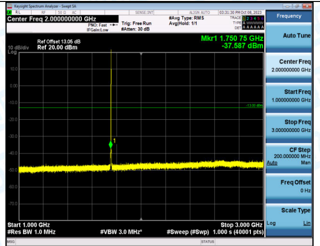
Band4_1.4MHz_QPSK_20393_1RB#0_1000~3000_1000~3000
