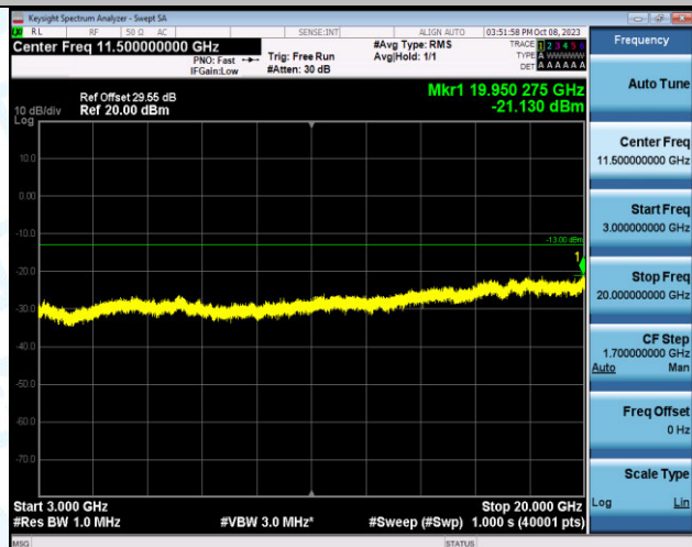
Band4_3MHz_QPSK_19965_1RB#0_3000~20000_3000~20000
