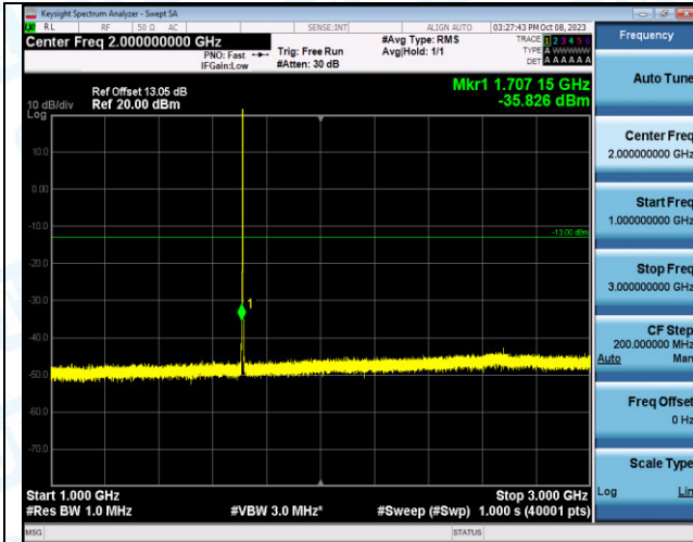
Band4_1.4MHz_16QAM_19957_6RB#0_1000~3000_1000 ~3000
