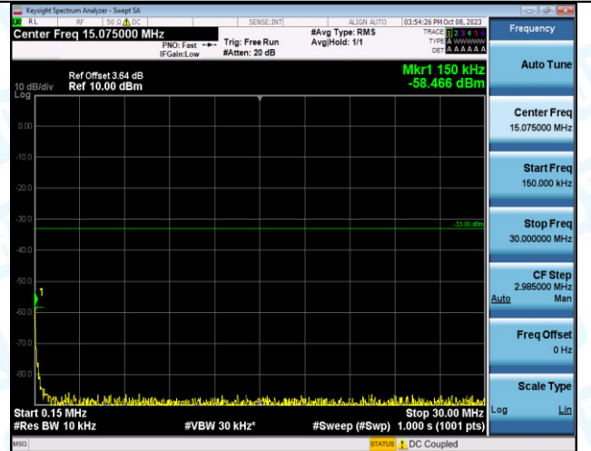
Band4_3MHz_QPSK_20175_1RB#0_0.15~30_0.15~30
