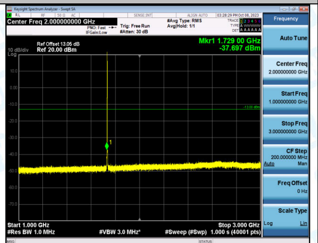
Band4_1.4MHz_QPSK_20175_1RB#0_1000~3000_1000~3000 3000
