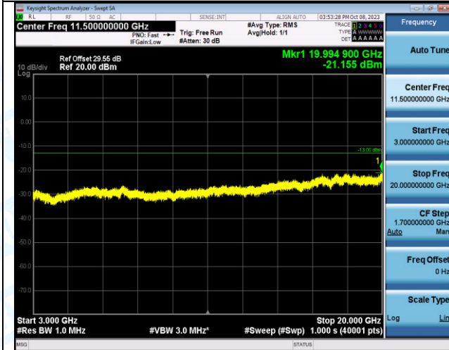
Band4_3MHz_QPSK_19965_15RB#0_3000~20000_3000~20000
