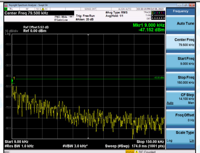
Band4_1.4MHz_16QAM_20175_6RB#0_0.009~0.15_0.00 9~0.15
