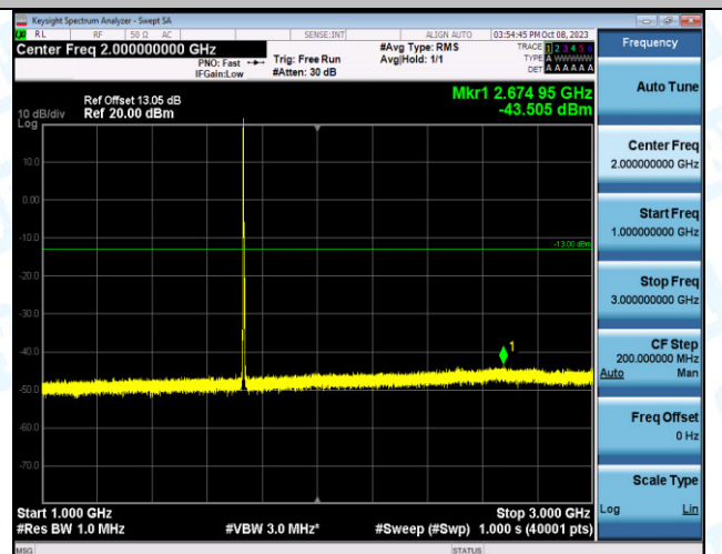
Band4_3MHz_QPSK_20175_1RB#0_1000~3000_1000~3000
