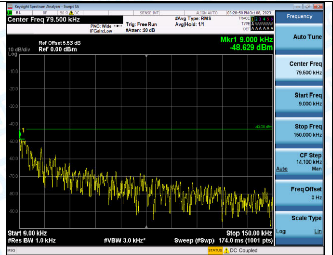
Band4_1.4MHz_16QAM_20175_1RB#0_0.009~0.15_0.00 9~0.15
