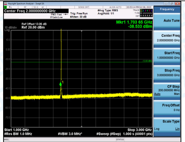
Band4_3MHz_QPSK_19965_15RB#0_1000~3000_1000~3000
