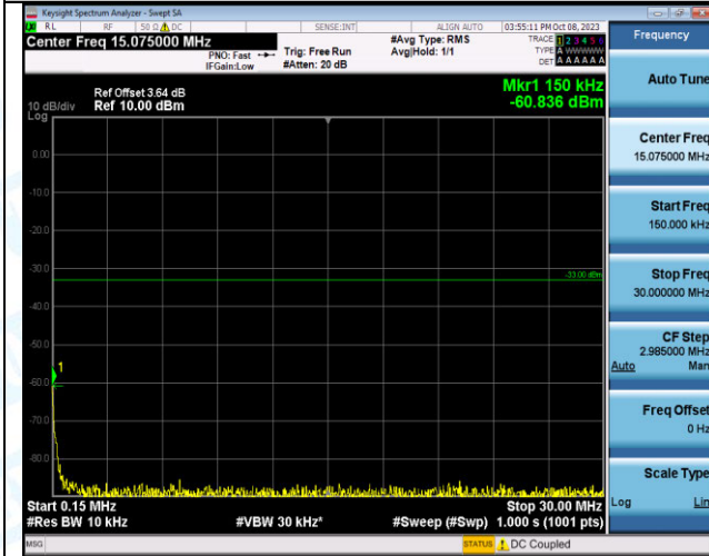
Band4_3MHz_16QAM_20175_1RB#0_0.15~30_0.15~30
