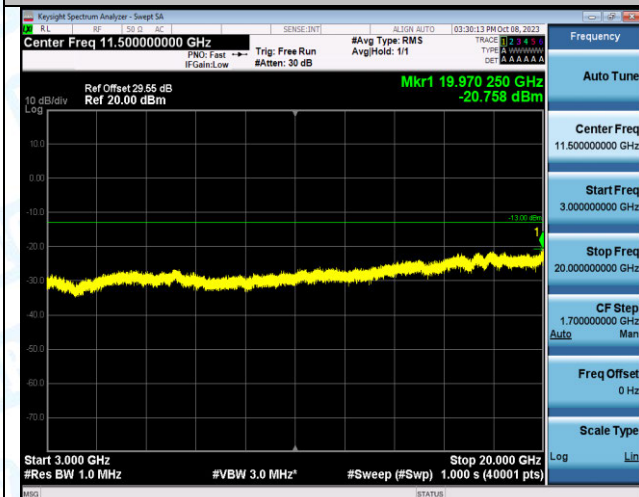
Band4_1.4MHz_QPSK_20175_6RB#0_3000~20000_3000 ~20000
