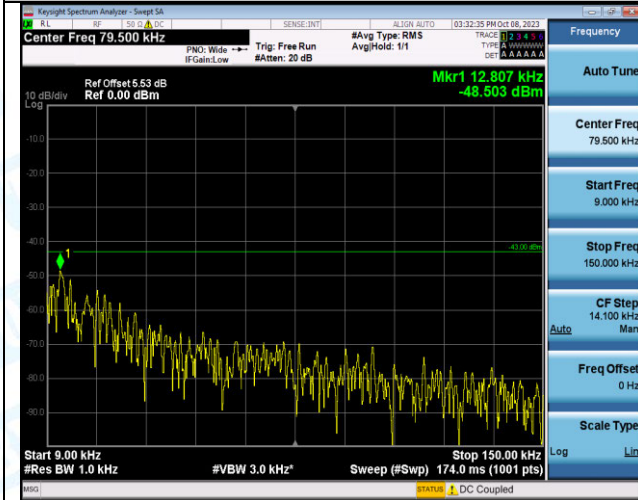
Band4_1.4MHz_QPSK_20393_6RB#0_0.009~0.15_0.009 ~0.15
