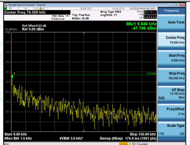
Band4_3MHz_16QAM_19965_1RB#0_0.009~0.15_0.009~0.15
