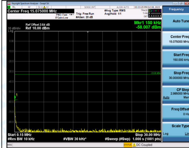
Band4_1.4MHz_16QAM_20393_6RB#0_0.15~30_0.15~3 0
