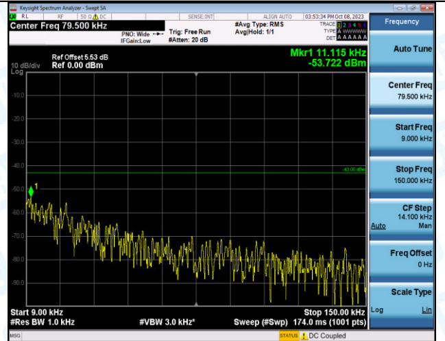
Band4_3MHz_16QAM_19965_15RB#0_0.009~0.15_0.009~0.15
