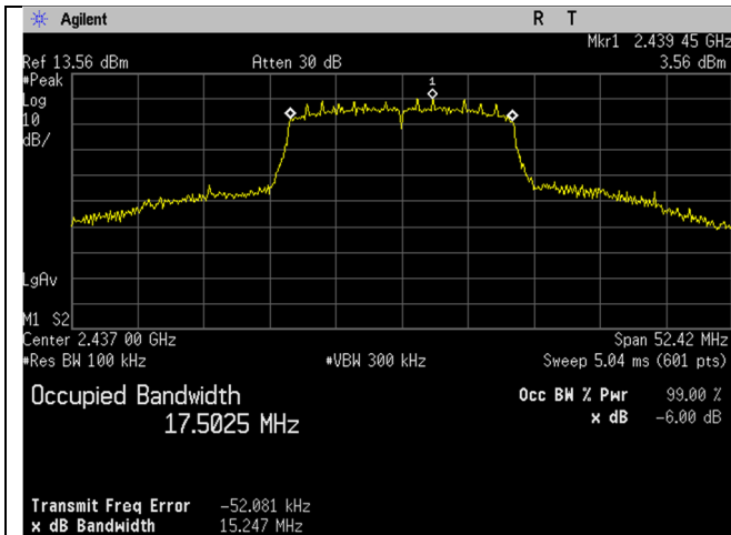
WIFI_Mid Ch_2437MHz_20MHz BW_n-mode_Occupied Bandwidth_-6dB
