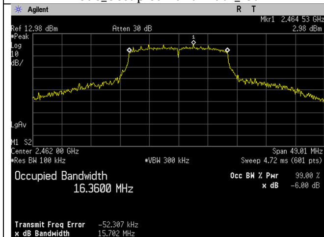
WIFI_High Ch_2462MHz_20MHz BW_g-mode_Occupied Bandwidth_-6dB
