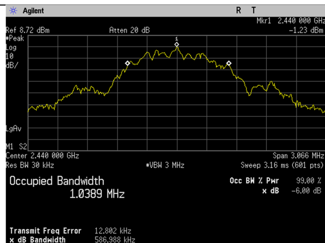
BLE_Mid Ch_2440MHz_1MBit_Occupied Bandwidth_99 percent
