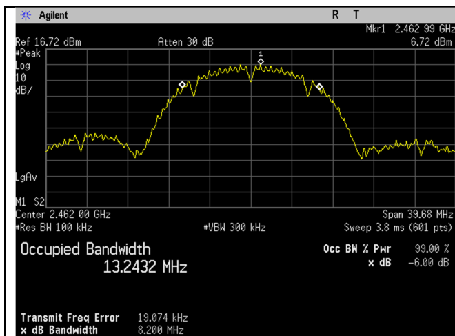
WIFI_High Ch_2462MHz_20MHz BW_b-mode_Occupied Bandwidth_-6dB
