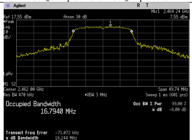
WIFI_High Ch_2462MHz_20MHz BW_g-mode_Occupied Bandwidth_99 percent
