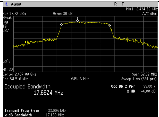
WIFI_Mid Ch_2437MHz_20MHz BW_n-mode_Occupied Bandwidth_99 percent
