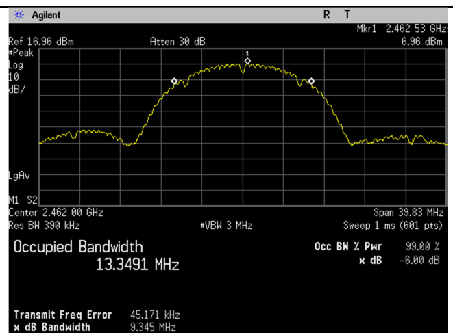
WIFI_High Ch_2462MHz_20MHz BW_b-mode_Occupied Bandwidth_99 percent
