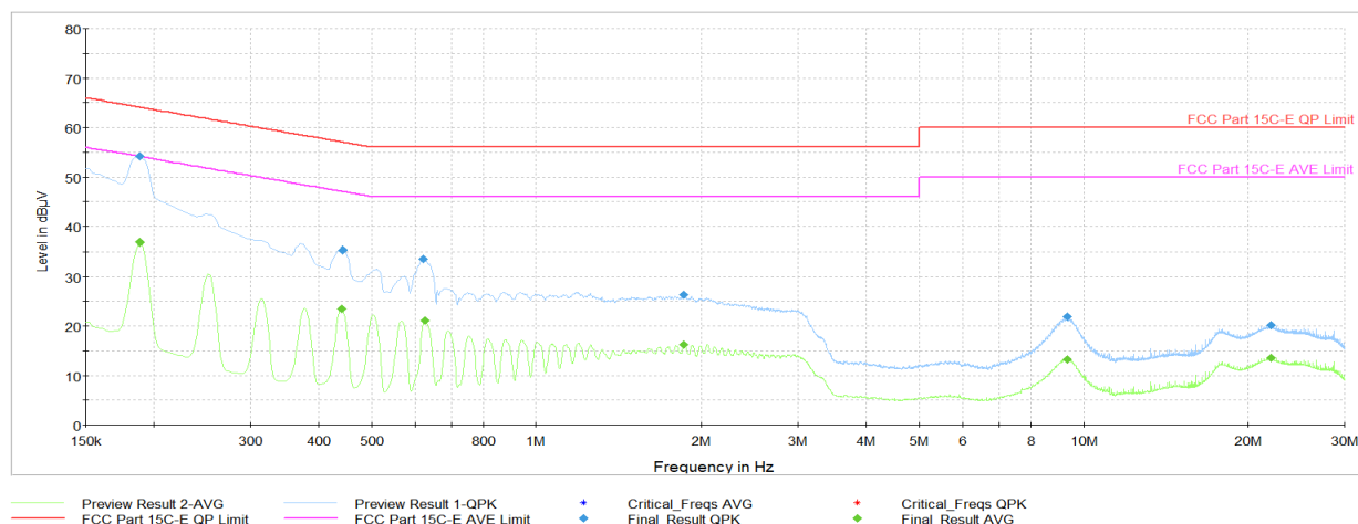
Plot 7-33. AC Line Conducted Plot with Bluetooth LE (N, 1Mbps – Ch.0 with charging case AC/DC Adapter)
