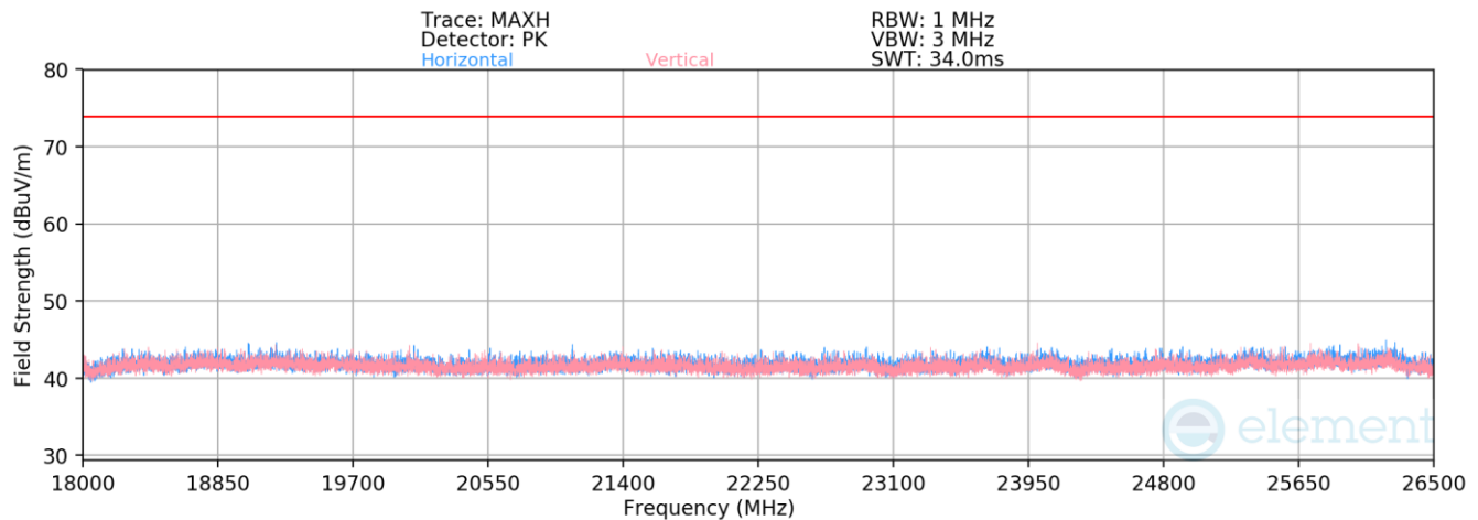
Plot 7-24. Radiated Spurious Emissions Above 18GHz (1Mbps – Ch. 0)
