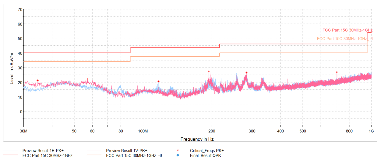
Plot 7-31. Radiated Spurious Emissions Below 1GHz (1Mbps – Ch.0, Pol. H & V, with charging case and AC/DC Adapter)
