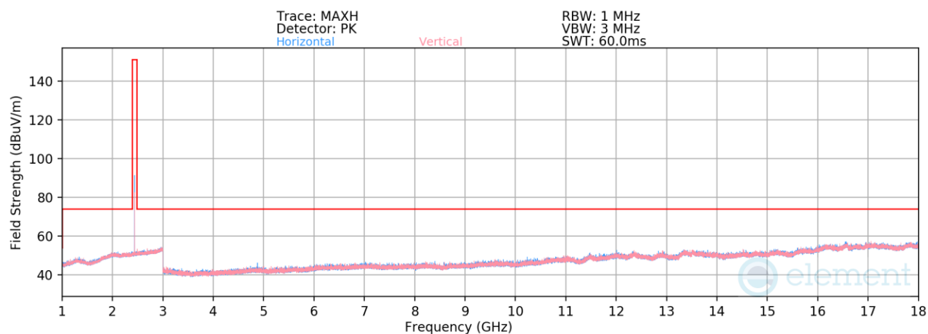
Plot 7-25. Radiated Spurious Emissions 1-18GHz (1Mbps – Ch. 19)
