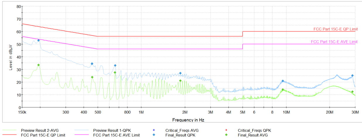
Plot 7-32. AC Line Conducted Plot with Bluetooth LE (L1, 1Mbps – Ch.0 with charging case AC/DC Adapter)
