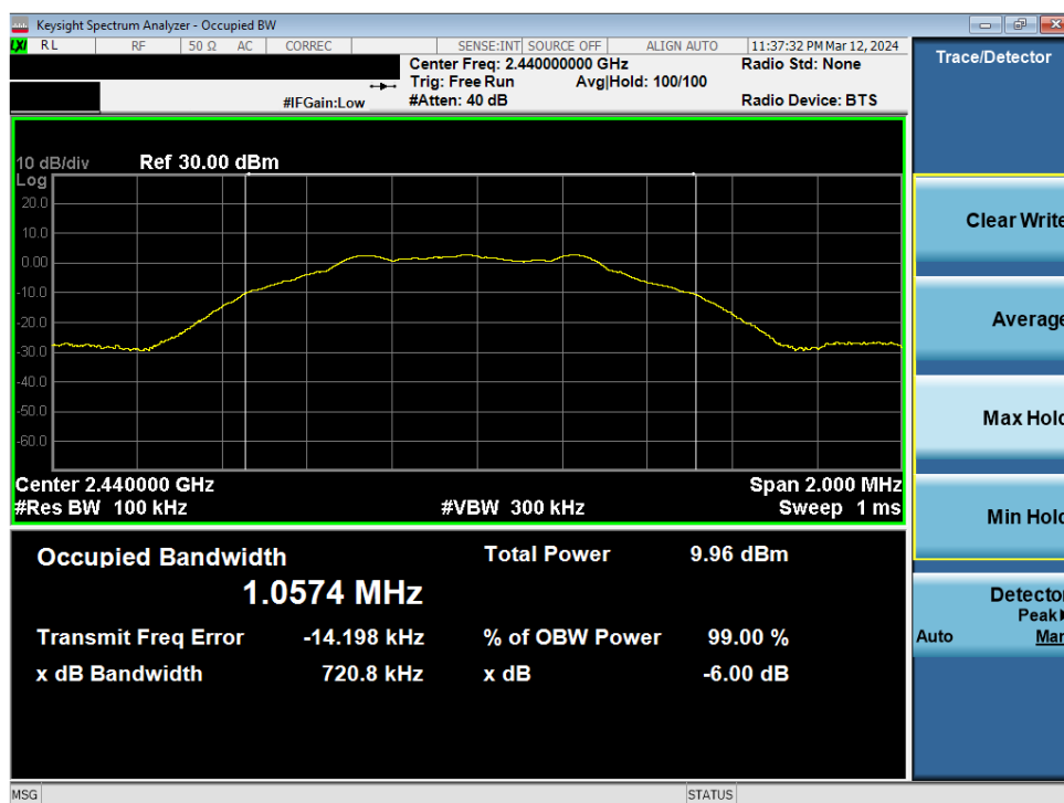
Plot 7-2. 6dB BW & 99% OBW Plot (Bluetooth (LE), 1Mbps – Ch. 19)
