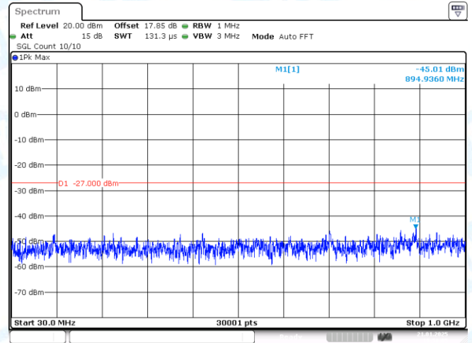
11AX40-CDD-Ant2-5710-30~1000-PASS
