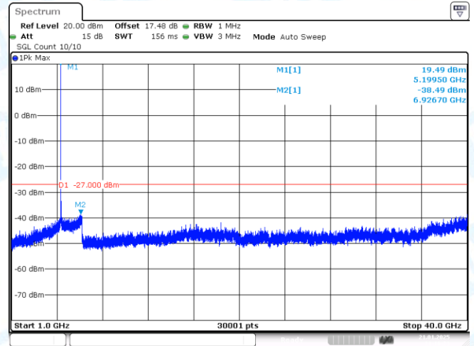
11AX20-CDD-Ant2-5200-1000~40000-PASS
