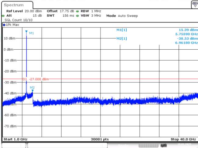
11AX40-CDD-Ant1-5755-1000~40000-PASS
