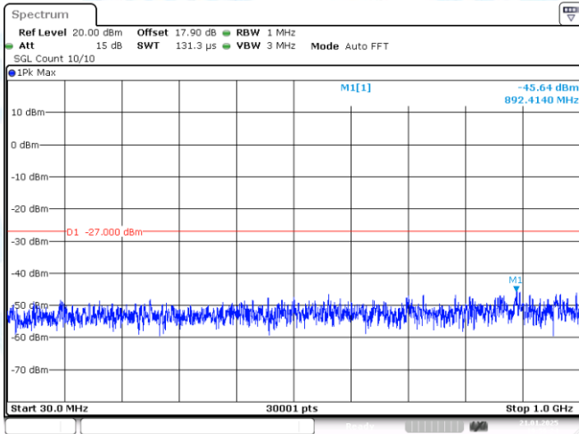
11AX40-CDD-Ant1-5710-30~1000-PASS
