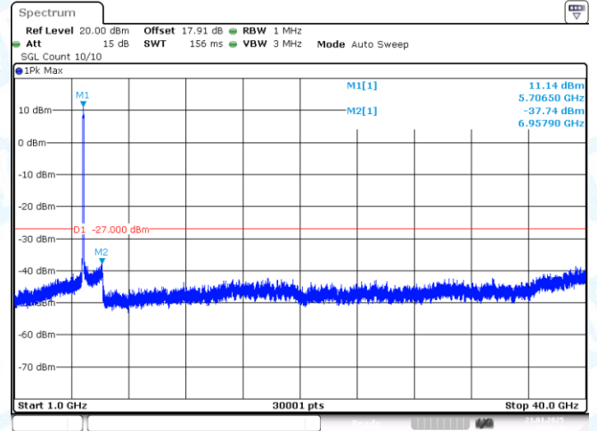
11AX80-CDD-Ant2-5690-1000~40000-PASS
