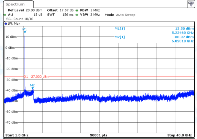
11AX40-CDD-Ant2-5230-1000~40000-PASS
