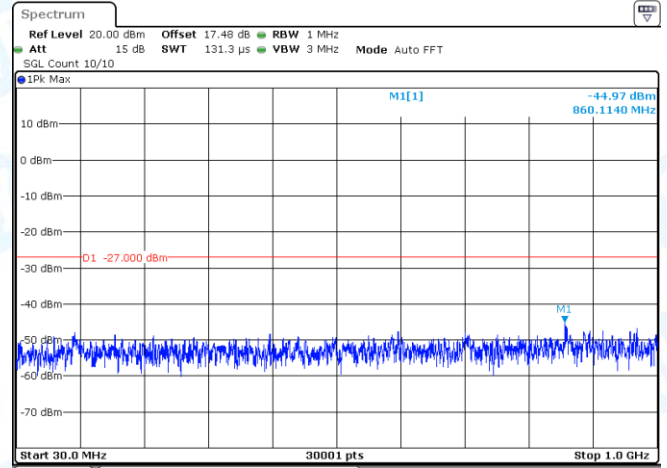
11AX40-CDD-Ant2-5190-30~1000-PASS
