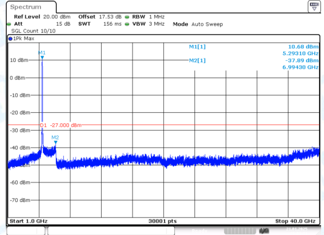
11AX80-CDD-Ant2-5290-1000~40000-PASS
