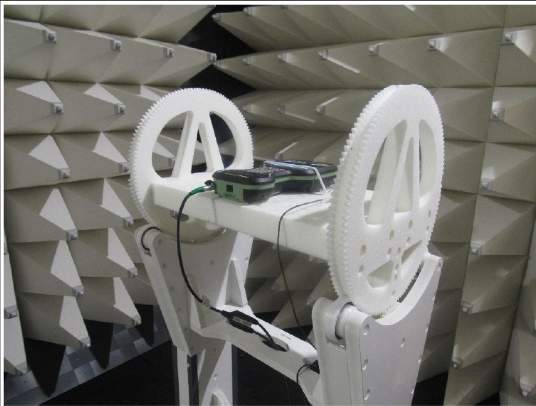
Testseup above 1 GHz
