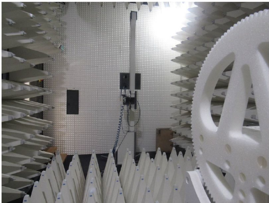
Testseup above 1 GHz
